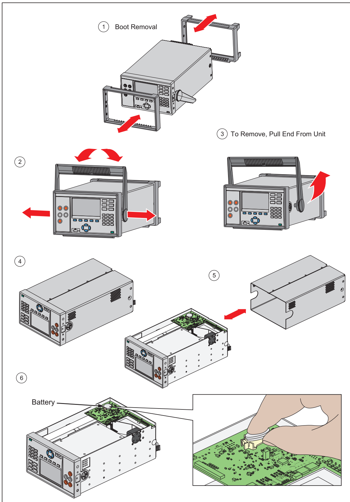
Figure 10. Disassembly
