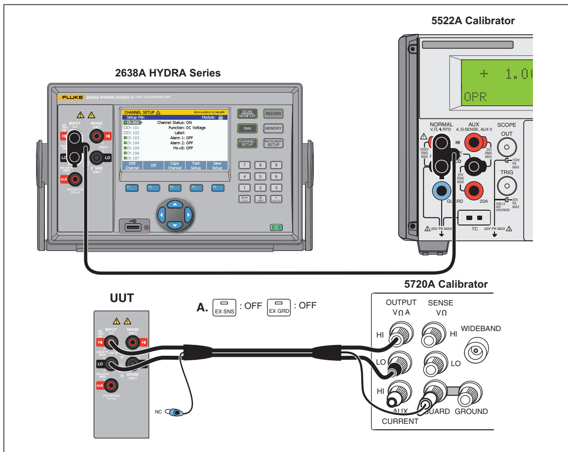
Figure 3. AC Volts Verification Connections
