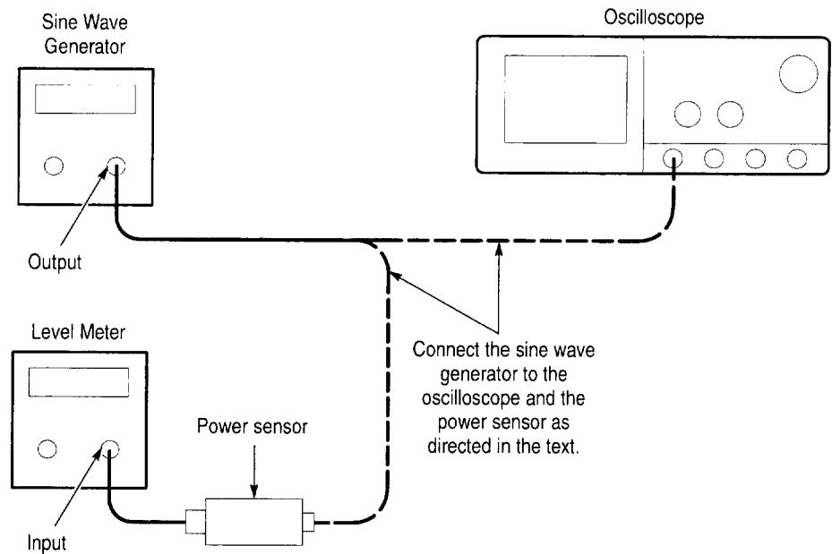
Figure 1-42: Equipment setup for maximum amplitude
