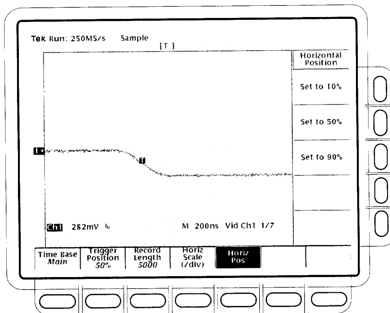
Figure 1-36: Line count accuracy test setup waveform – TDS 684C shown
