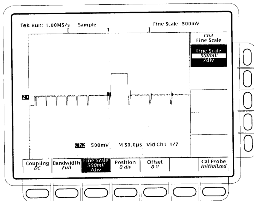
Figure 1-34: 60 Hz Rejection test result – TDS 684C shown
