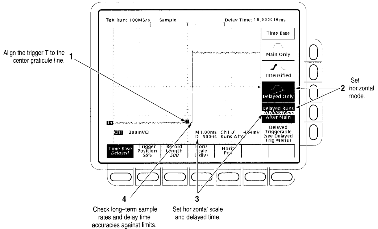
Figure 1-13: Measurement of accuracy – Long-term and delay time
