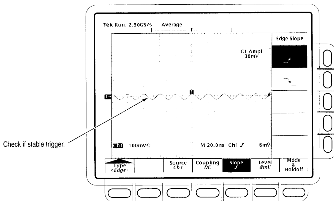
Figure 1-19: Measurement of trigger sensitivity – 50 MHz results shown on a TDS 684C screen
