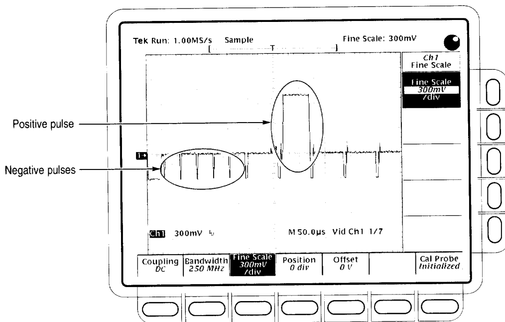
Figure 1–29: Triggered signal range test – 300 mV
