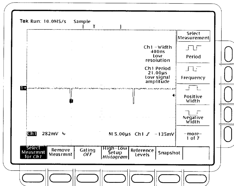
Figure 1-40: Sync duty cycle test: critically adjusted pulse
