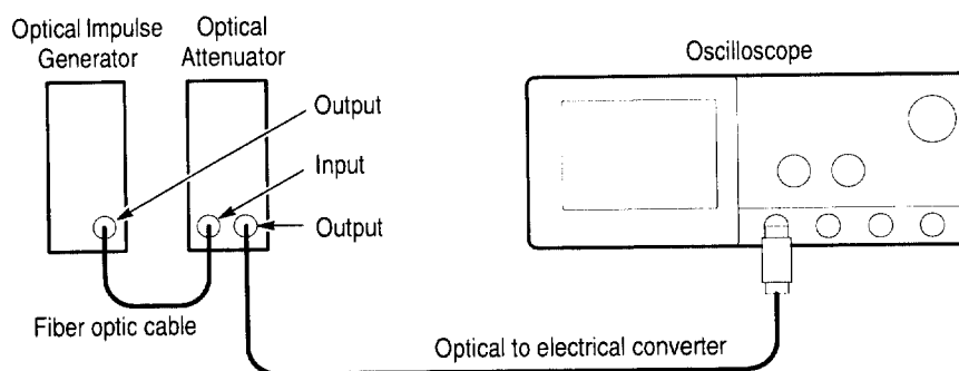
Figure 1–43: Reference-receiver performance-verification set up
