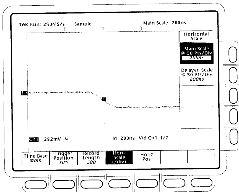
Figure 1-27: Jitter test displayed waveform – TDS 684C shown
