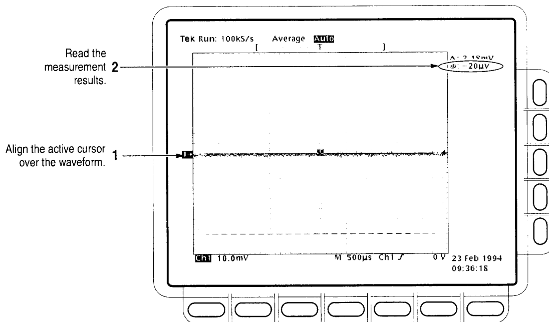
Figure 1–4: Measurement of DC offset accuracy at zero setting – TDS 684C shown
