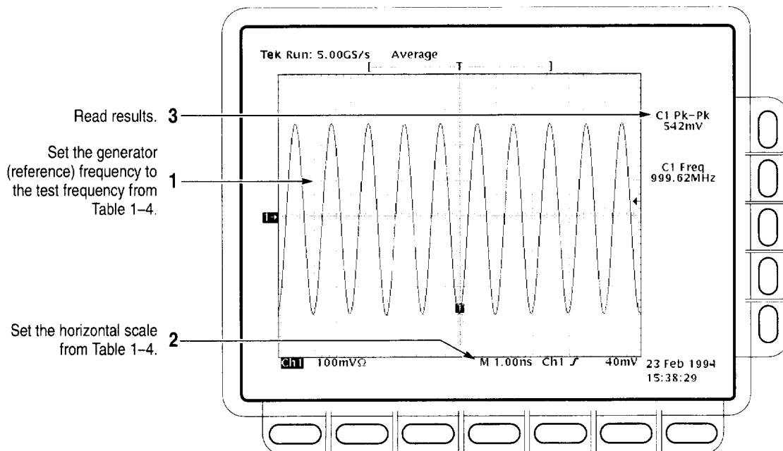
Figure 1–9: Measurement of analog bandwidth
