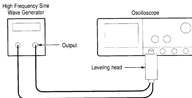
Figure 1–8: Optional initial test hookup
