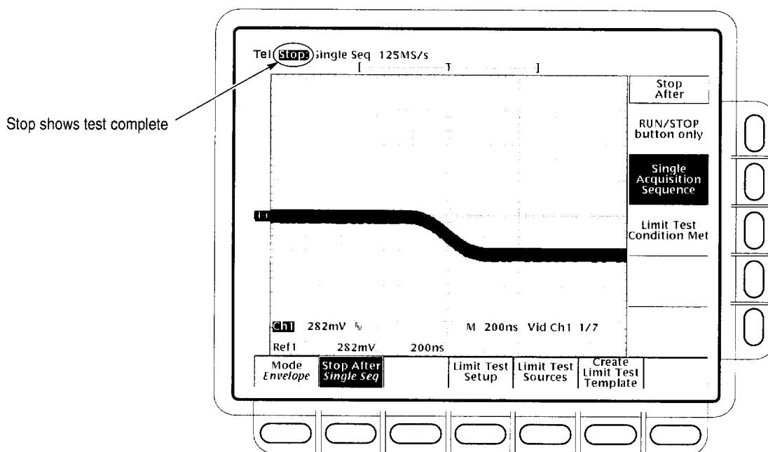
Figure 1–28: Jitter test when completed – TDS 684C shown
