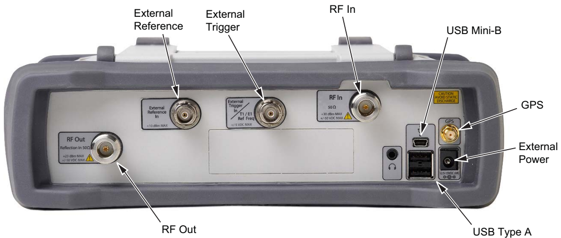
Figure 2-7. S332E Test Panel Connector
