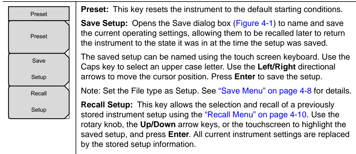
Figure 5-5. Preset Menu
