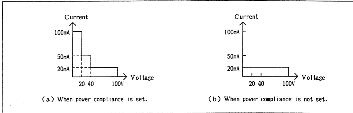
Allowable I Output when the MPSMU sweeps voltages from 0 V to 100 V
