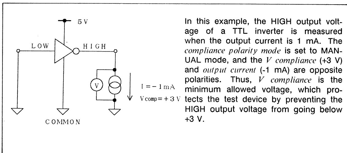
Compliance Polarity MANUAL Mode V Measurement Example
