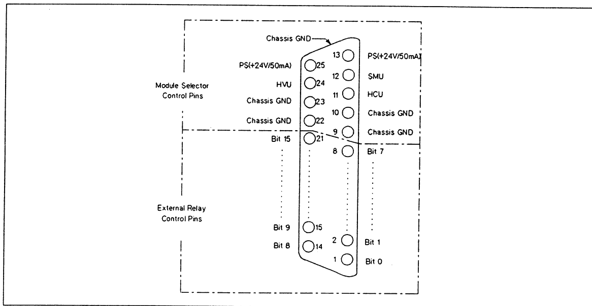
Pin Assignment of the CONTROL Connector
