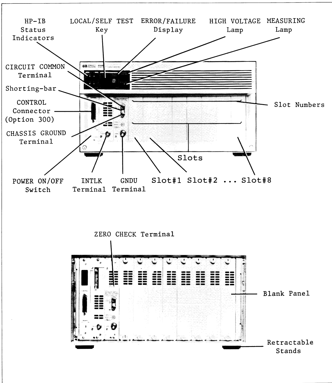
HP 4142B Panel Overview (1 of 2)
