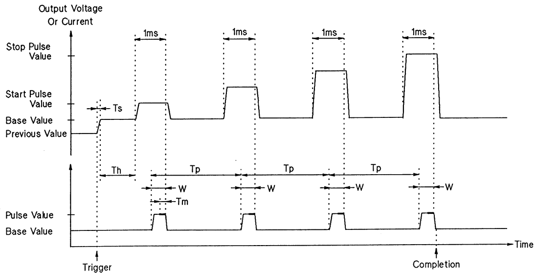
Pulsed Sweep with Pulsed Bias Measurement Output Waveform (1 of 2)
