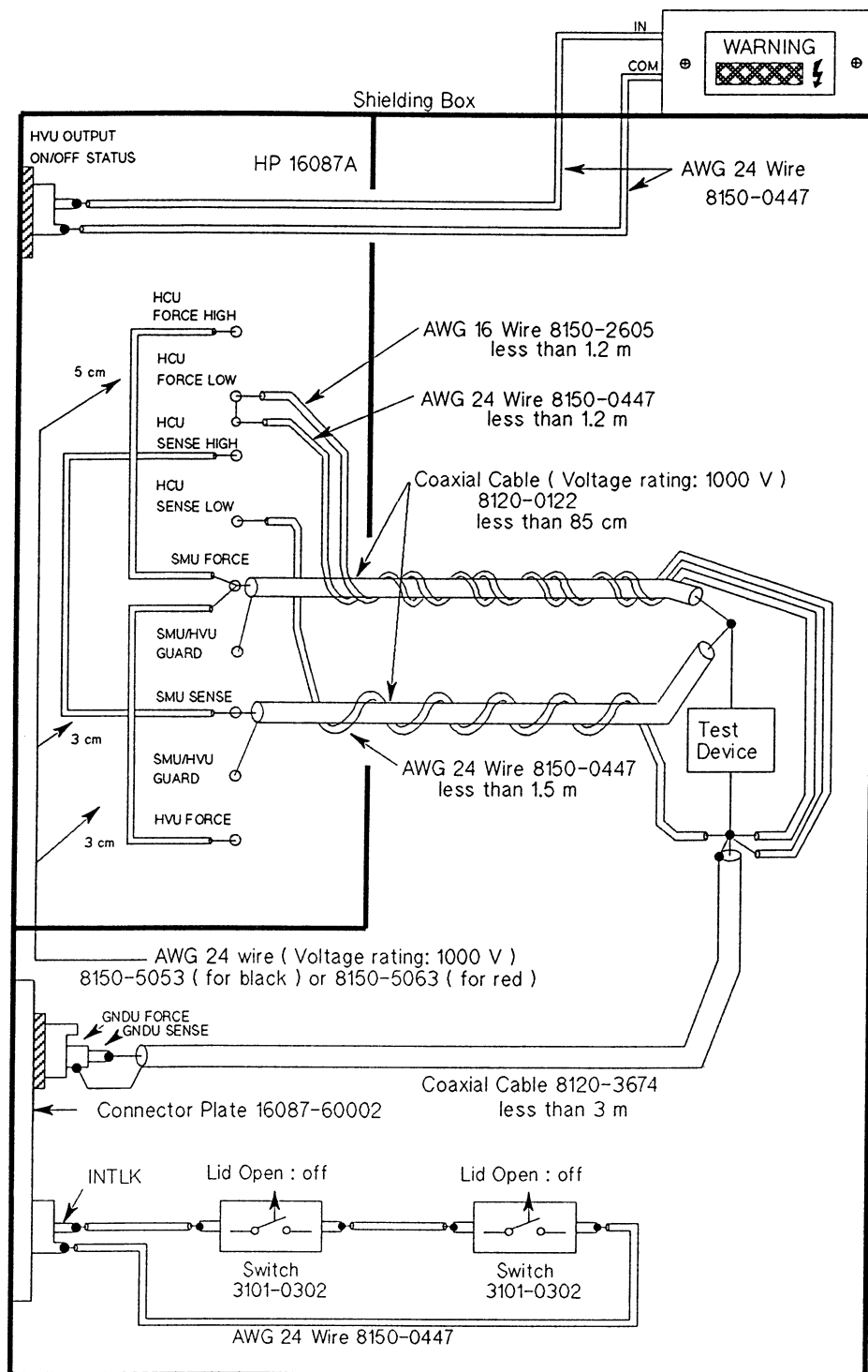
Connections between the HP 16087A and Test Device
