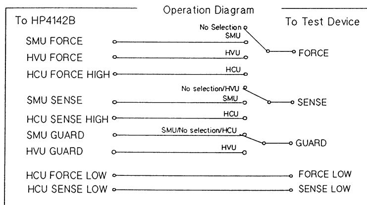
Module Selector Circuit Diagram
