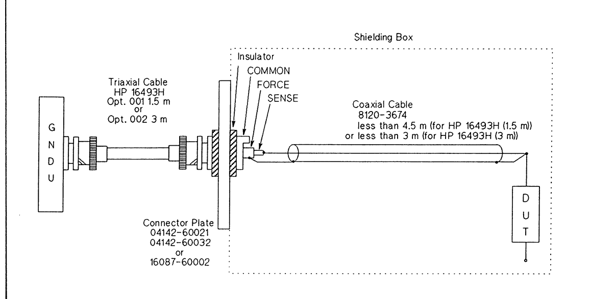
GNDU Example Connections (1 of 2)
