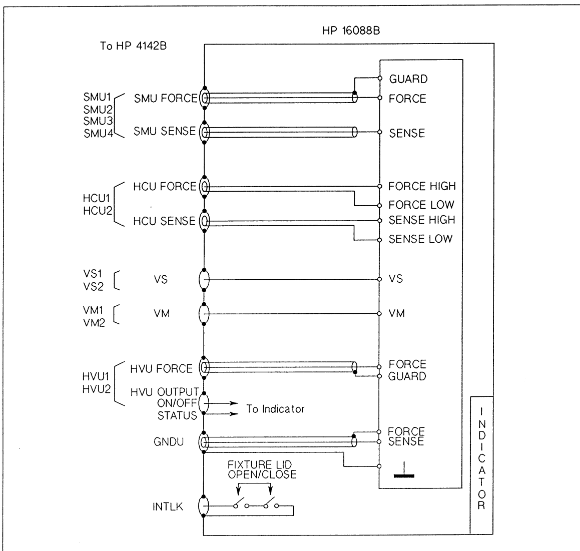
HP 16088B Circuit Diagram
