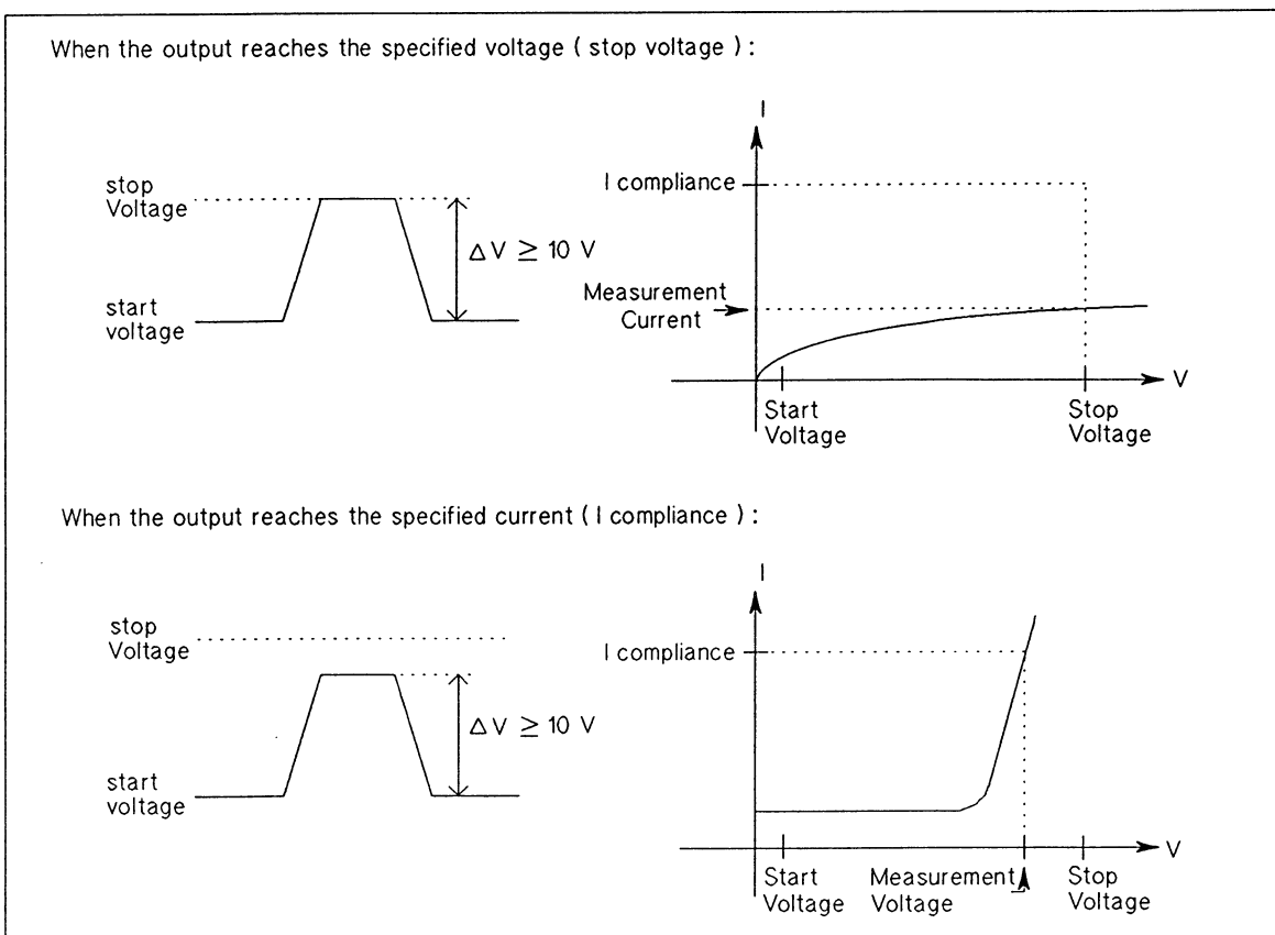
Output Waveform
