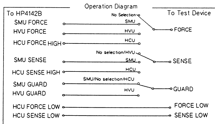
HP 16087A Circuit Diagram
