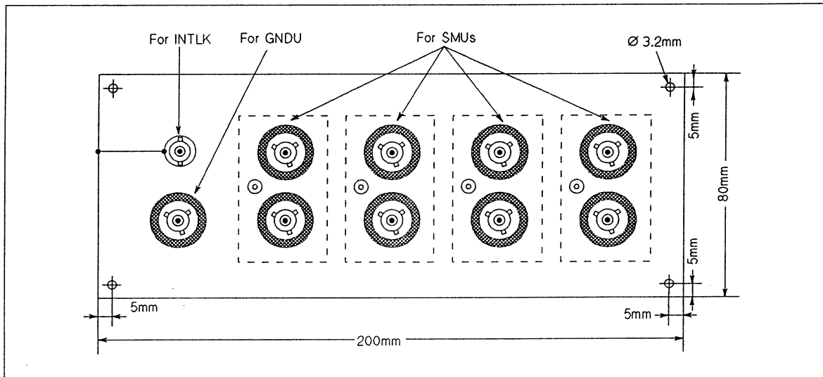
Connector Plate Part Number 04142-60021
