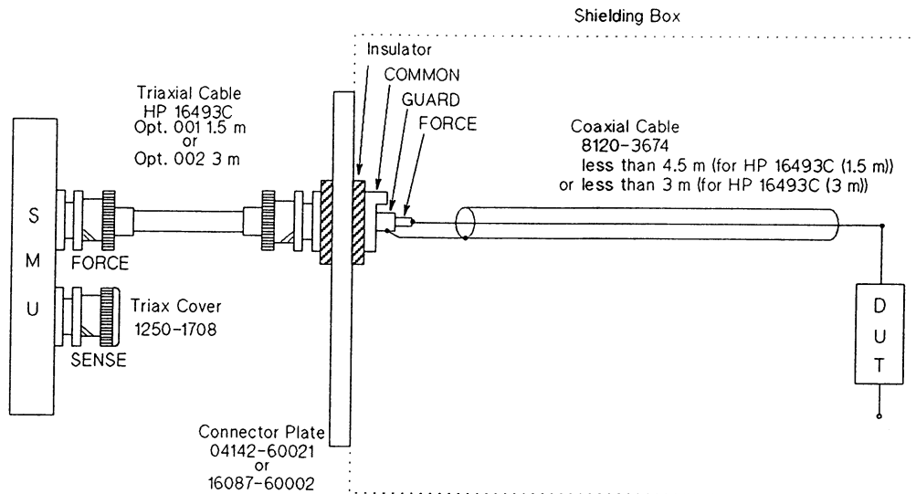
SMU Example Connections (3 of 3)
