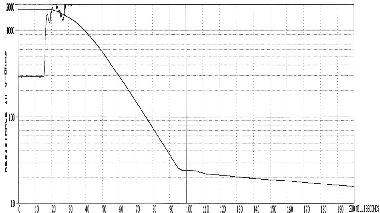
Figure 33. Dynamic Resistance Graph in Semi-Log Scale
