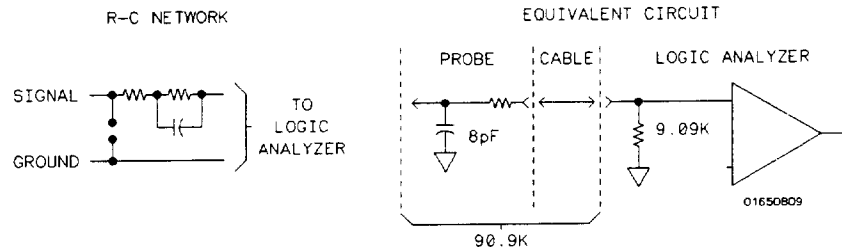
Figure 2-5. Probe Input Circuit
