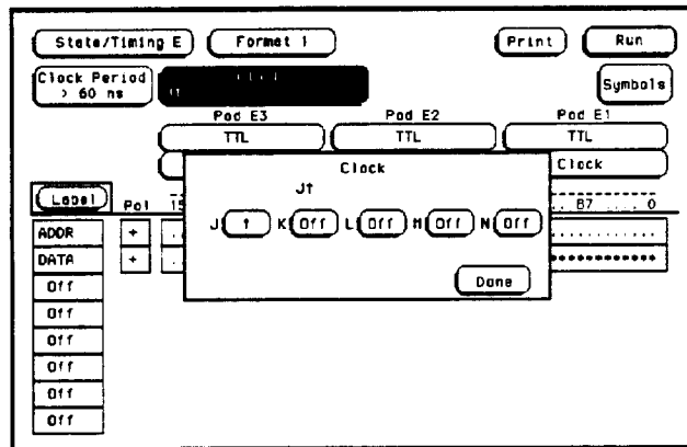
Figure 8-9. Clock Selection
