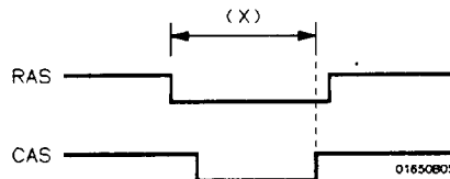
Figure 7-1. RAS and CAS Signals
