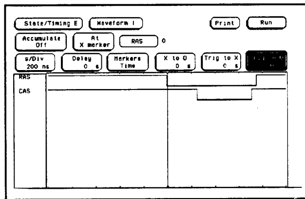
Figure 7-10. Marker Placement
