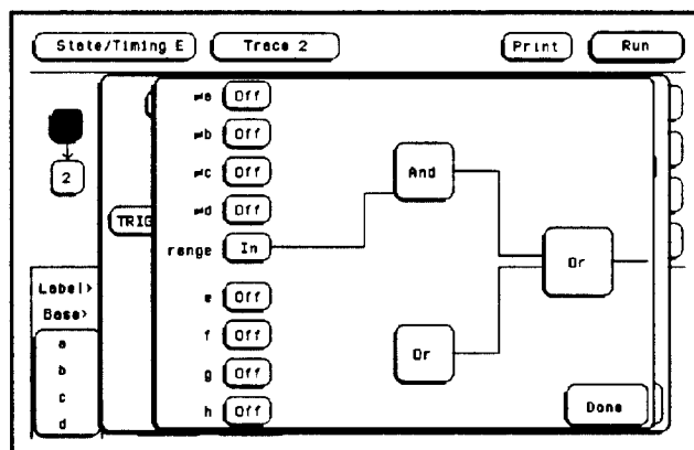
Figure 5-50. Complemented Patterns
