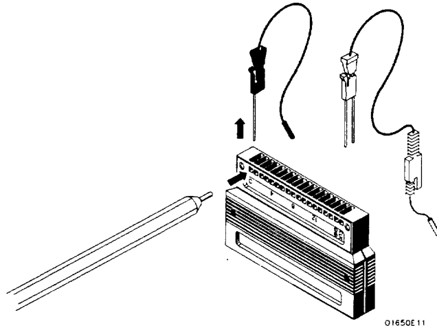
Figure 2-8. Disconnecting Probes from Pods
