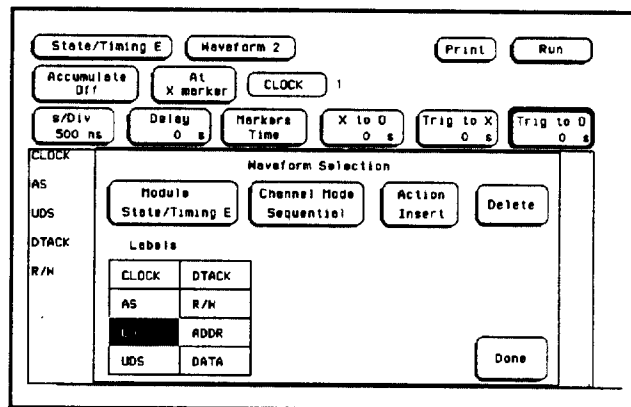
Figure 12-13. Replace Label
