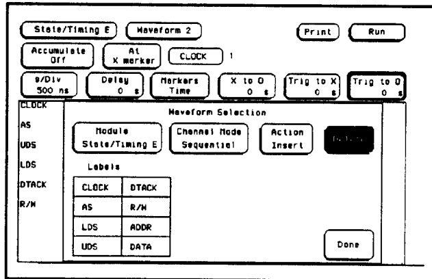
Figure 12-12. Delete Label
