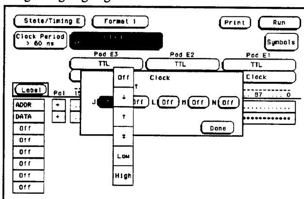
Figure 8-11. Negative-edge Selection
