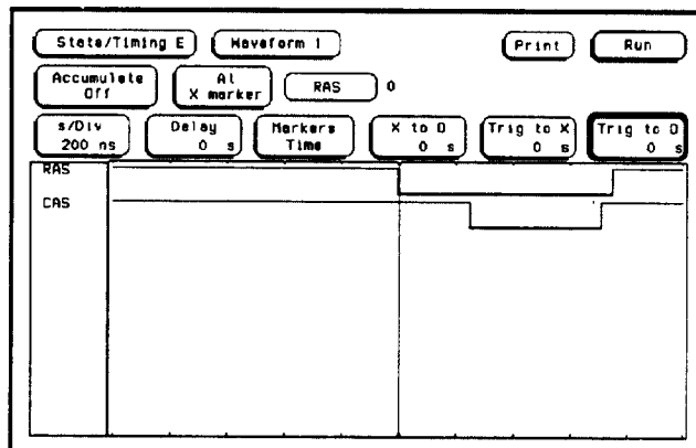
Figure 7-9. Waveform at 200 ns/Div
