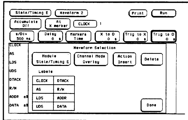
Figure 12-19. Overlapped Waveforms
