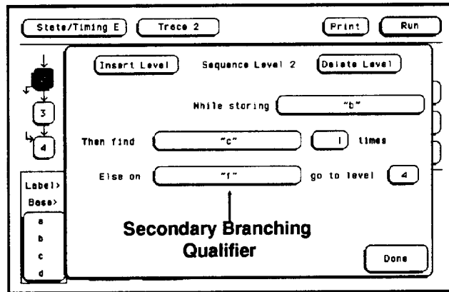
Figure 5-67. Secondary Branching
