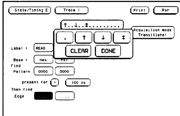
Figure 5-44. Combination of Edges Specified
