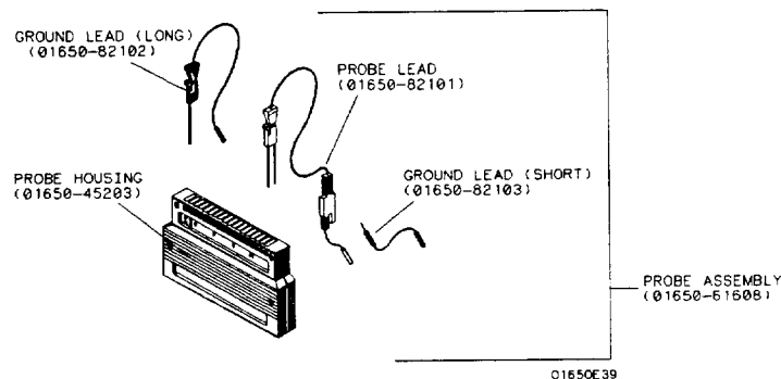
Figure 2-3. Probe Assembly
