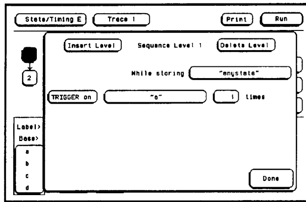
Figure 8-14. Sequence Levels
