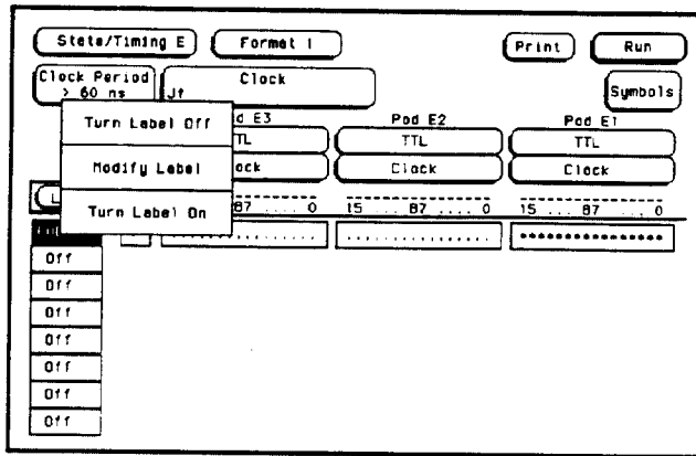
Figure 8-4. Label Selection
