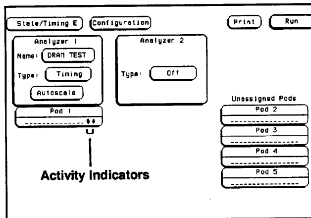
Figure 7-3. Activity Indicators
