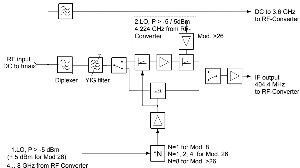
Fig. 3-4 Conversion of the RF to the IF from 3.6 GHz
