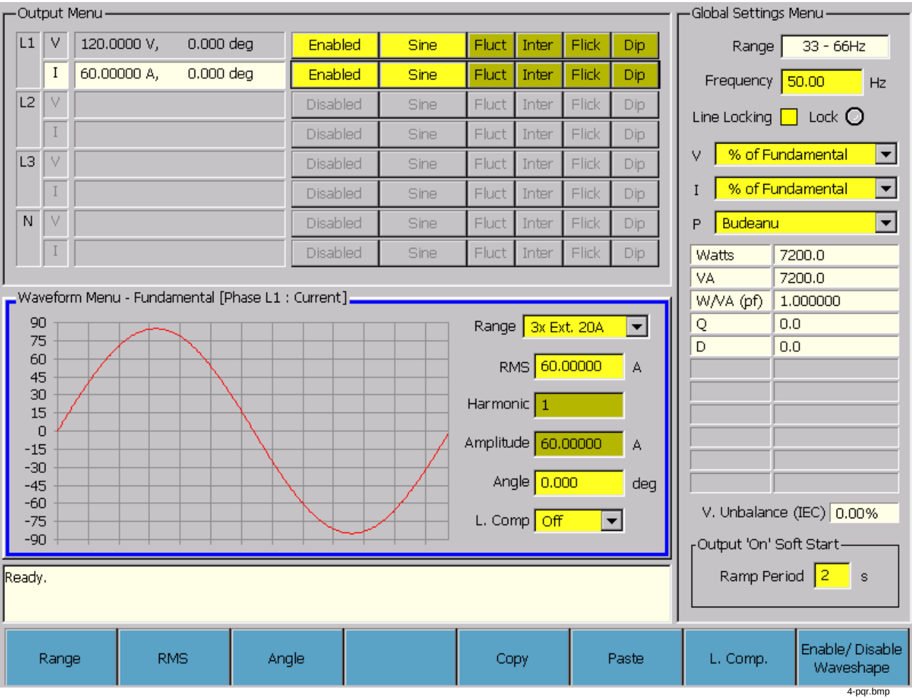
Figure 4-45. Output Menu
