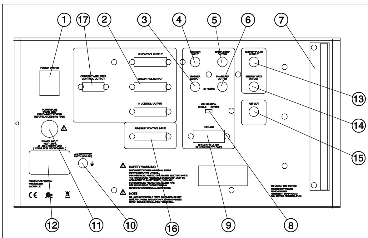
Figure 3-13. Rear-Panel Features
