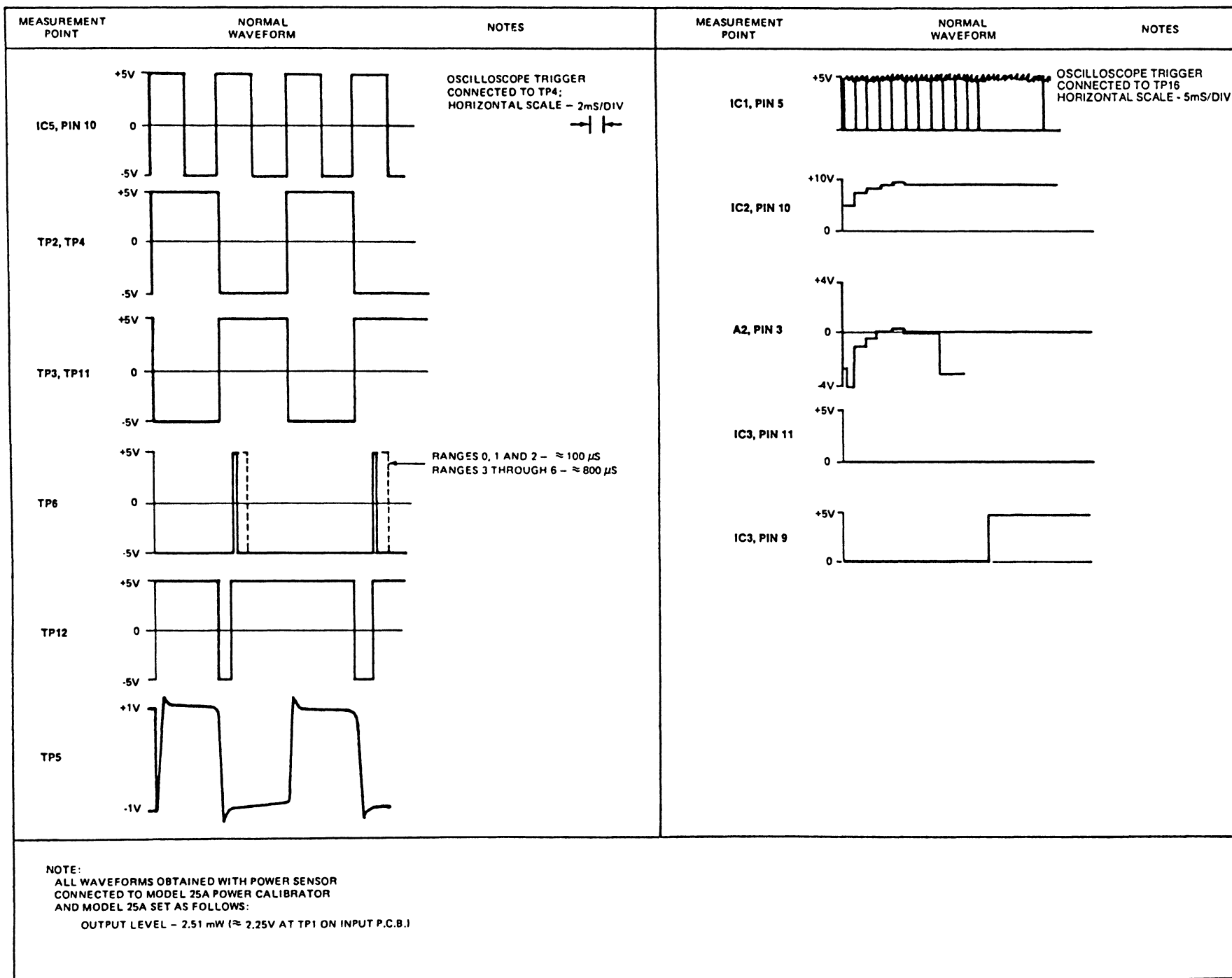
Figure 4-2 Input P.C. Board, Voltage and Waveform Data
