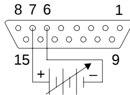
Figure 2-1 Connector J1
