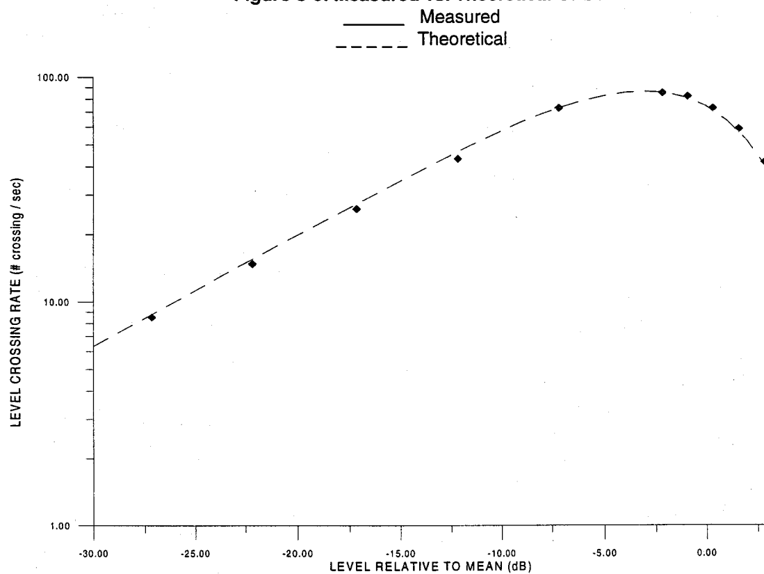
Figure 3-10. Measured vs. Theoretical LCR
