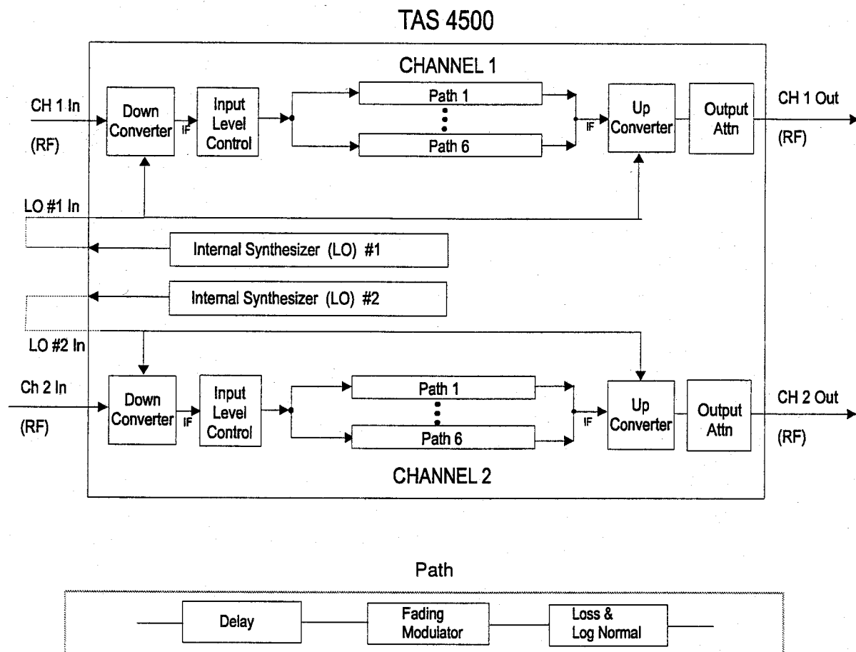
Figure 1-1. TAS 4500 Block Diagram
