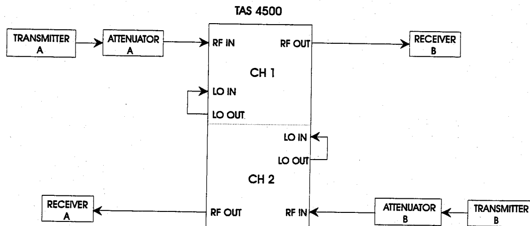
Figure 1-6. Duplex Channel Configuration
