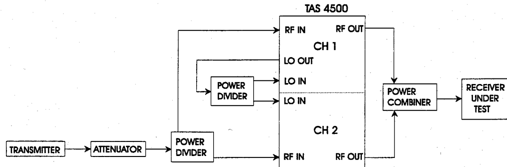
Figure 1-5. Single Channel 12 Path Configuration
