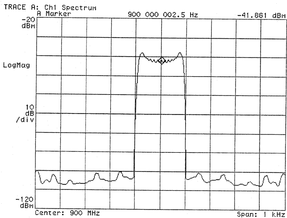
Figure 3-8. Measured Rayleigh Power Spectral Density
