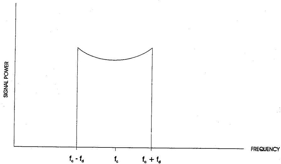
Figure 3-7. Theoretical Rayleigh Power Spectral Density
