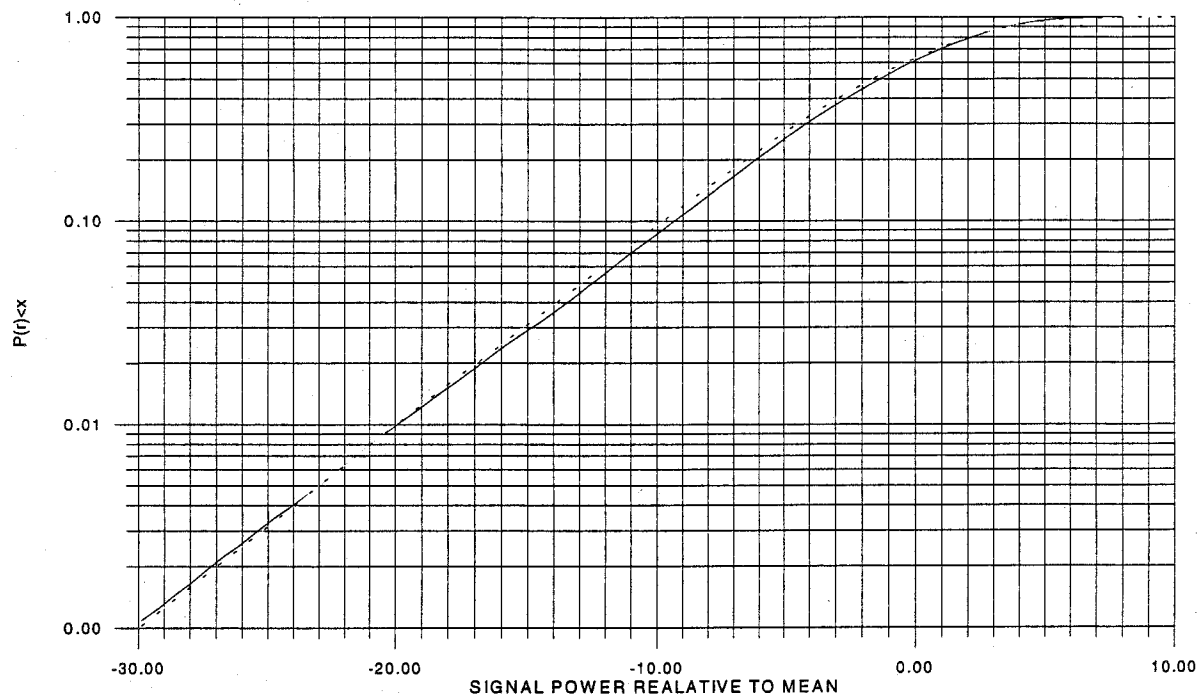
Figure 3-9. Measured vs. Theoretical CPDF
