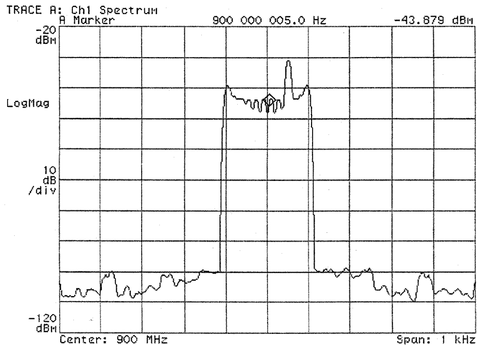
Figure 3-14. Measured GSM Rician Fading Power Spectral Density
