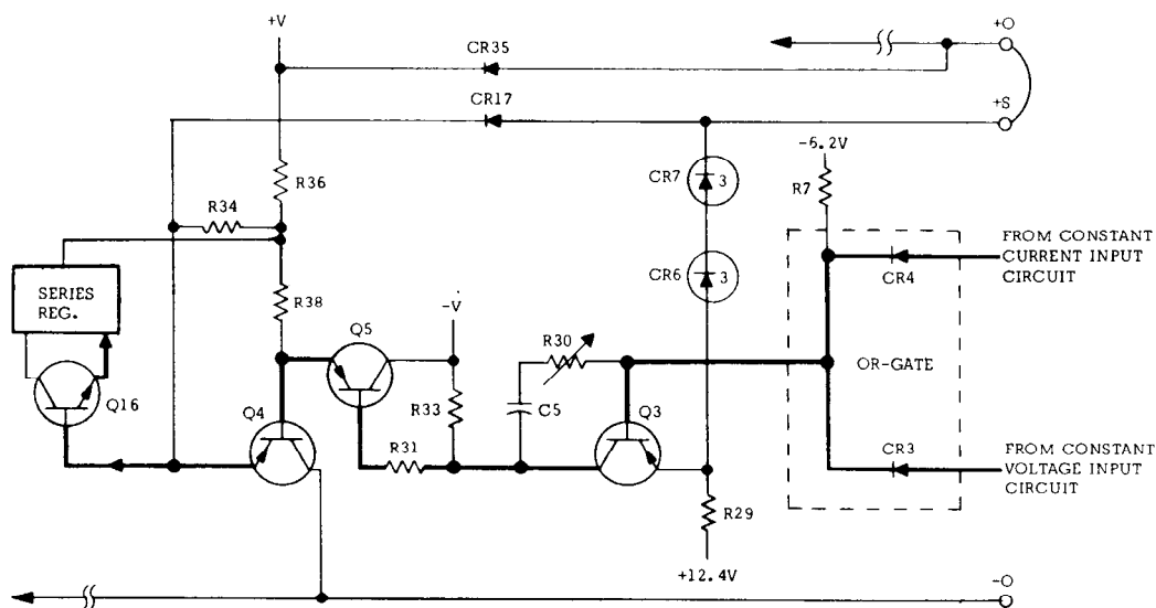
Figure 4-6. Mixer and Error Amplifiers, Simplified Schematic
