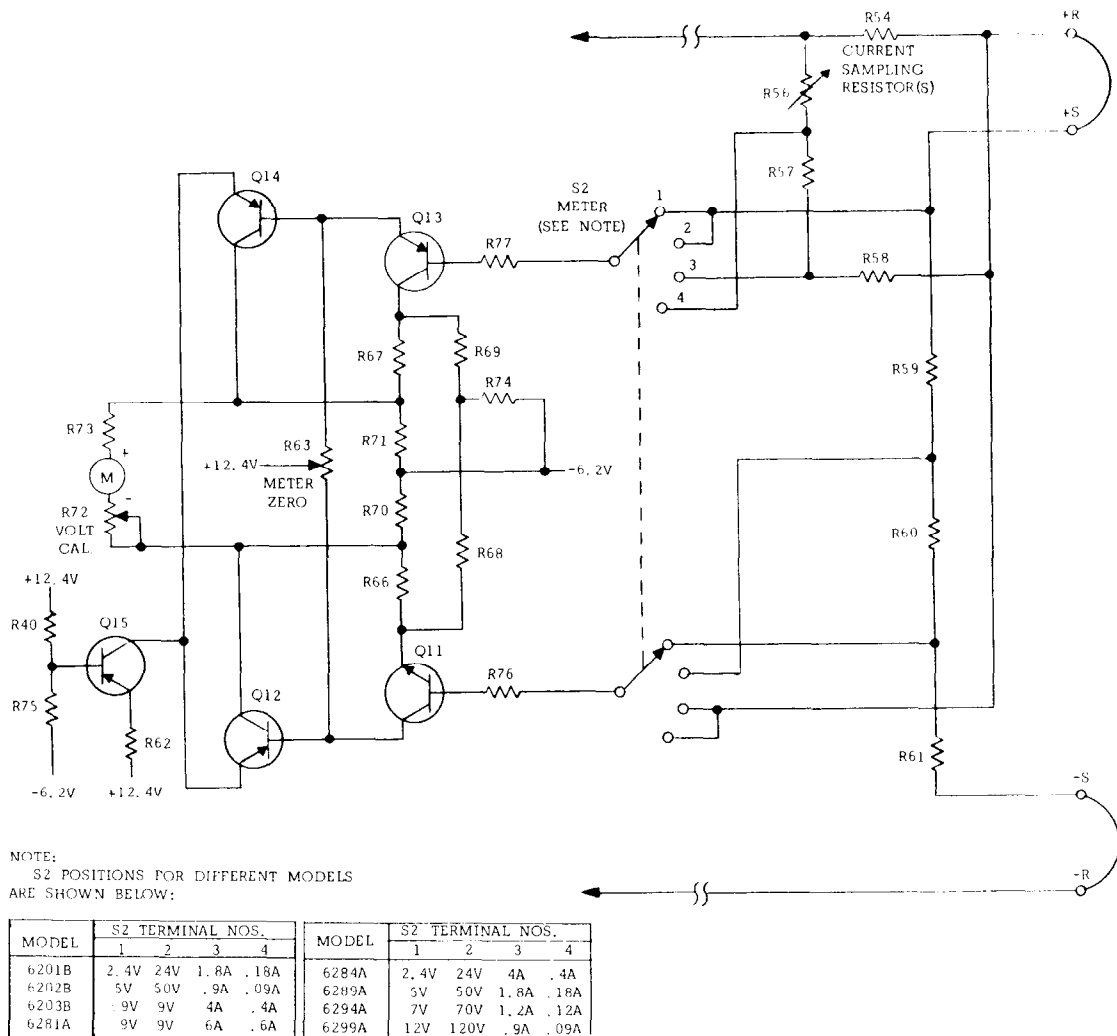
Figure 4-7. Meter Circuit, Simplified Schematic
