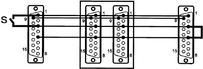
Wiring diagram for the interlock system:
