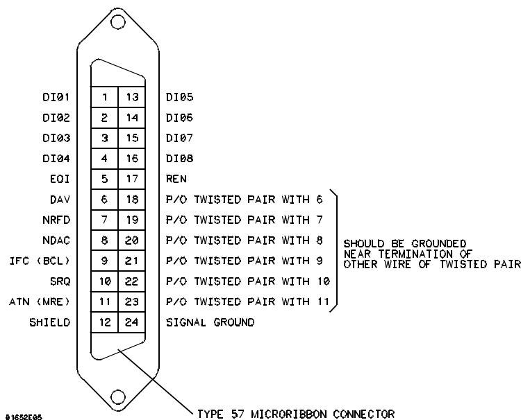
GPIB Interface Connector
