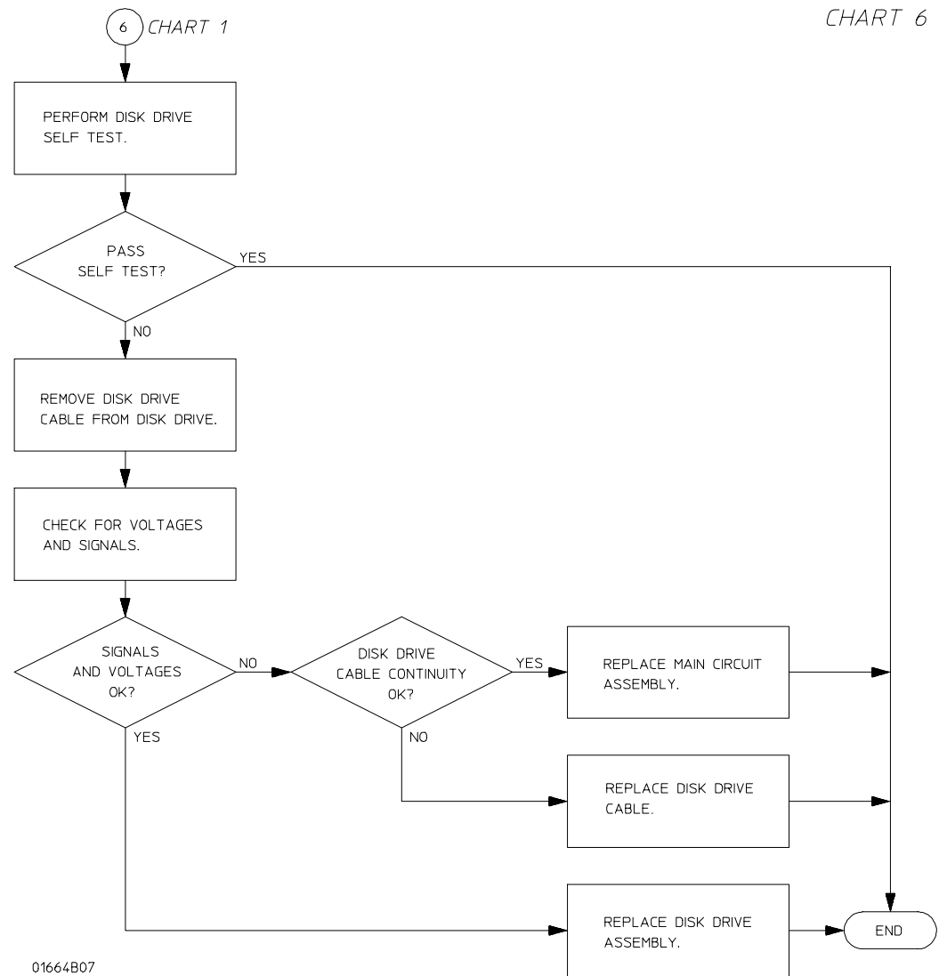
Troubleshooting Flowchart 6
