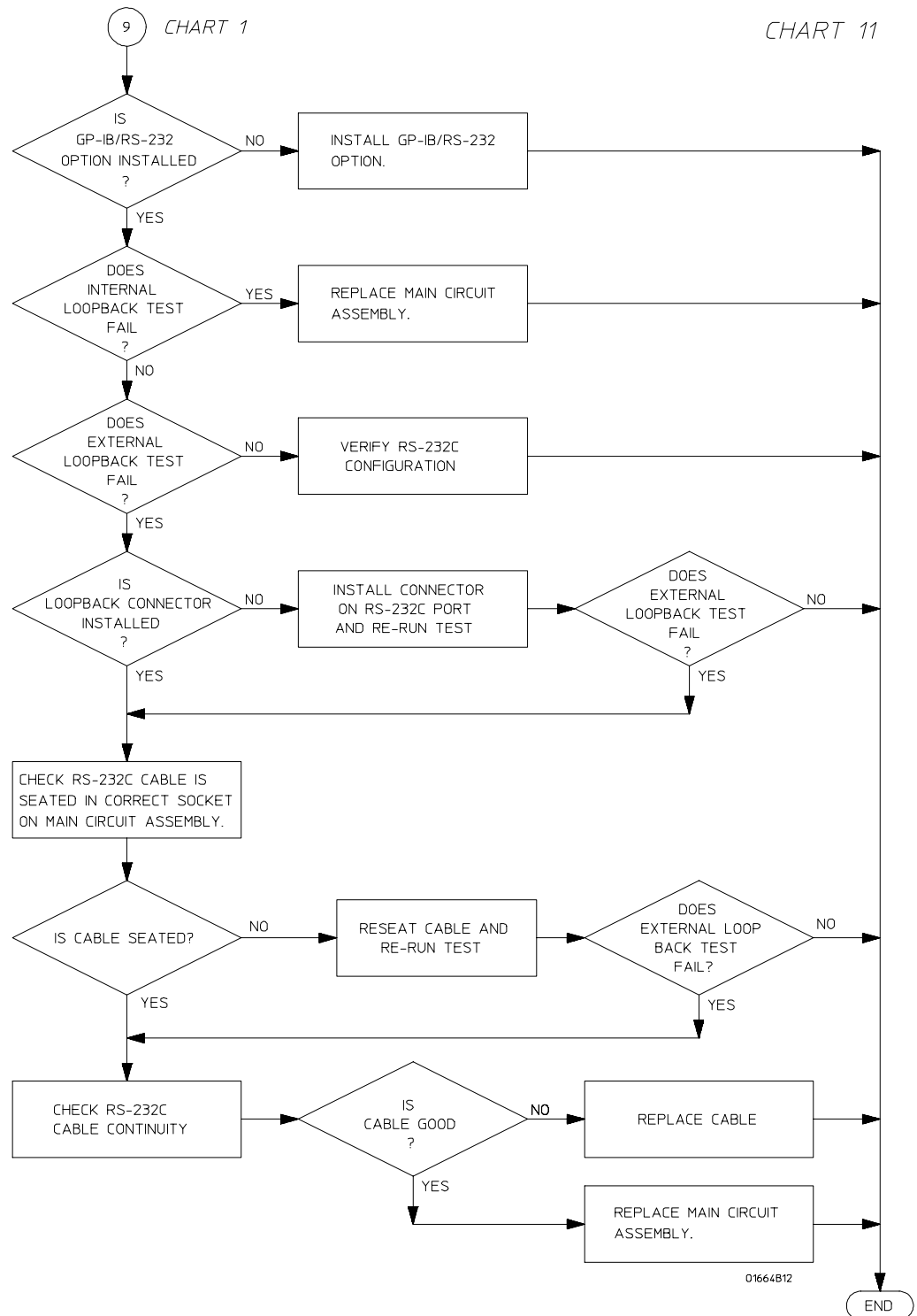
Troubleshooting Flowchart 11
