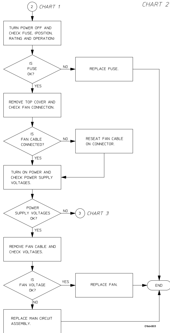
Troubleshooting Flowchart 2
