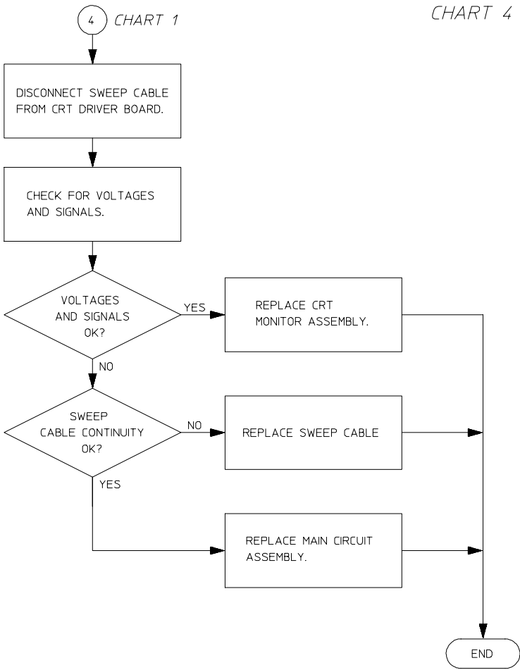
Troubleshooting Flowchart 4
