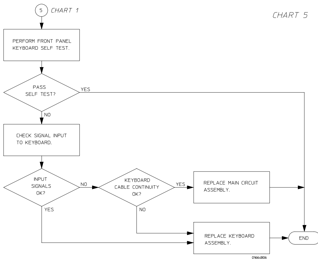
Troubleshooting Flowchart 5
