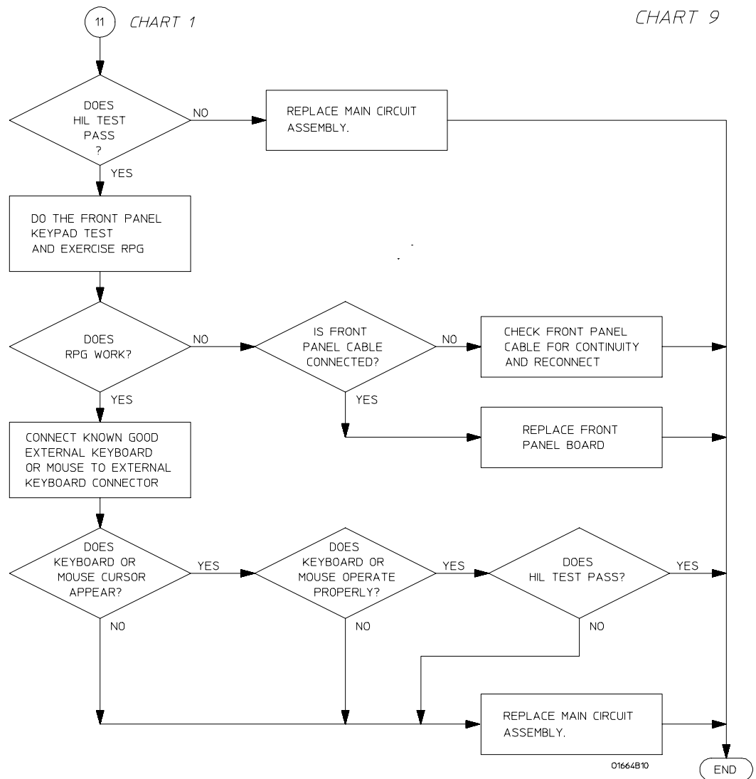
Troubleshooting Flowchart 9
