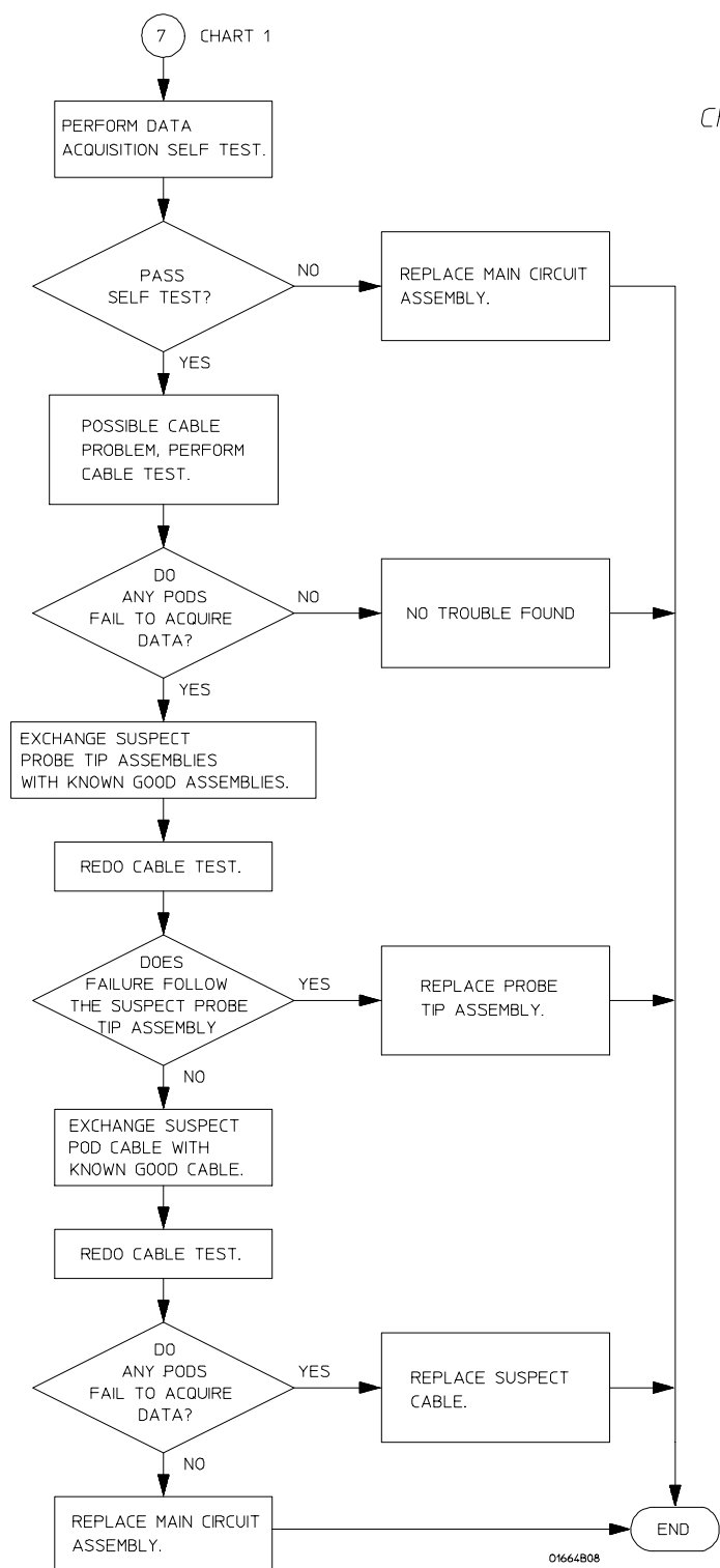
Troubleshooting Flowchart 7
