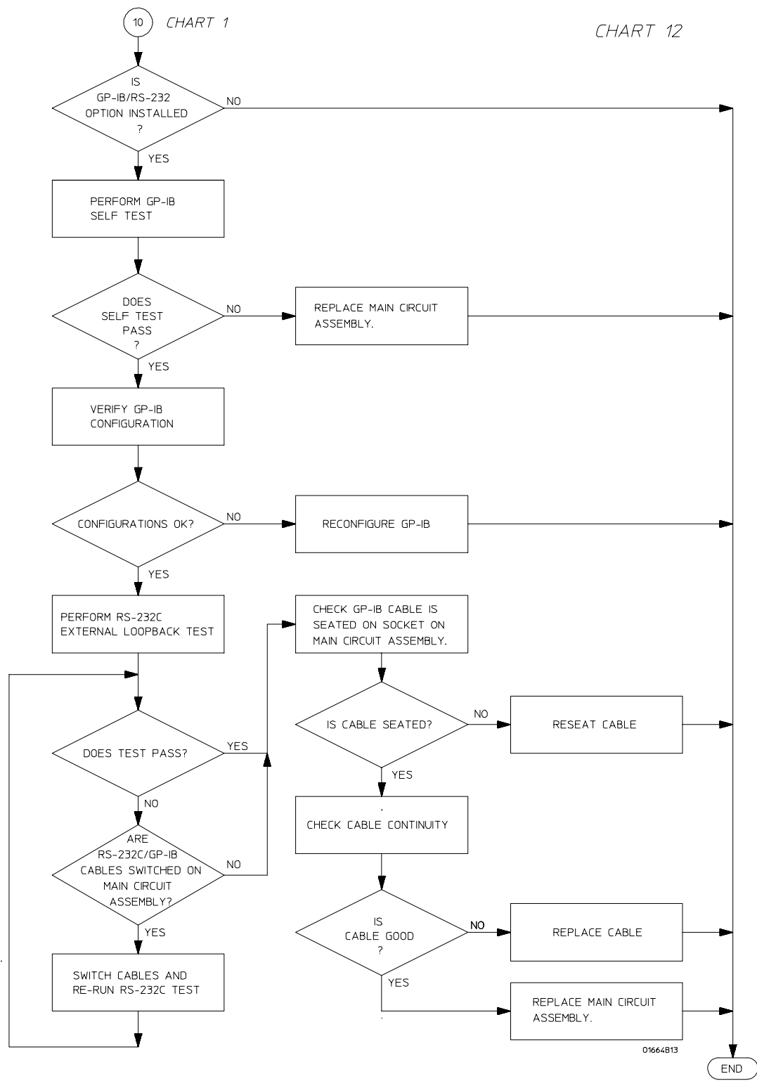
Troubleshooting Flowchart 12
