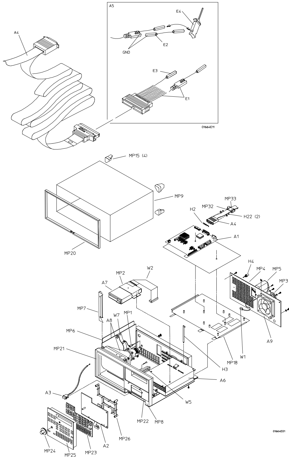
Exploded view of the 1664A logic analyzer.
