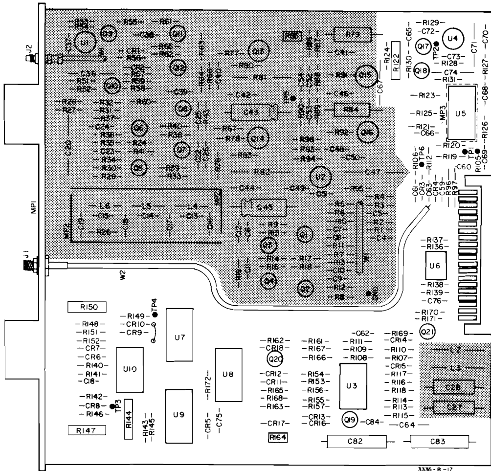
A6 -hp- Part No. 03335-66508 Level Control
