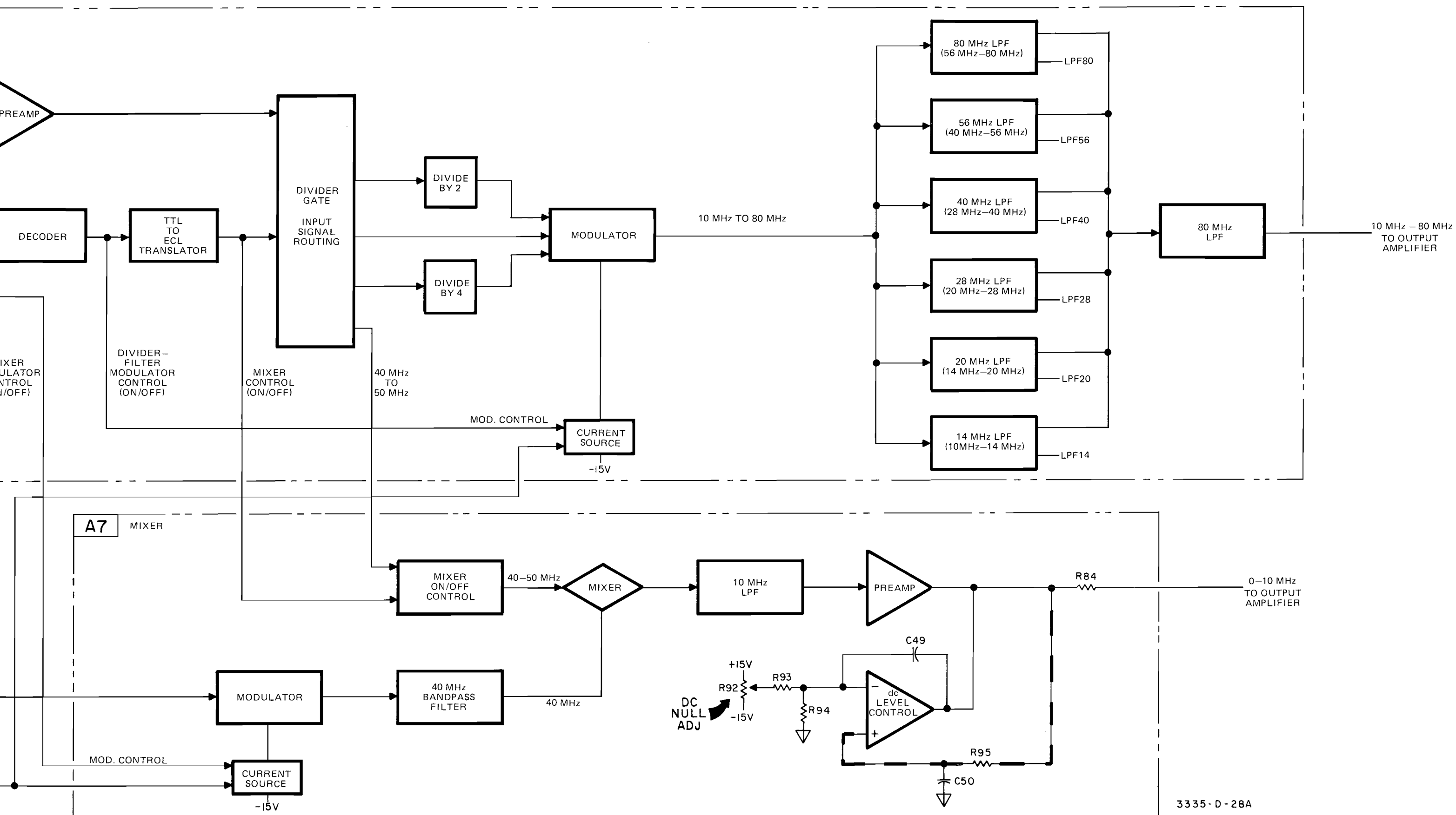
Figure 8-L-2. Block Diagram, Divider-Filter (03335-66536) A2 Mixer (03335-66507) A7.
