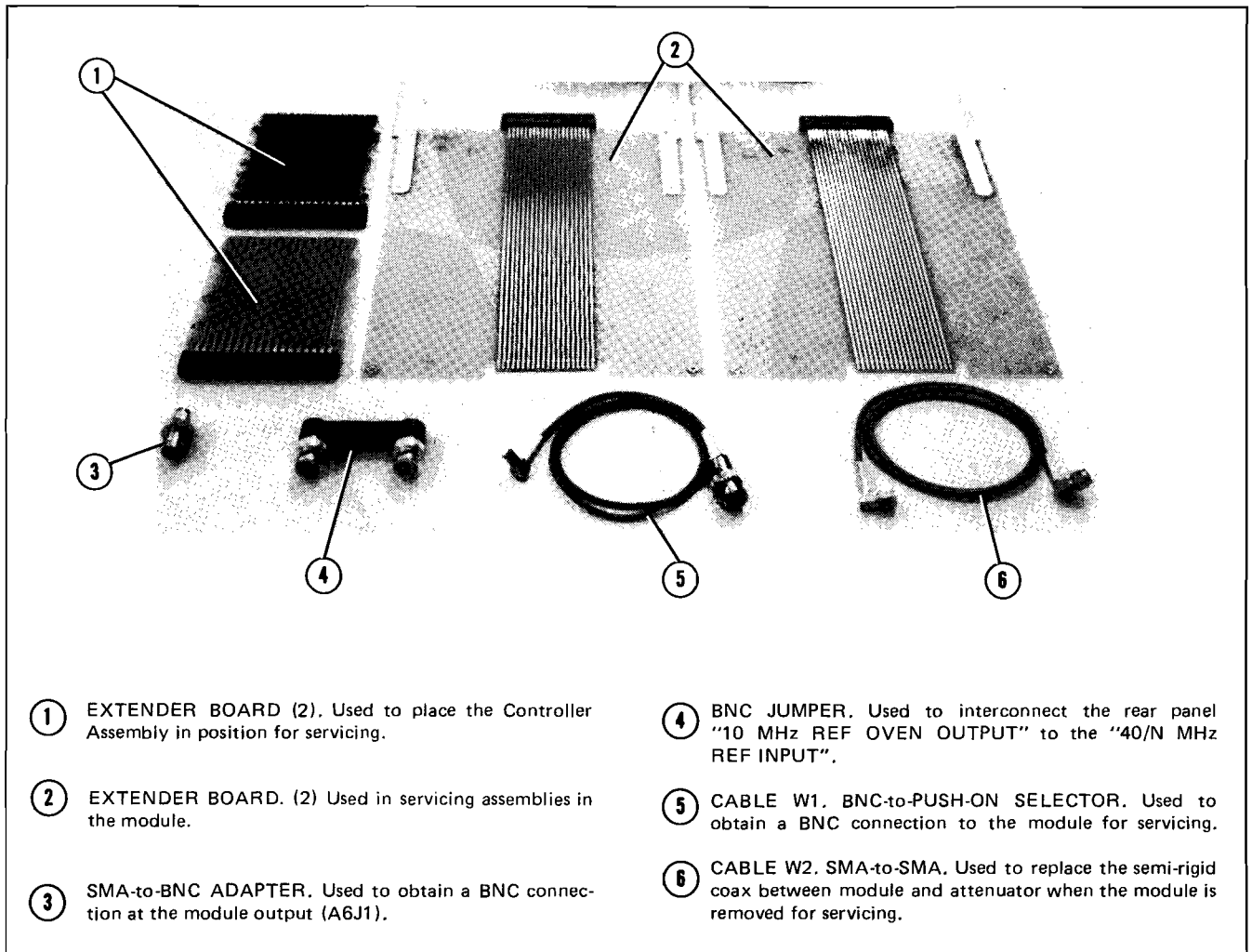
Figure 8-49. Service Items.
