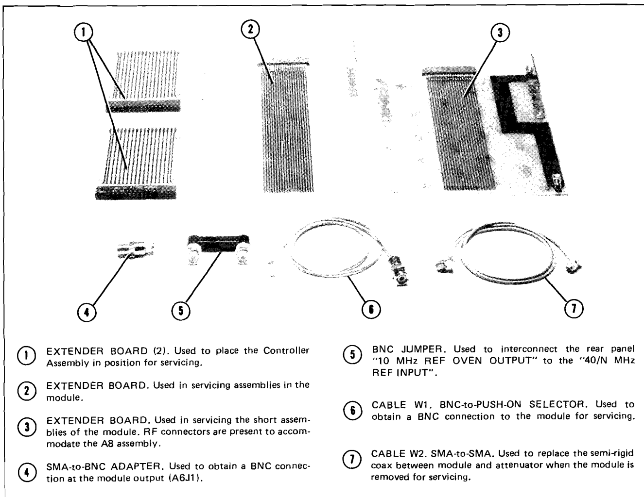
Figure 8-49. Service Items.
