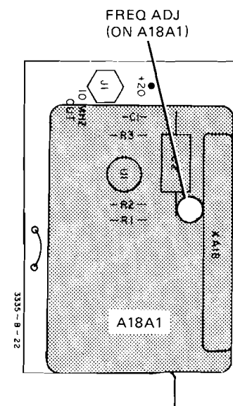
A18 TEMP-STABILIZED OSCILLATOR INTERFACE (OPTION 001) 03335-66517
