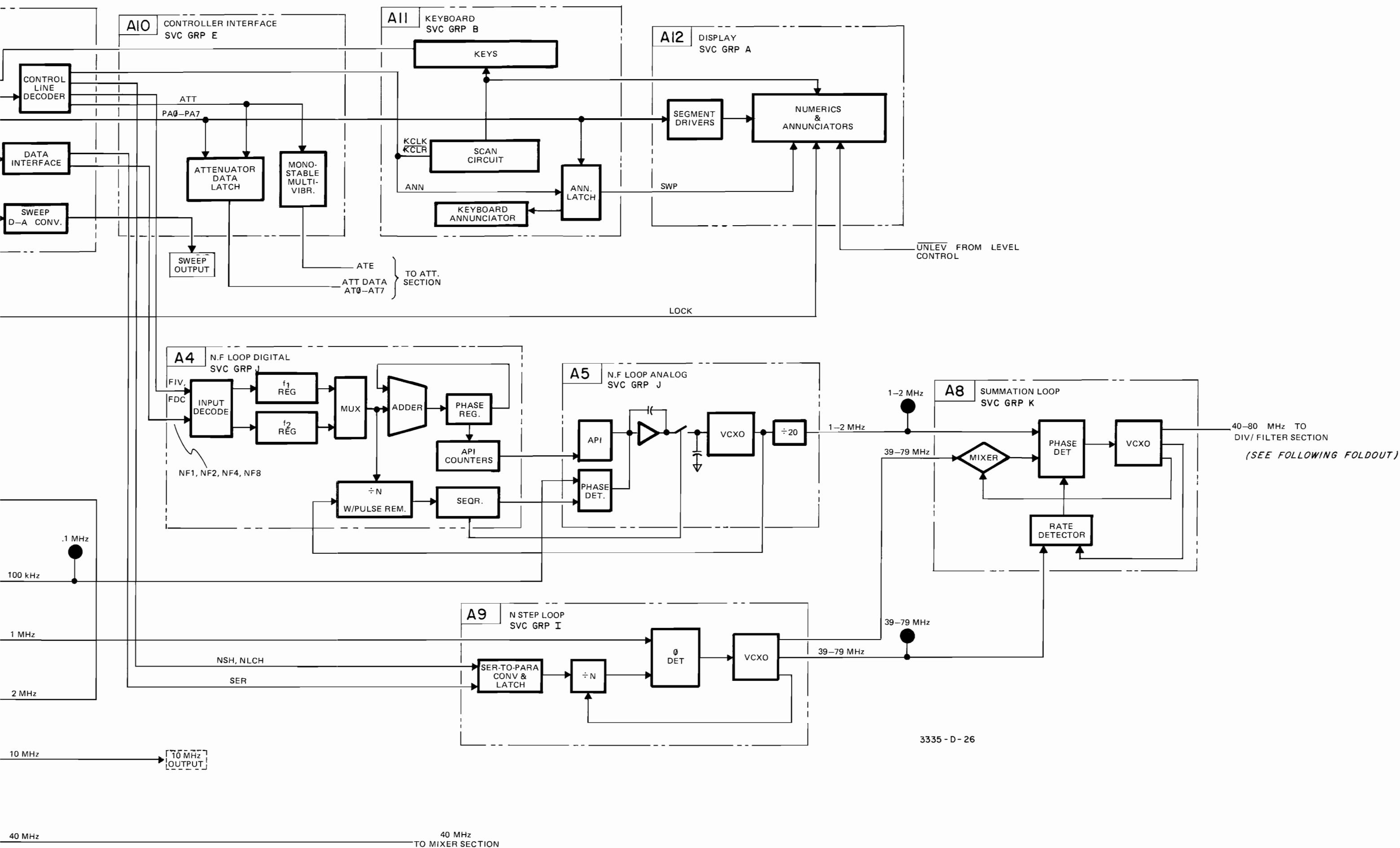
Figure 8-O-2. Block Diagram, Instrument Functional Block Diagram. 8-O-7/8-O-8
