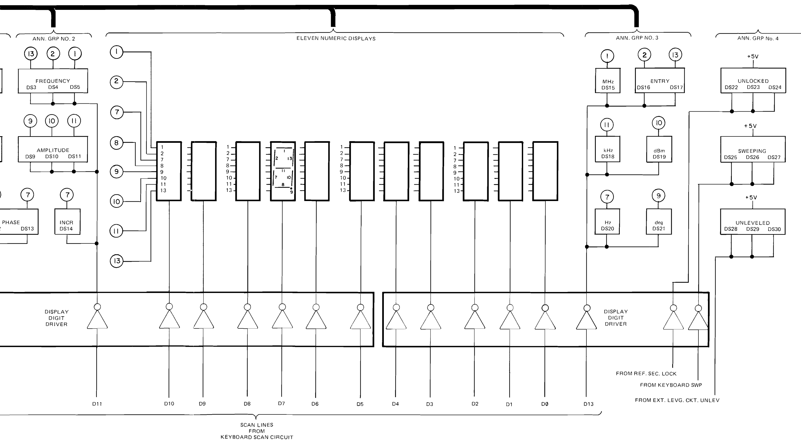
Figure 8-A-2. Block Diagram, Display (03335-66509) A12. 8-A-7/8-A-8
