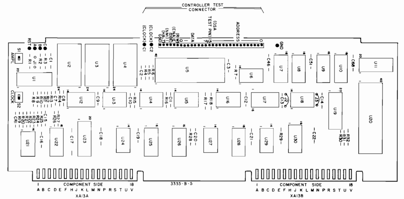
A13 -hp- Part No. 03335-66511
