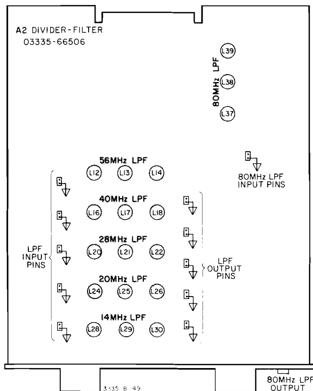
Figure 5-3. Filter Adjustment Location.
