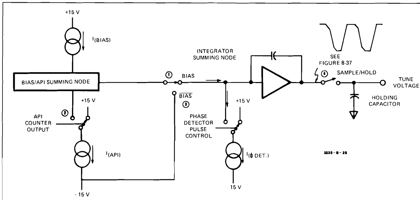
Figure 8-36. N.F. Loop Integrated Currents.
