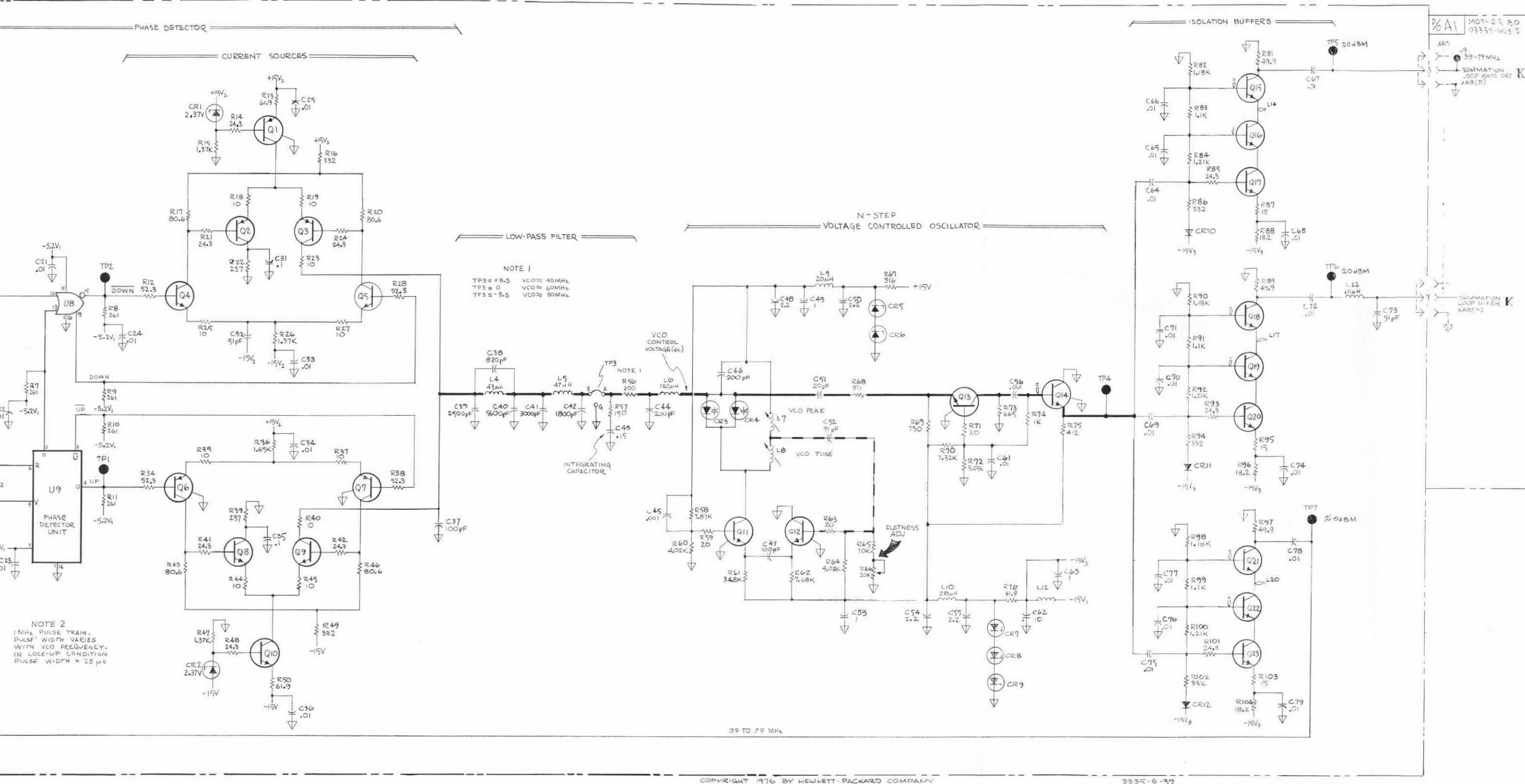
Figure 8-I-1. Schematic Diagram, N Step Loop (03335-66501) A9. 8-I-7/8-I-8
