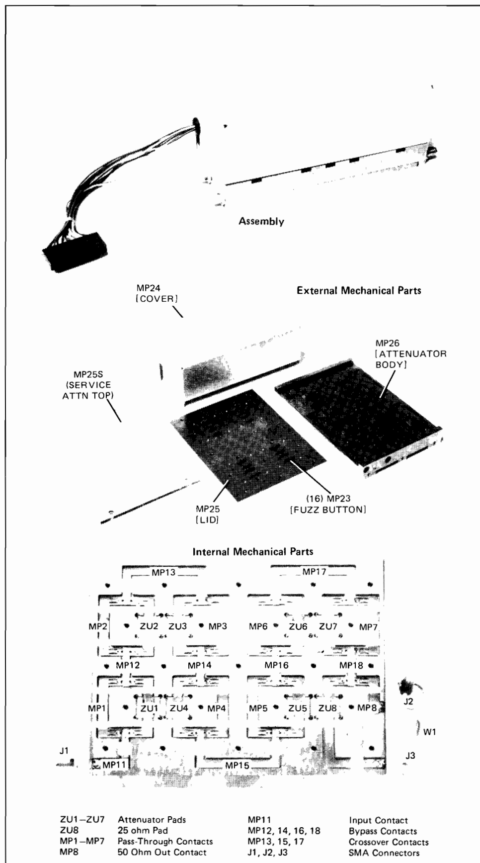
Figure 8-N-2. A25 Attenuator
