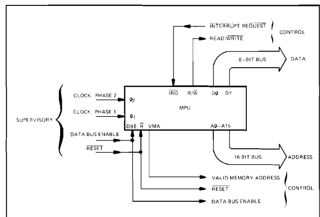
Figure 8-6. MPU I/O; Data, Address, Supervisory and Control.
