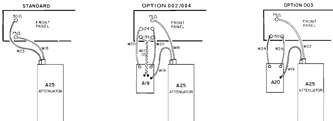
Figure 6-2. Cable Identification.
