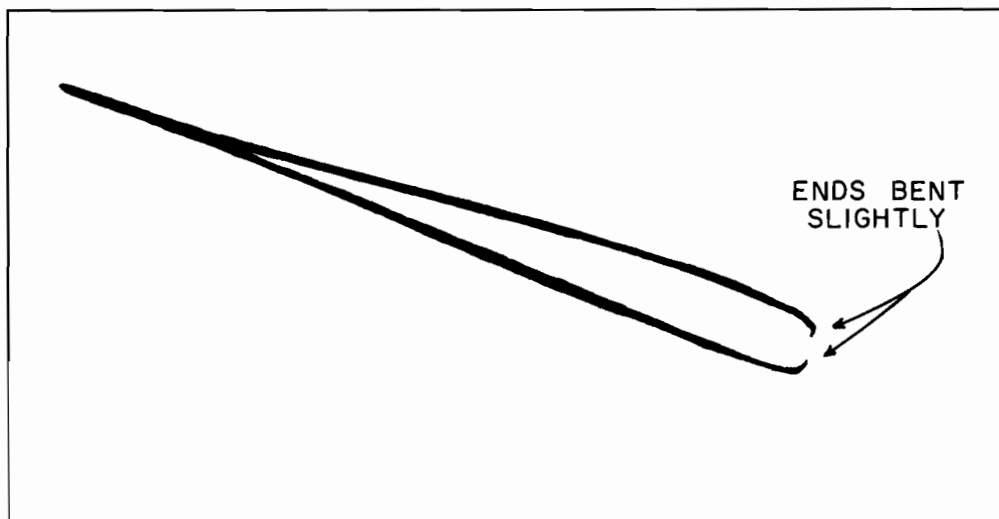
Figure 8-N-1. Tweezer Modification.
