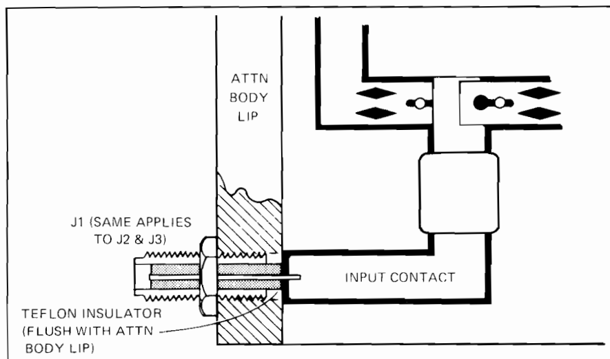
Figure 8-N-9. Connector Installation.
