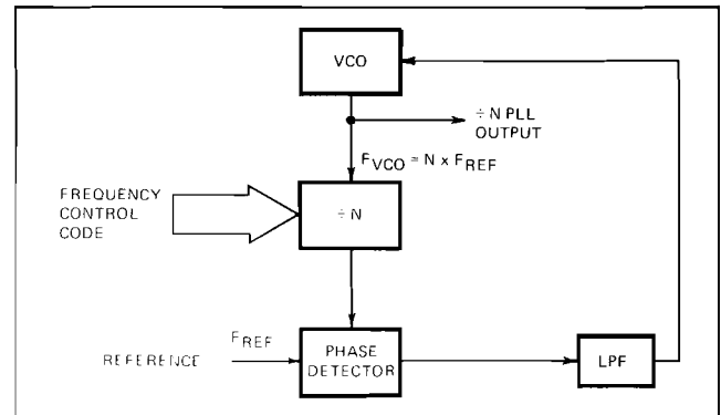
Figure 8-17. Basic Diagram, N Step Loop.
