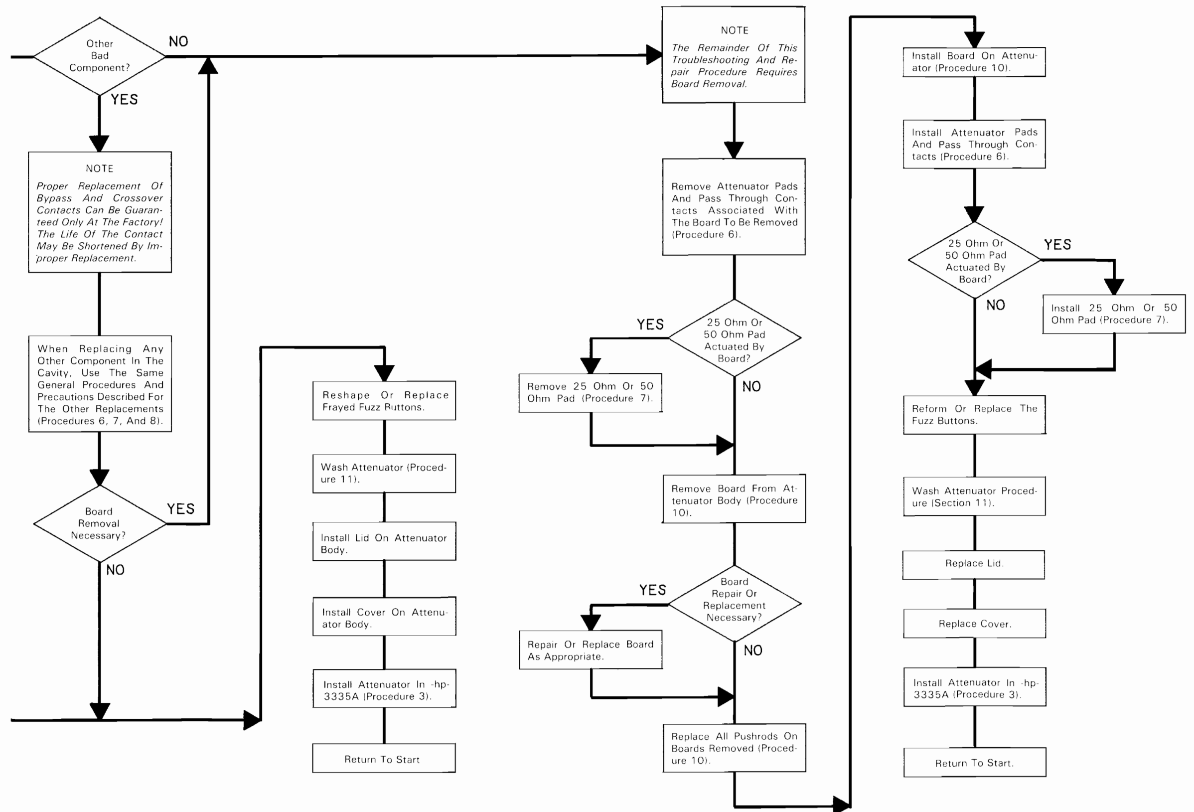
Figure 8-N-14. Attenuator Troubleshooting Tree (Cont'd). 8-N-17/8-N-18(A)
