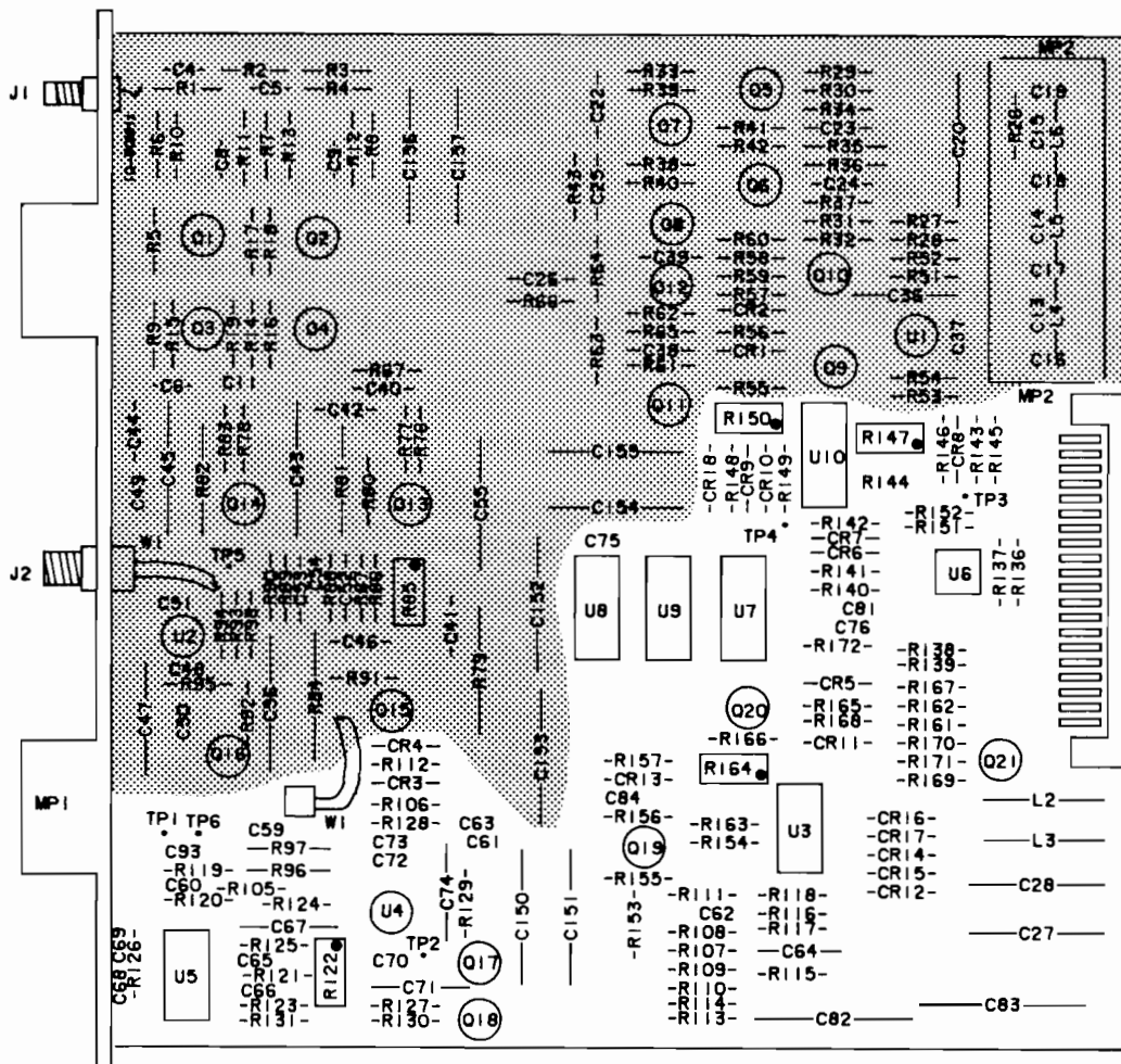
A6 -hp- Part No. 03335-66538 Level Control
