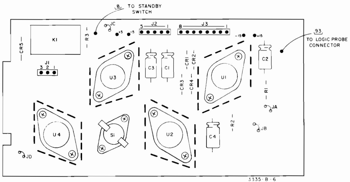
A15 -hp- Part No. 03335-66516
