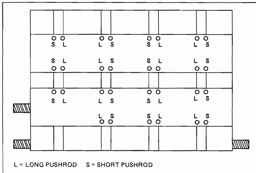
Figure 8-N-12. Pushrod Placement.
