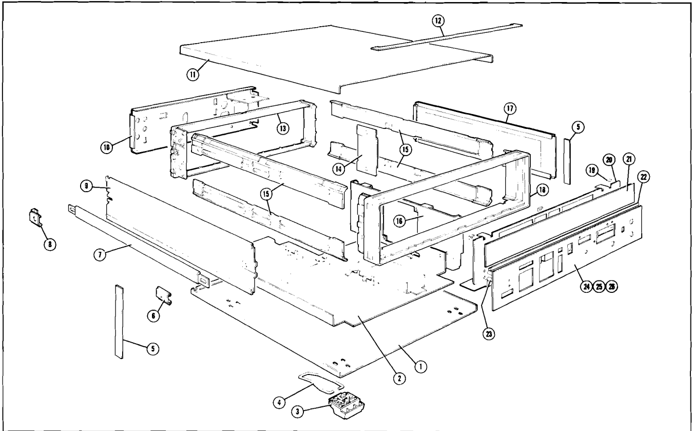
Figure 6-1. Mechanical Parts Identification.
