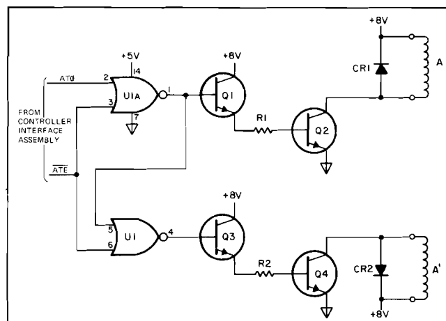
Figure 8-46. Relay Energizing Circuit, Typical.
