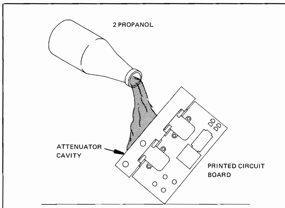
Figure 8-N-13. Attenuator Wash.
