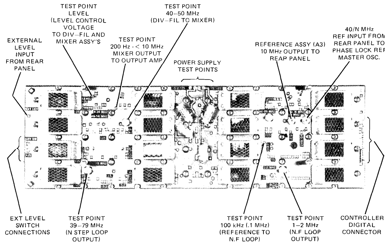
A1 MOTHER 03335-66515 (TEST CONNECTOR LOCATIONS)
