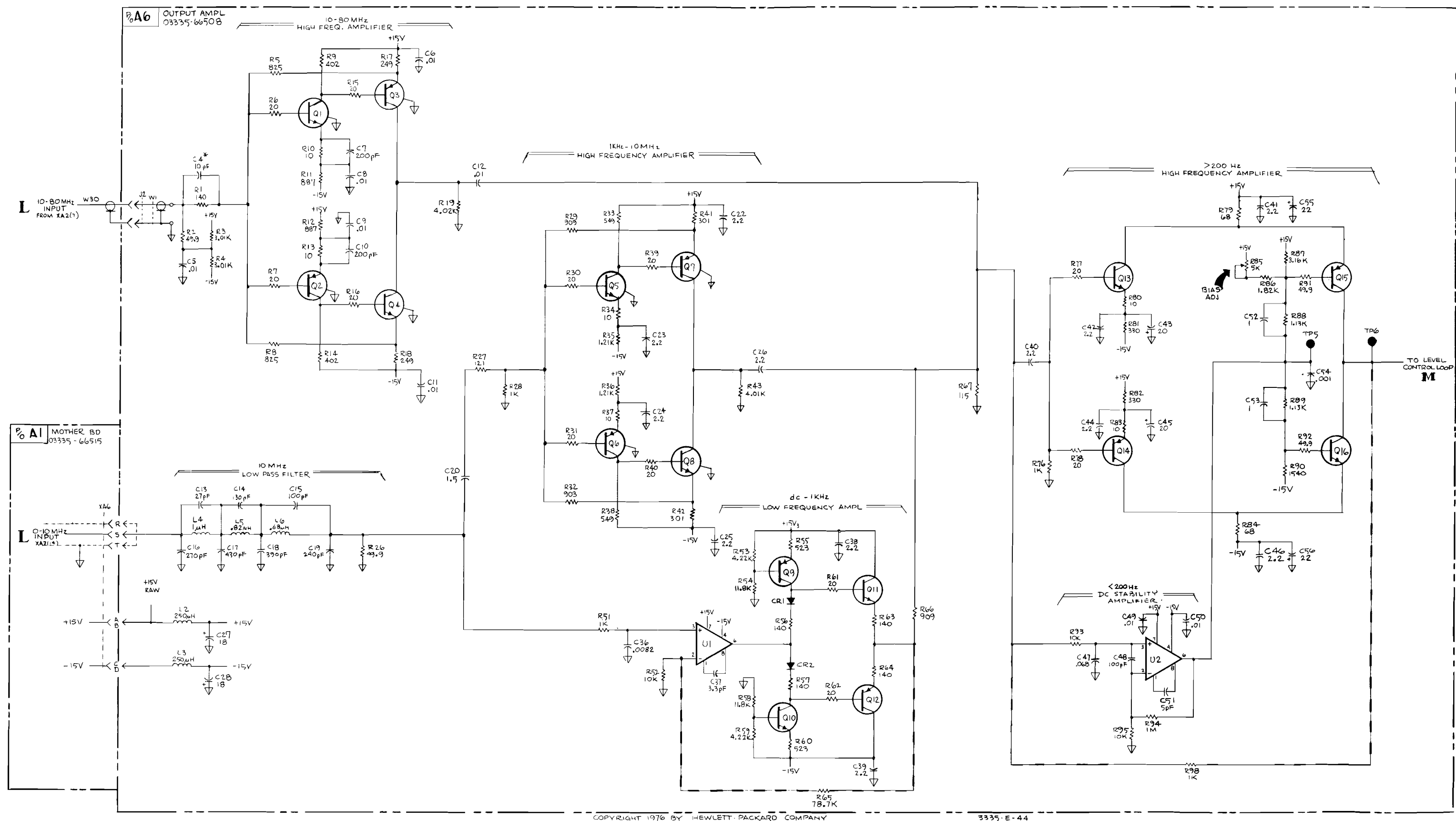
Figure 8-M-1. Schematic Diagram, Output Amplifier (03335-66508) A6. Backdating 8-M-9/8-M-10
