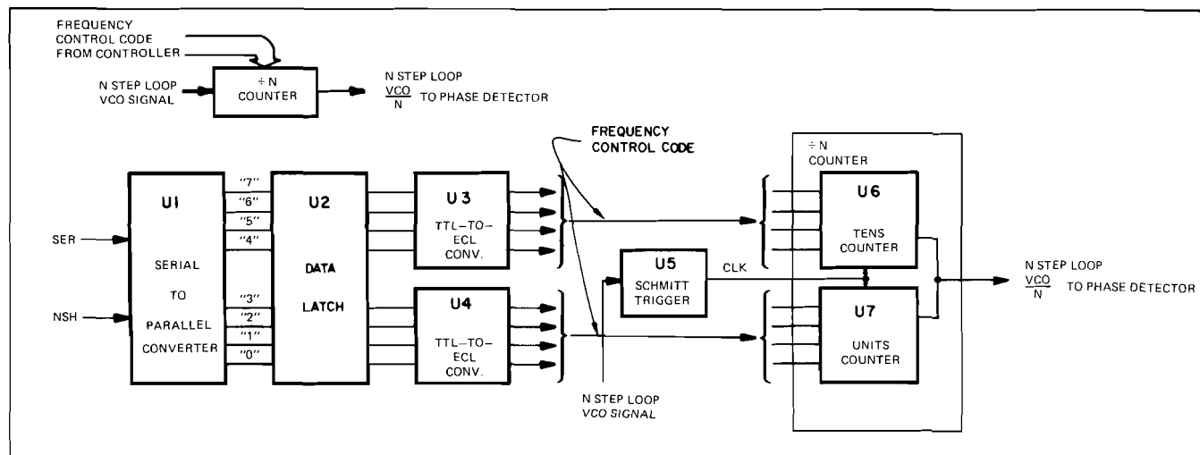
Figure 8-19. Divide-by-N Counter.
