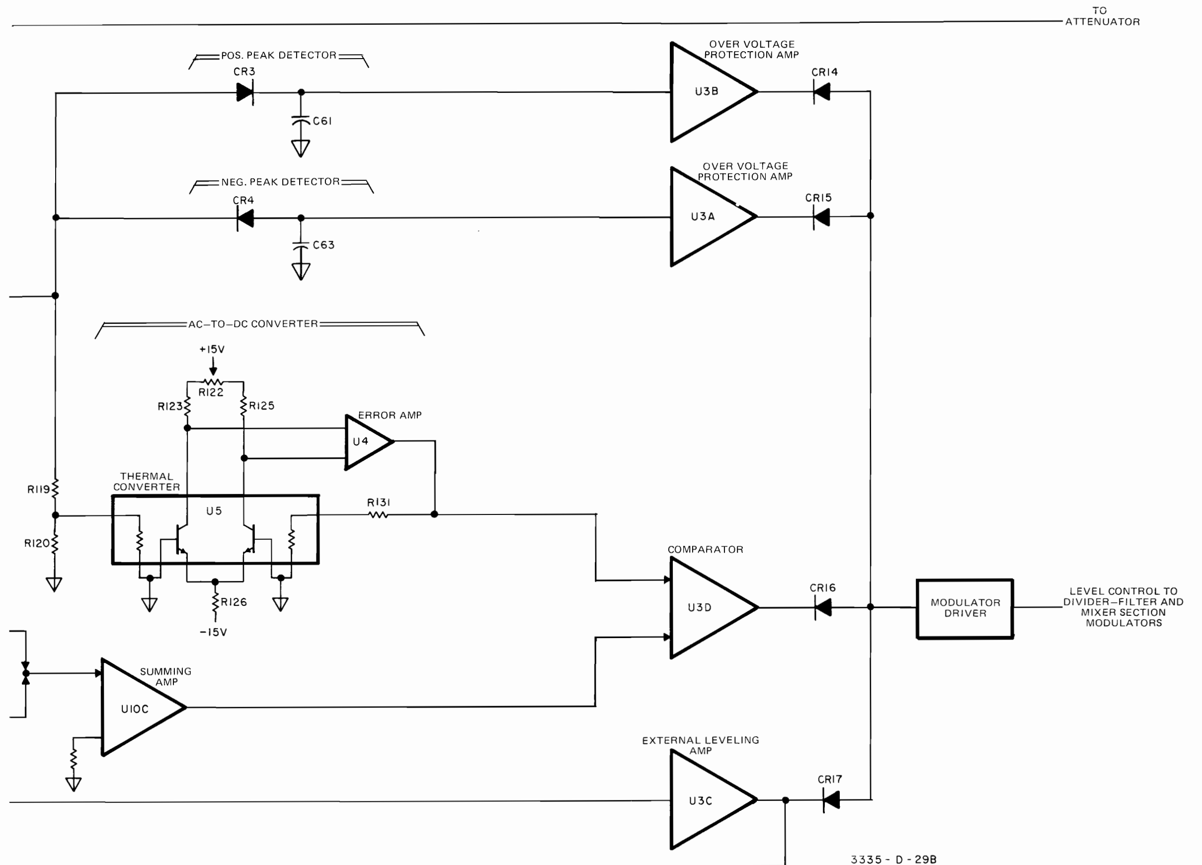
Figure 8-M-4. Block Diagram, Level Control (03335-66538) A6. 8-M-15/8-M-16
