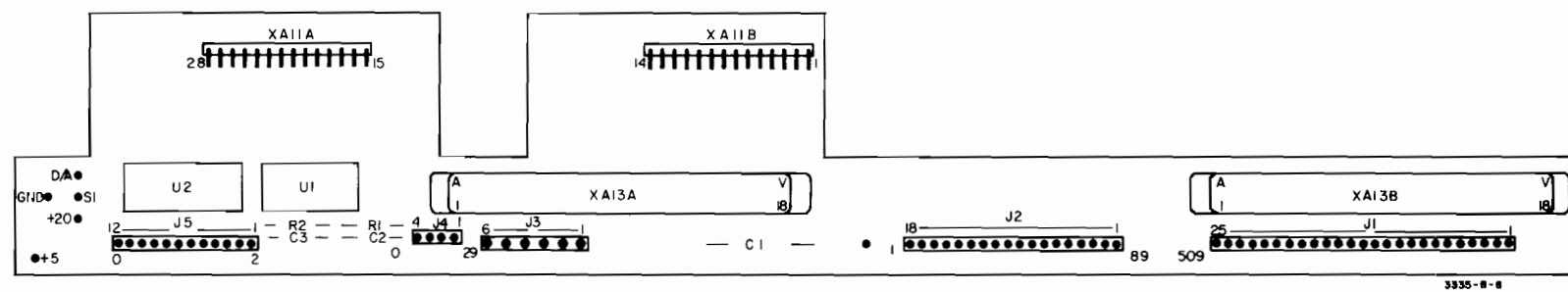
A10 -hp- Part No. 03335-66512
