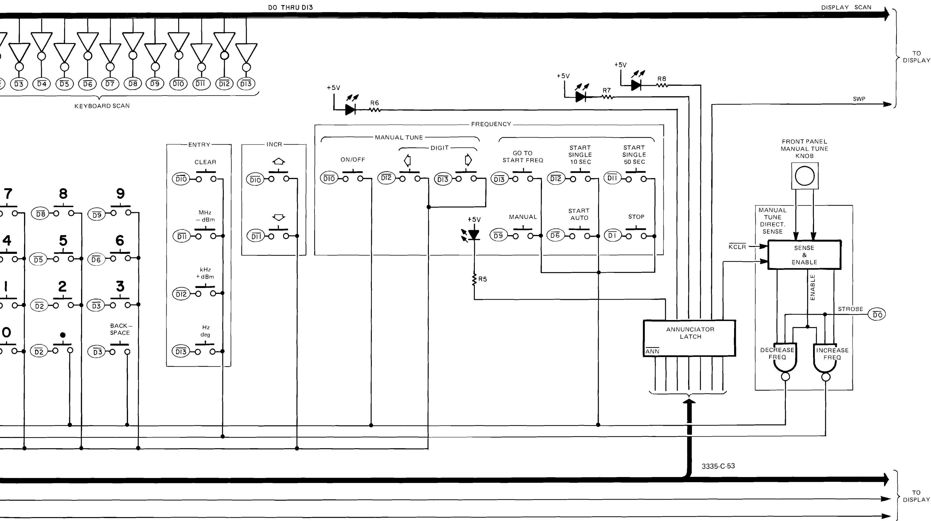
Figure 8-B-2. Block Diagram, Keyboard (03335-66510) A11. 8-B-5/8-B-6
