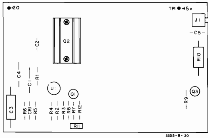
A17 -hp- Part No. 03335-66522
