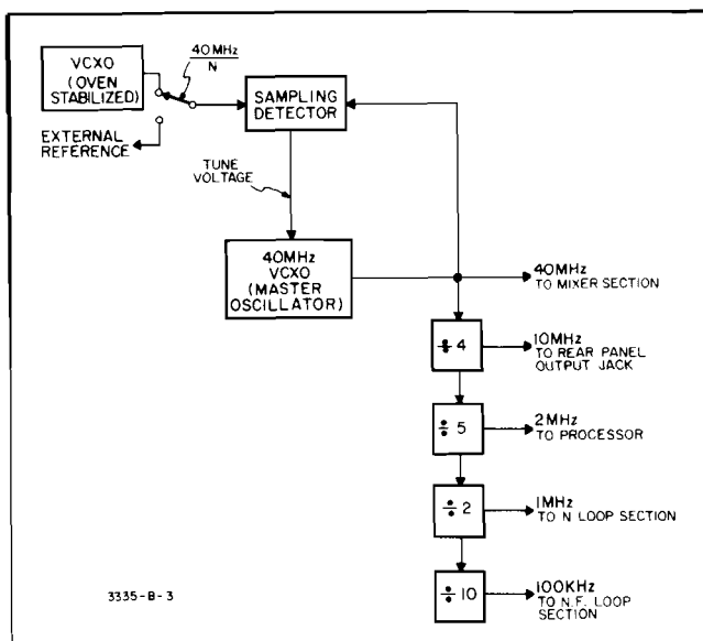
Figure 8-12. Simplified Block Diagram, Reference Section.
