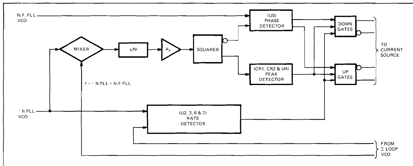
Figure 8-42. Phase Detector Current Source Control.
