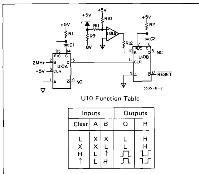
Figure 8-7. Start-Up Circuit.
