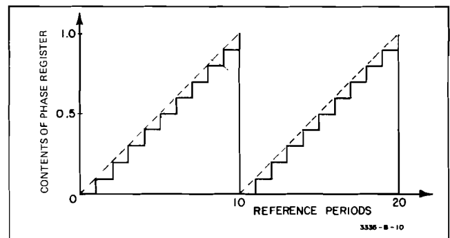
Figure 8-31. Phase Register Contents.
