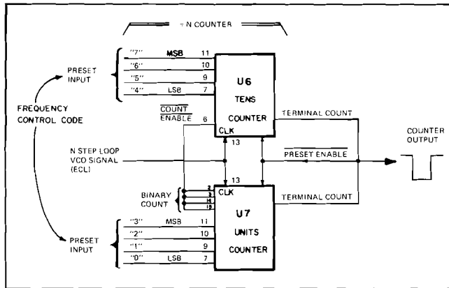
Figure 8-20. ÷N Counter.
