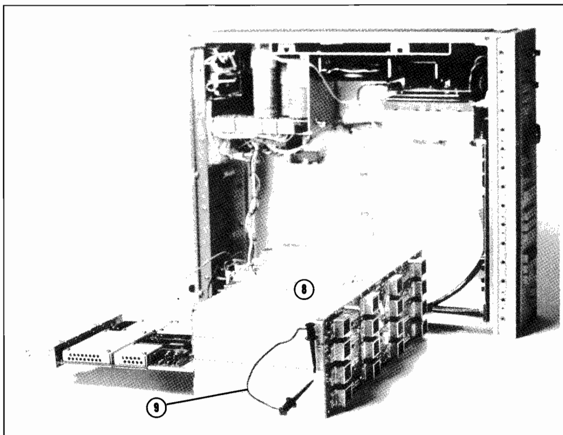
Figure 8-O-5. Module Position.
