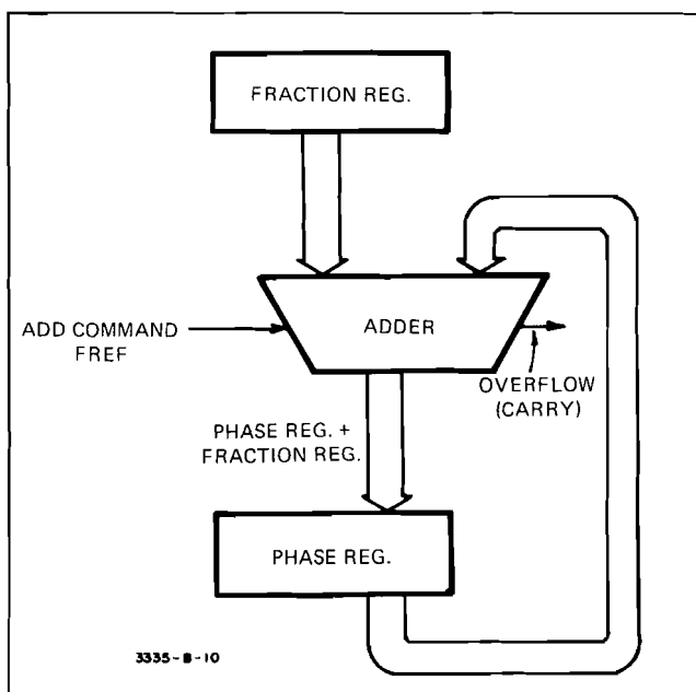
Figure 8-29. Accumulator.
