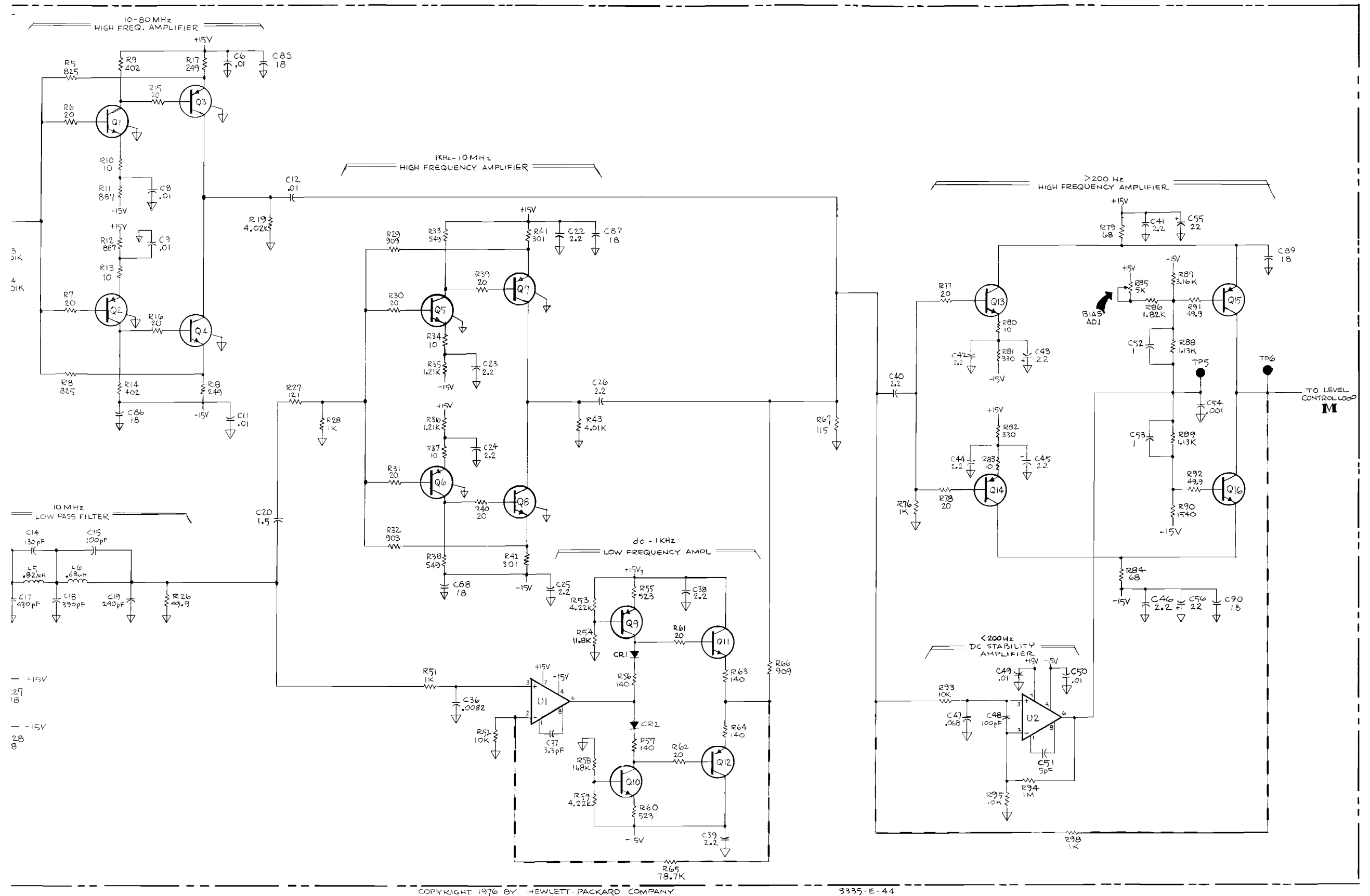
Figure 8-M-1. Schematic Diagram, Output Amplifier (03335-66538) A6. 8-M-9/8-M-10
