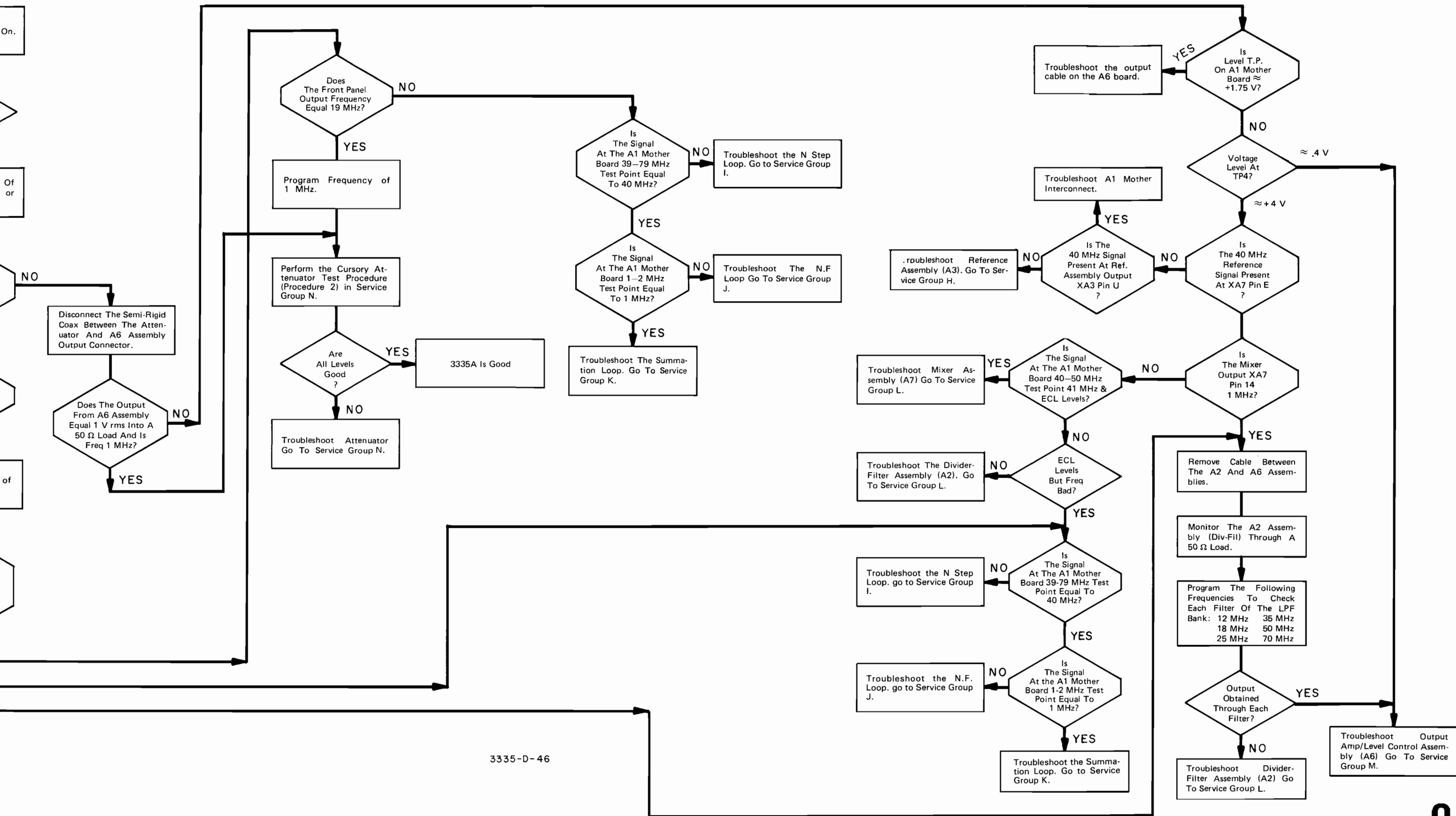
Figure 8-O-1. TS Flowchart, Section Level Troubleshooting. 8-O-5/8-O-6
