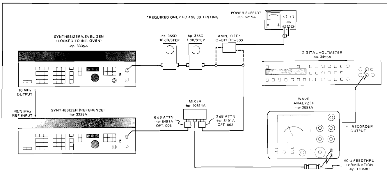
Figure 4-7. Attenuator Verification Test.
