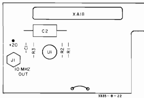
A18 -hp- Part No. 03335-66517
