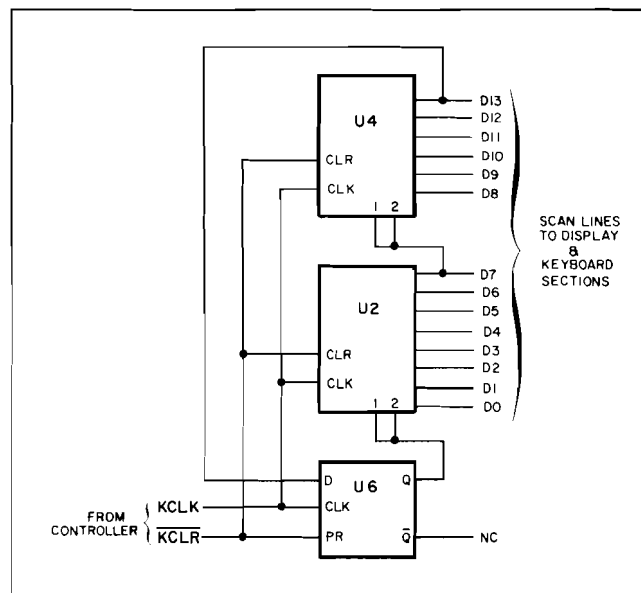
Figure 8-9. Scan Circuit.
