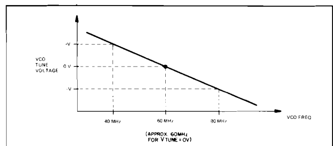
Figure 8-18. VCO Tune Voltage vs. VCO Frequency.
