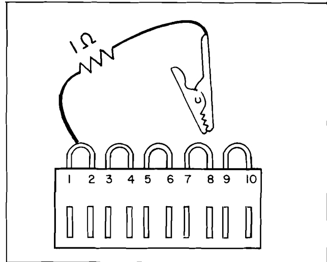
Figure 5-1. Current Limit Test Fixture.
