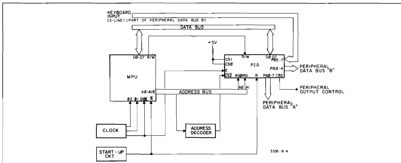
Figure 8-8. MPU and PIA Interconnection.
