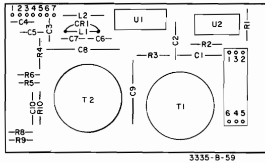
A19 -hp- Part No. 03335-66519
