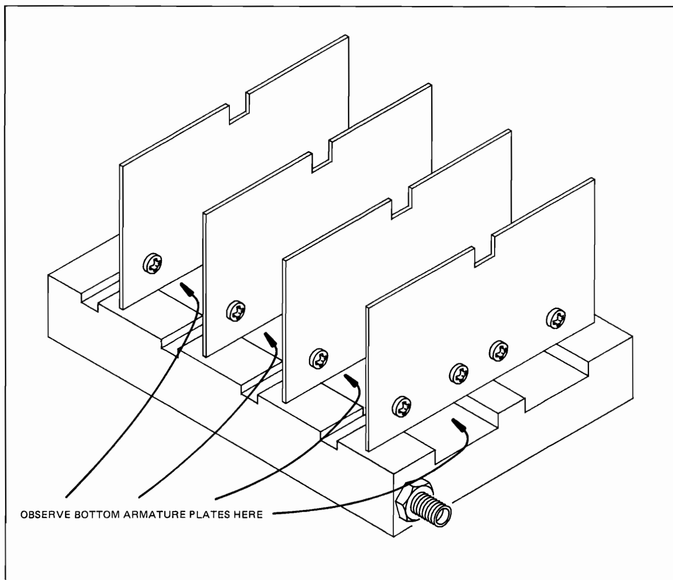
Figure 8-N-6. Bottom Armature Plates.
