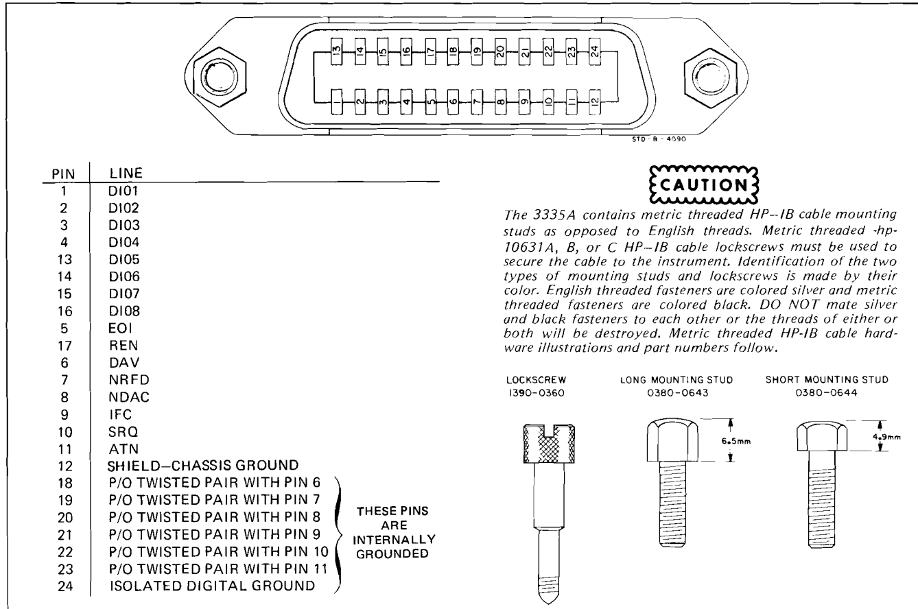
Figure 2-2. HP-IB Connector.
