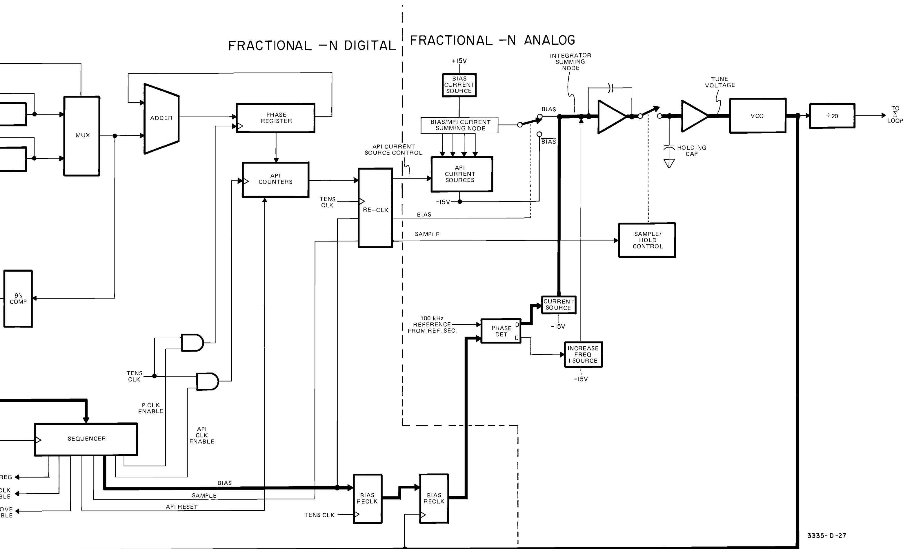
Figure 8-J-5. Block Diagram, Fractional-N Loop (03335-66503, 03335-66504) A4, A5. 8-J-17/8-J-18
