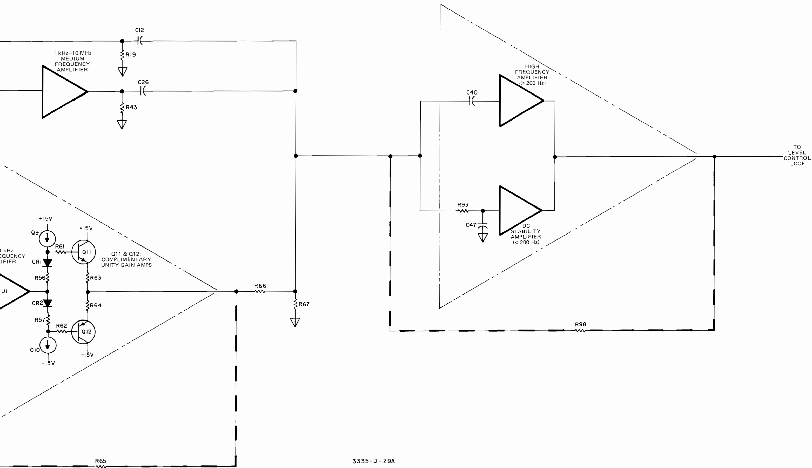
Figure 8-M-3. Block Diagram, Output Amplifier (03335-66538) A6. 8-M-13/8-M-14
