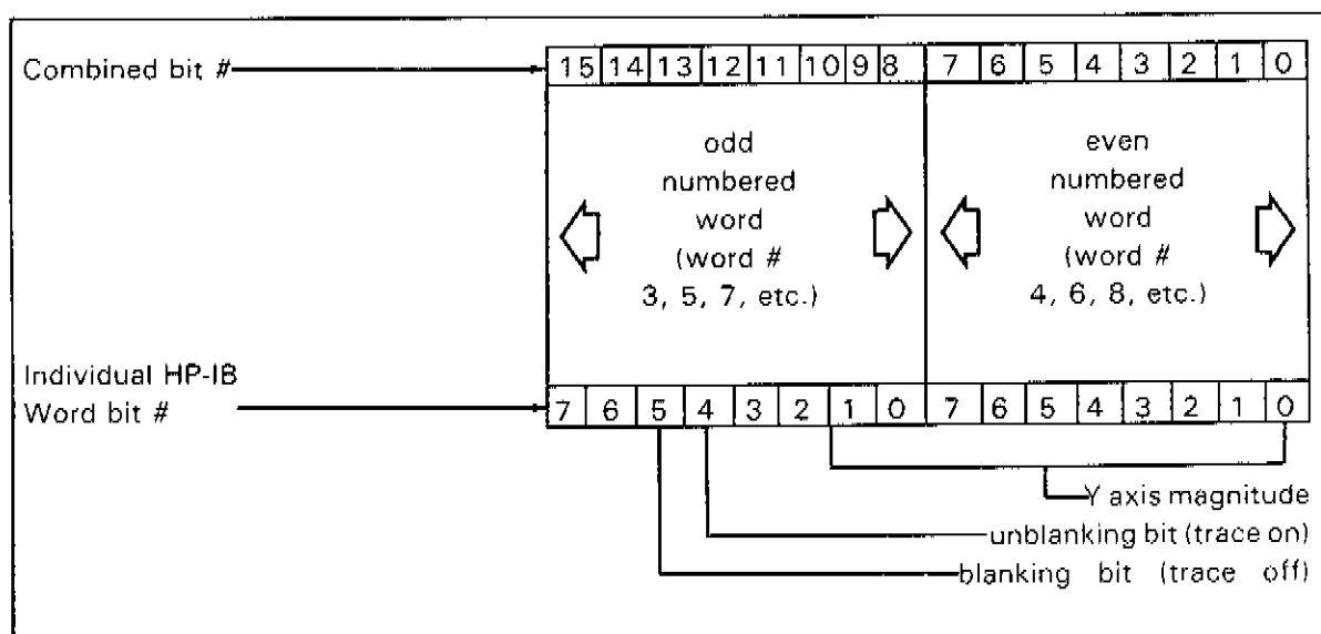
Figure 3-2-3. CRT Trace Word In Binary Mode.
