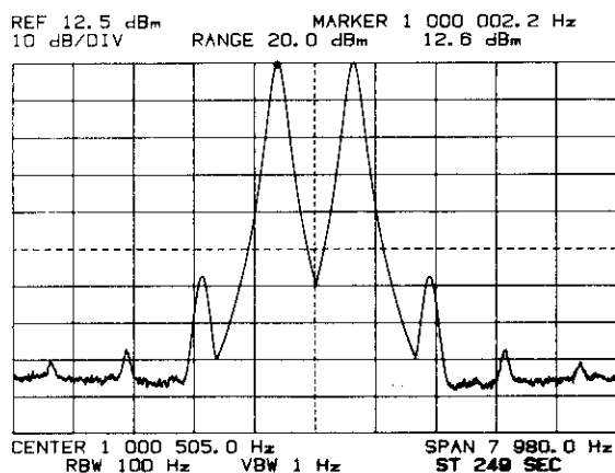
Driving Signals and Odd-Order IM Distortion Products.
