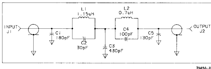
Figure 4-19. 9 MHz Low Pass Filter.
