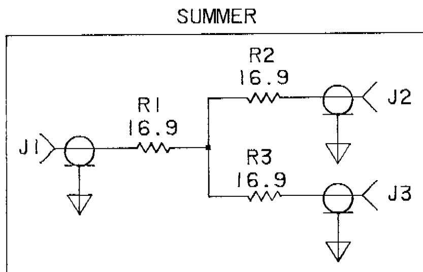
Figure 4-22. Frequency Summer.
