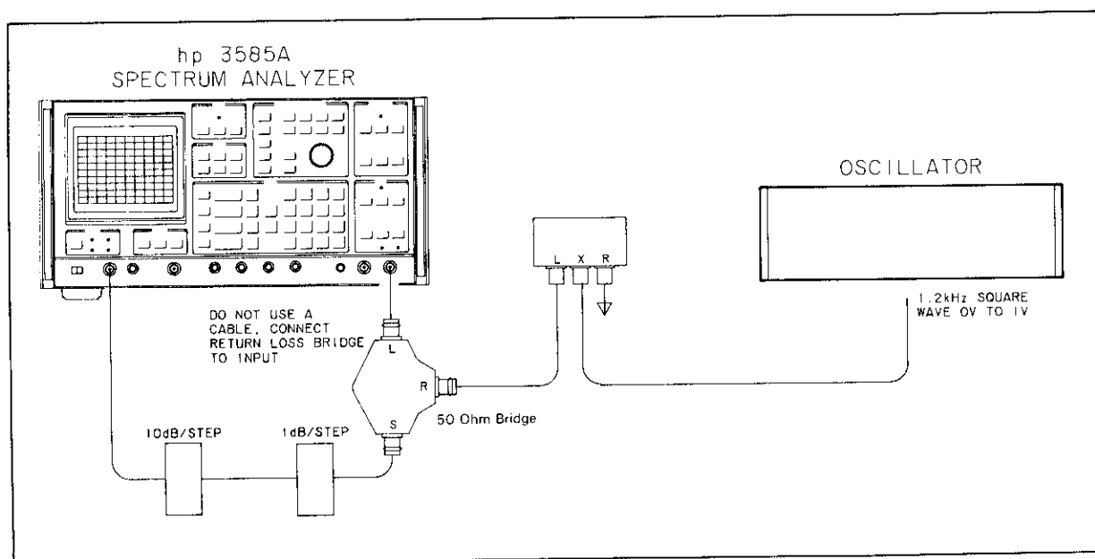
Figure 4-10. 50 ohm Return Loss Test (Automatic Tests).
