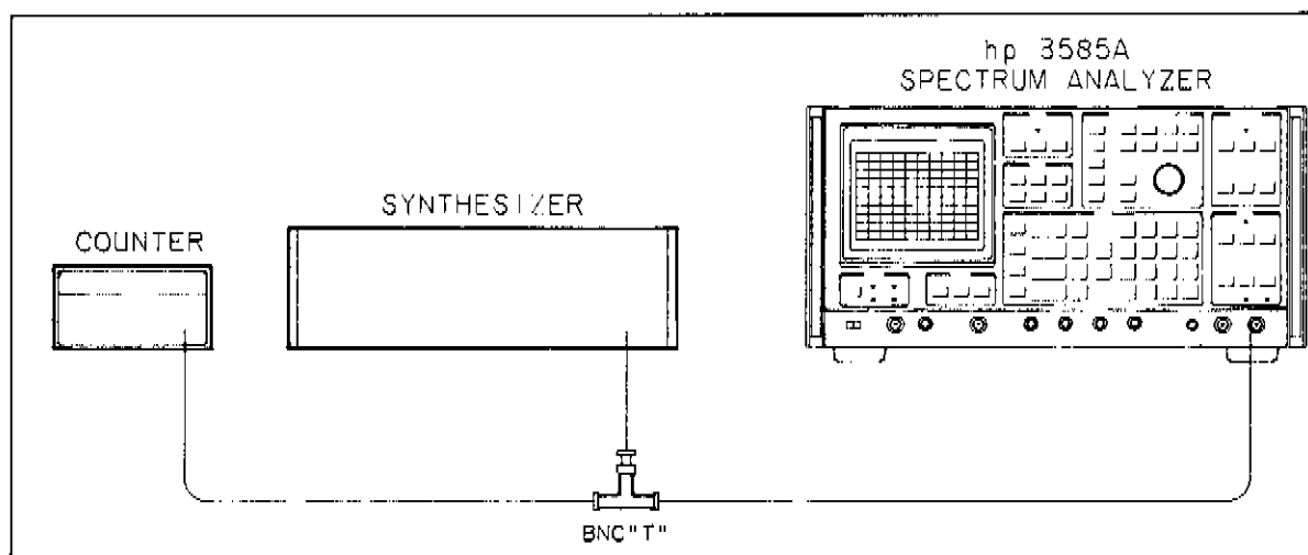
Figure 4-1. Frequency Accuracy Test
