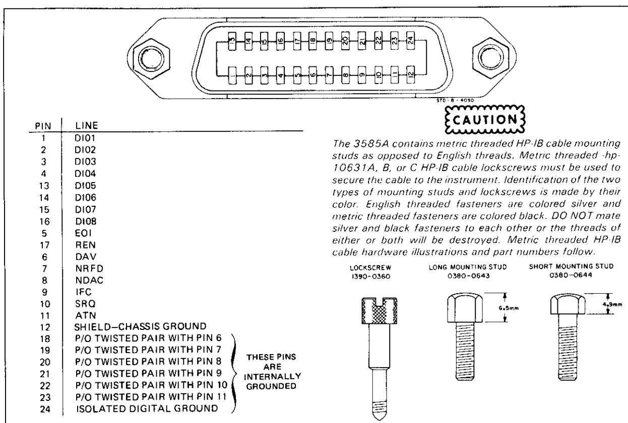
Figure 2-5. HP-IB Connector.
