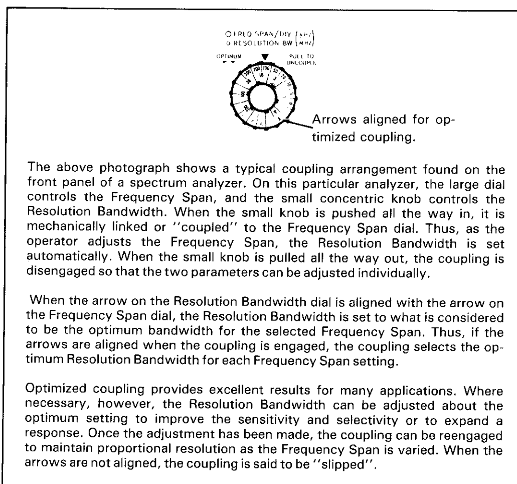
Figure 1. Mechanical Coupling.
