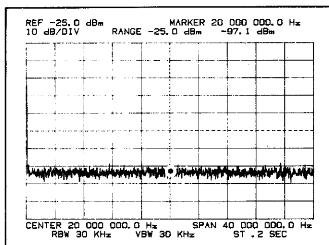
Figure 2-4. Turn-On Display.
