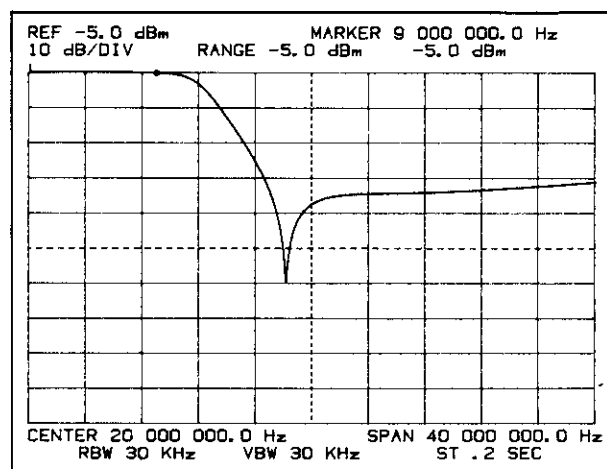
Figure 4-20. Approximate Filter Response.
