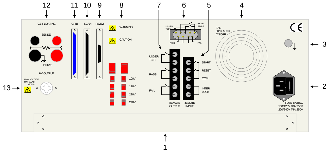
Figure 1-3: G6000 Plus Rear Panel Controls and Connectors
