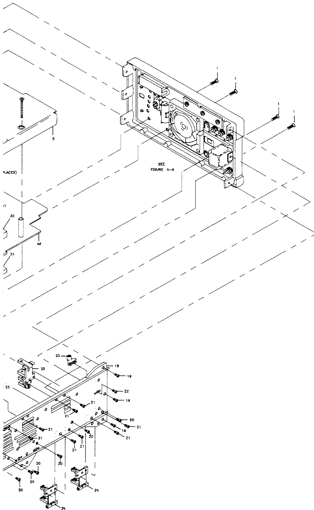
FIGURE 4-3. PARTS IDENTIFICATION, MAIN CHASSIS
