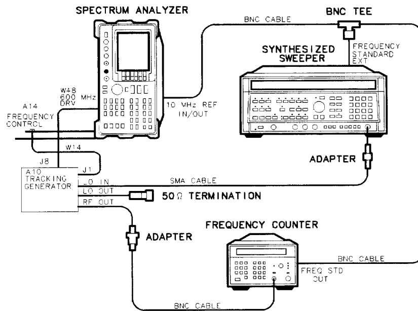
Figure 2-25. Tracking Oscillator Adjustment Setup
