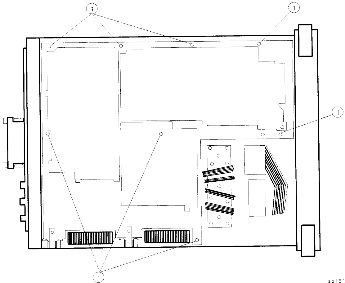
Figure 3-19. A14 and A15 Assembly Removal
