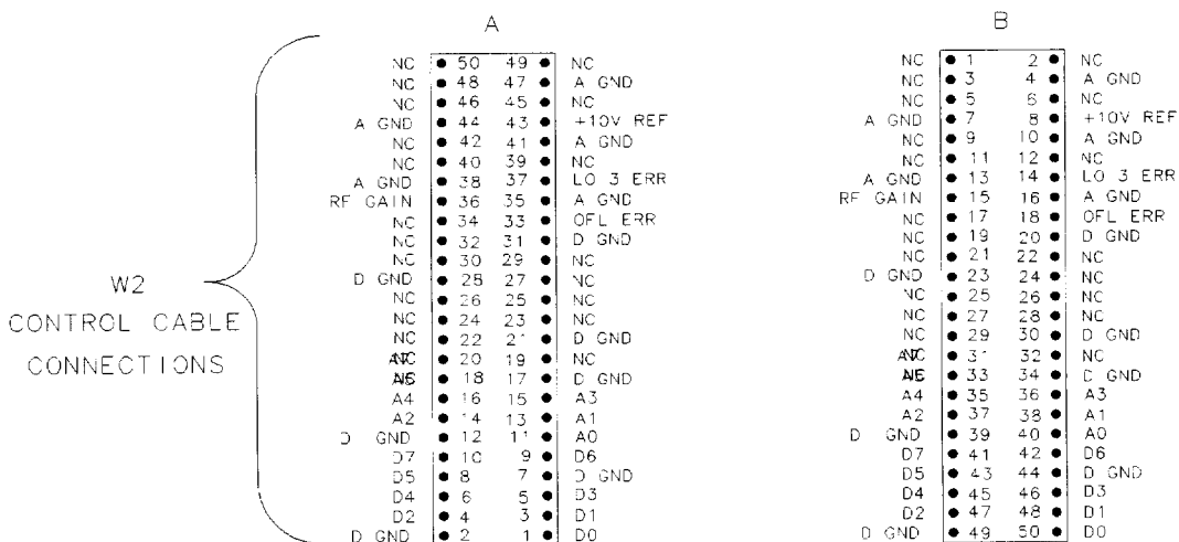
Figure 6-2. Ribbon Cable Connections
