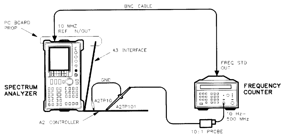
Figure 2-26. 16 MHz PLL Adjustment Setup
