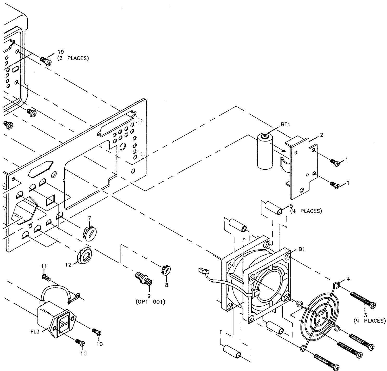
Figure 4-6. Parts Identification, Rear Frame
