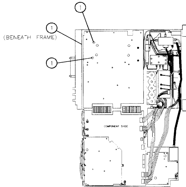
Figure 3-29. A21 OCXO Mounting Screws
