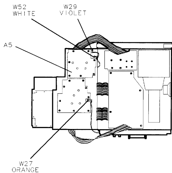
Figure 3-8. Assembly Cables (2 of 2)
