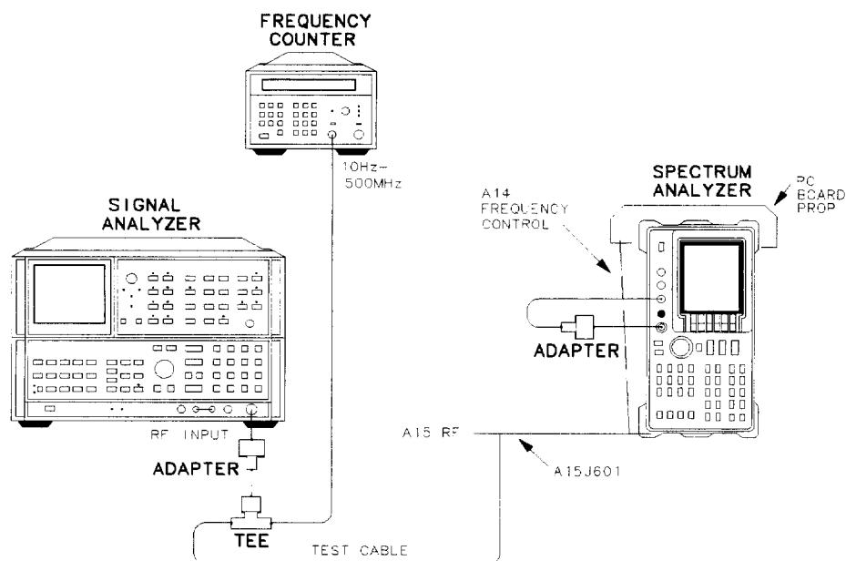
Figure 2-22. Signal ID Oscillator Adjustment Setup
