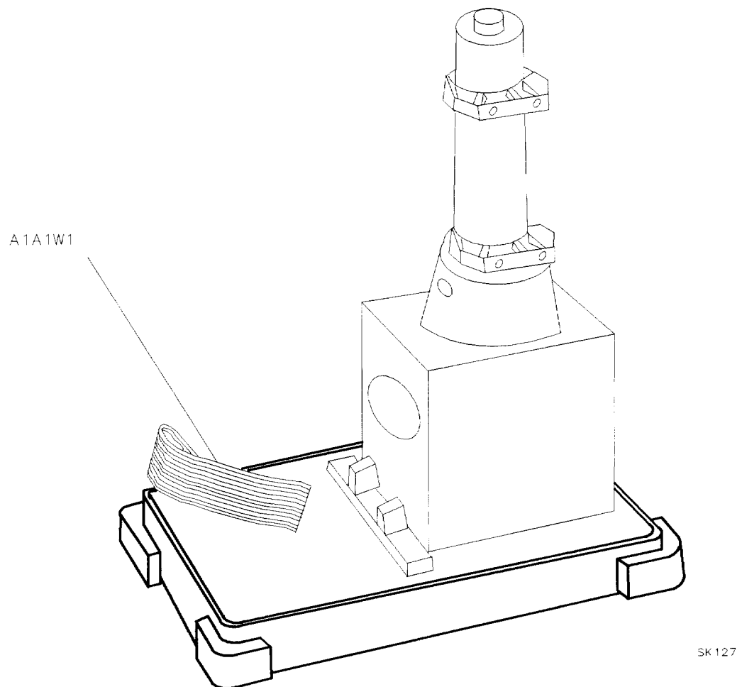
Figure 3-6. Placing the CRT into the Front Frame
