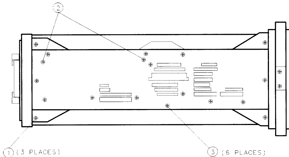
Figure 3-28. Side Frame Mounting Screws
