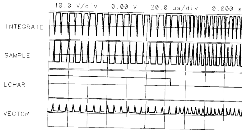
Figure 9-5. Switch Driver Waveform LCHAR
