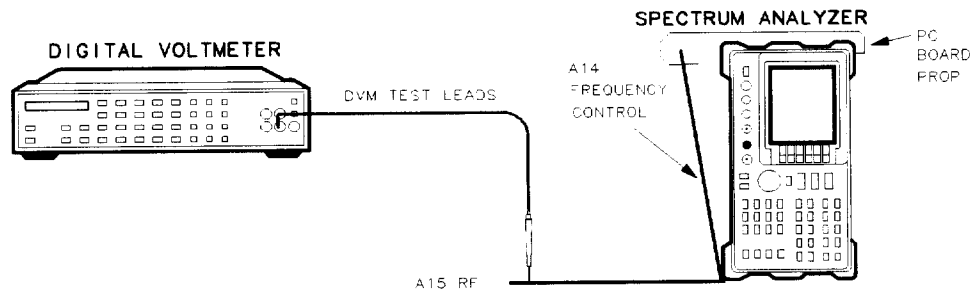
Figure 2-8. Sampler Adjustment Setup
