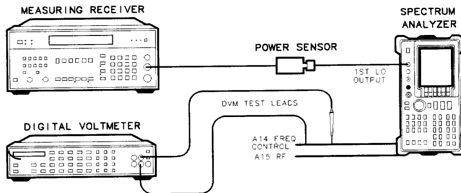
Figure 2-12. First LO Distribution Amplifier Adjustment Setup
