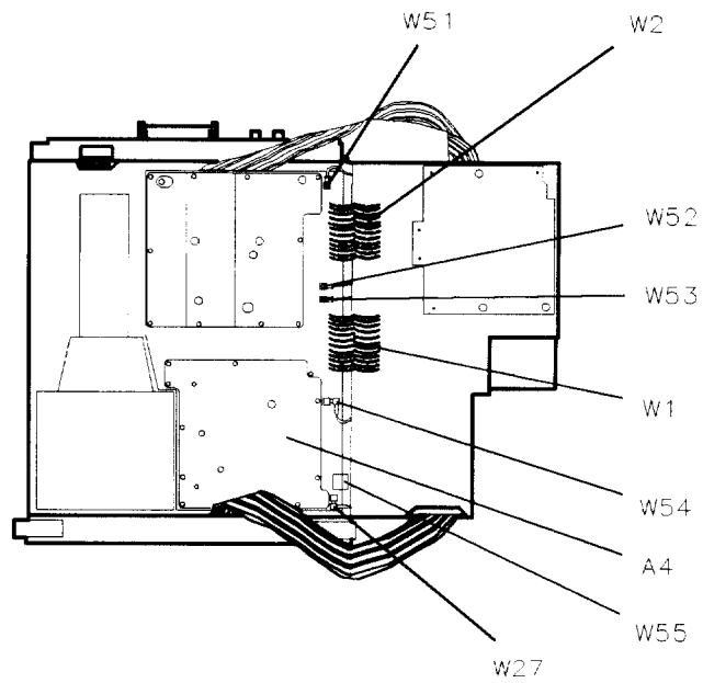
Figure 5-3. Top View (A2 and A3 Unfolded)
