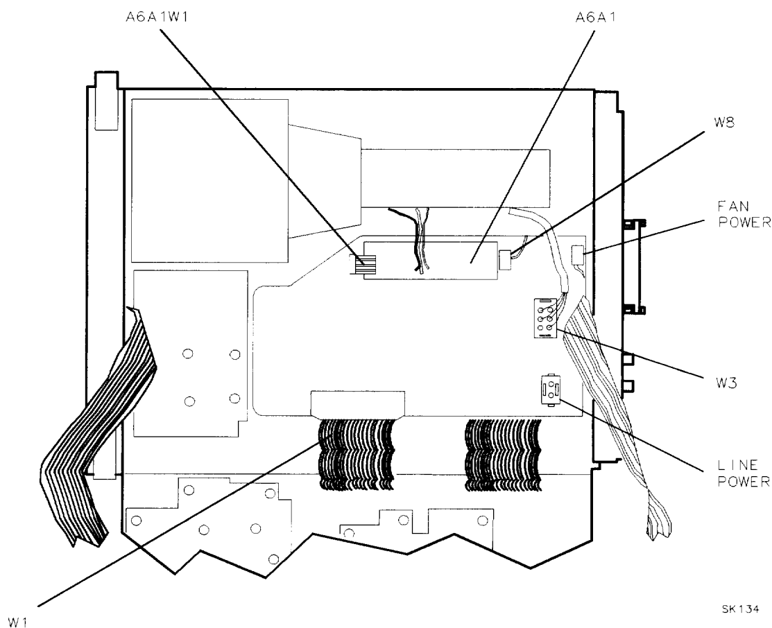
Figure 3-11. A6 Power Supply Connections
