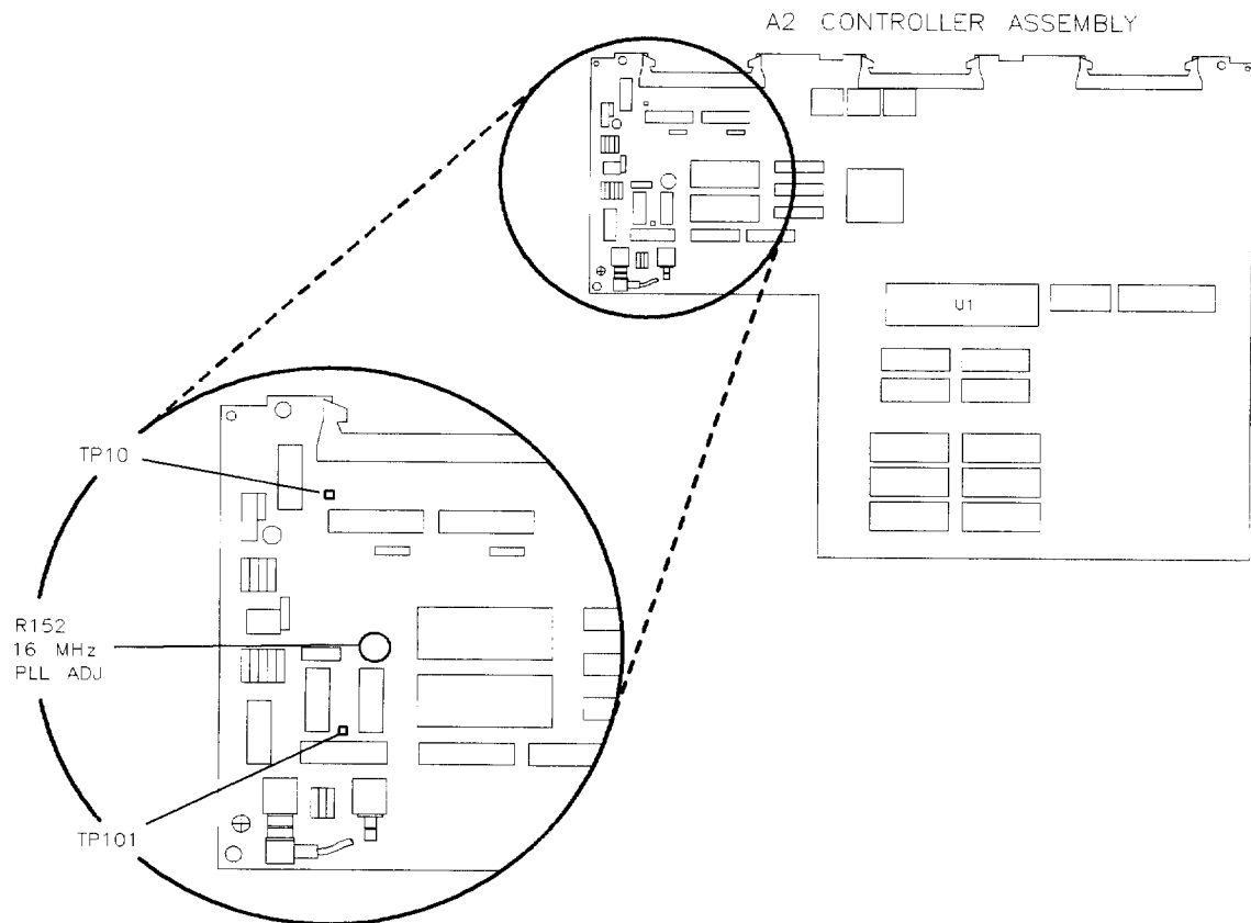
Figure 2-27. 16 MHz PLL Adjustment Location
