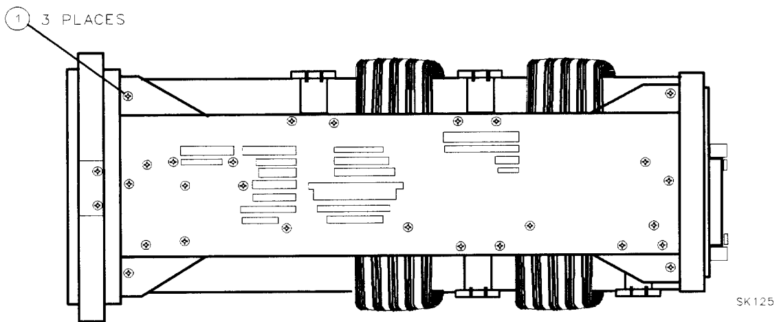
Figure 3-4. Front-Frame Mounting Screws
