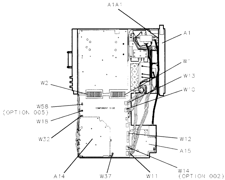
Figure 5-6. Bottom View (A15 and A14 Unfolded)
