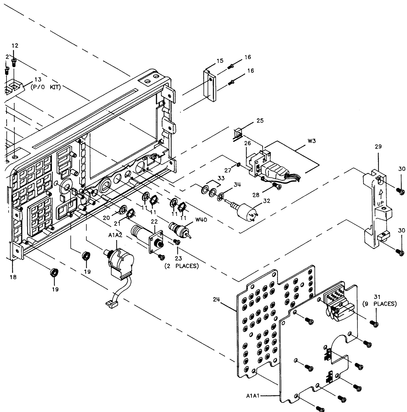
Figure 4-5. Parts Identification, Front Frame
