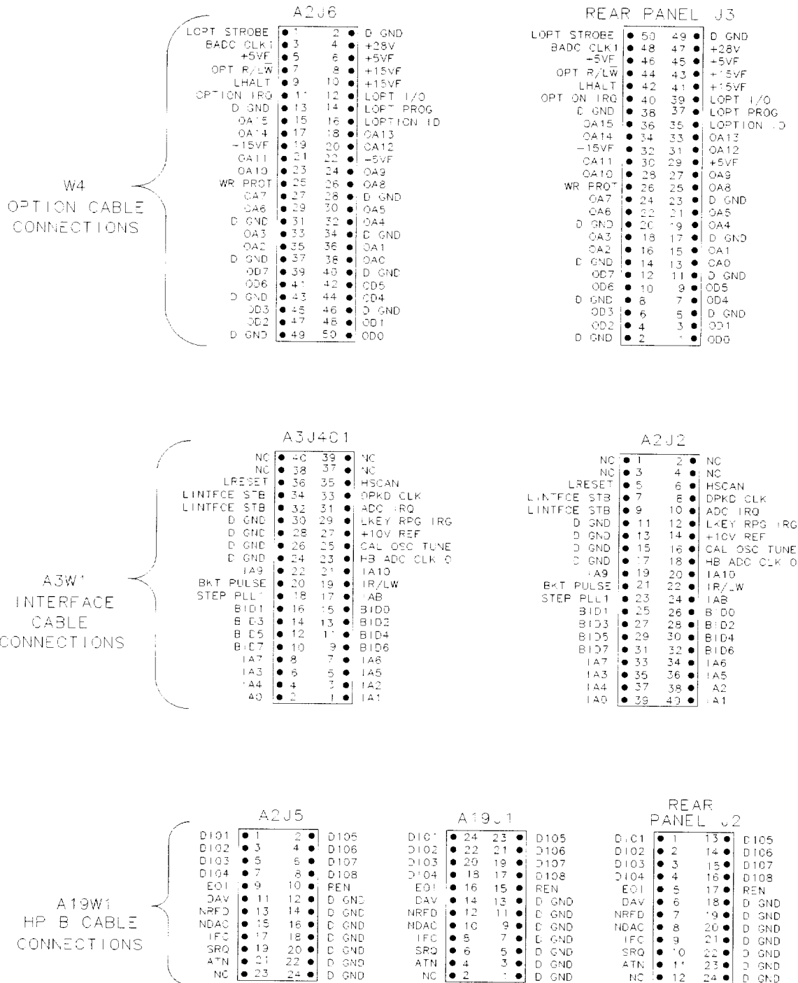
Figure 6-2. Ribbon Cable Connections (2 of 2)
