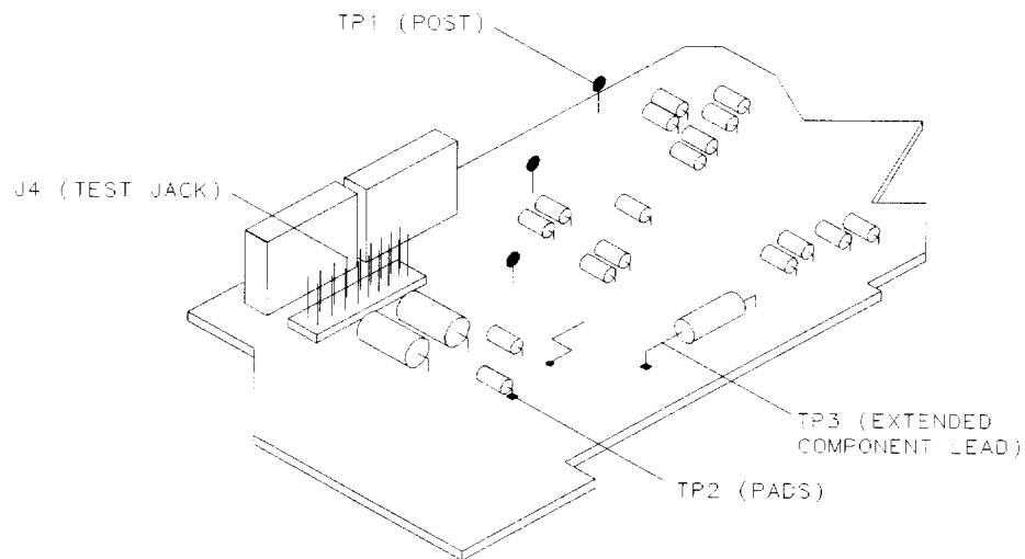
Figure 6-1. Assembly Test Points
