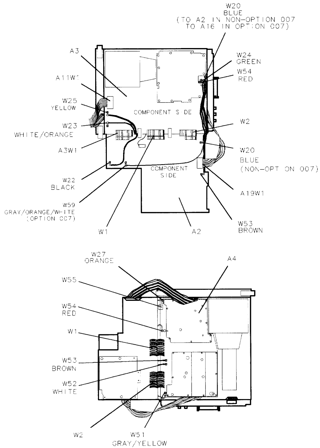
Figure 3-8. Assembly Cables
