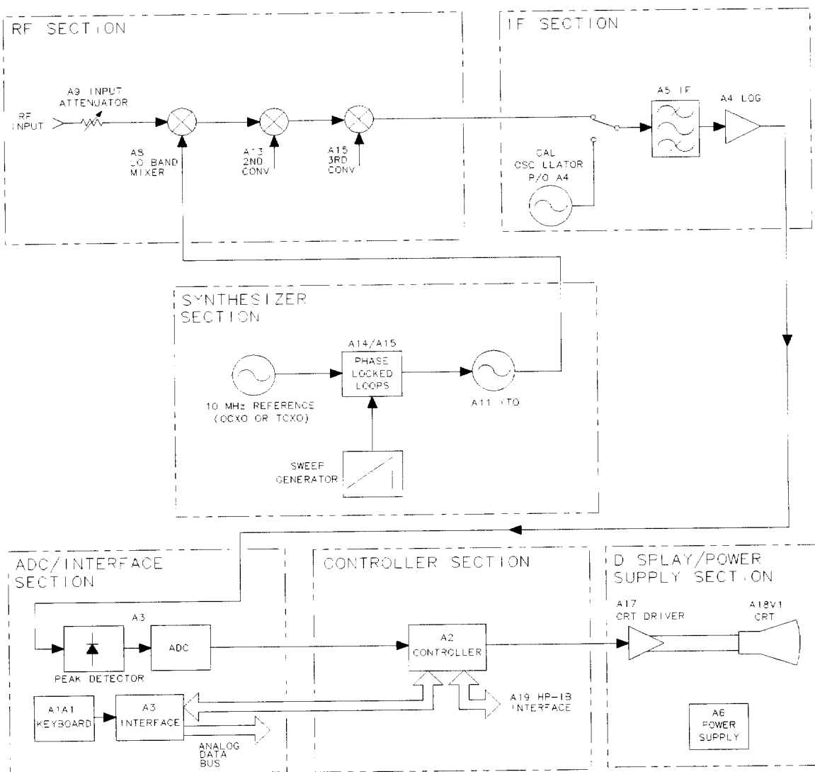
Figure 6-4. Functional Sections
