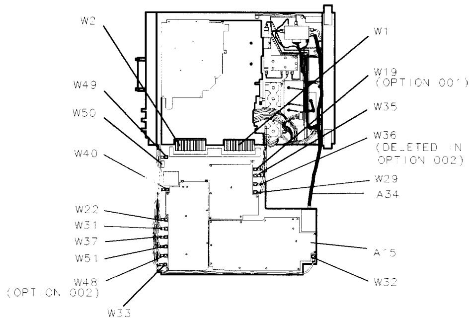
Figure 5-5. Bottom View (A15 Unfolded)
