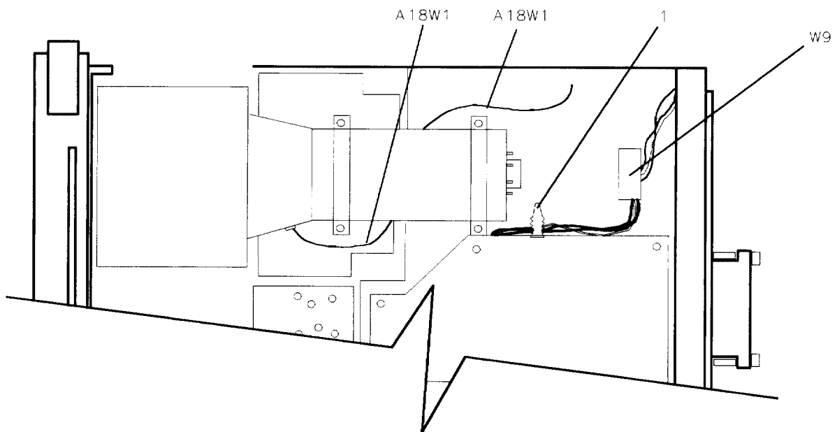
Figure 3-5. Installing the CRT and Front-Frame Assemblies
