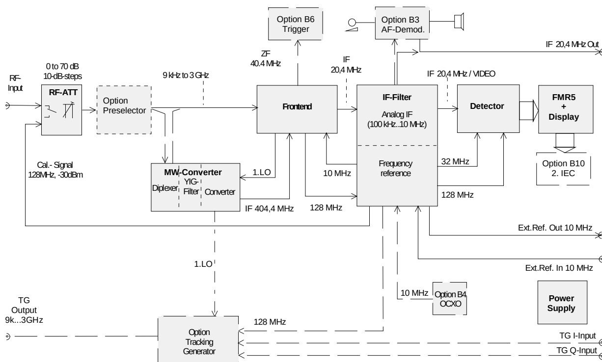
Fig. 3-1 Block diagram
