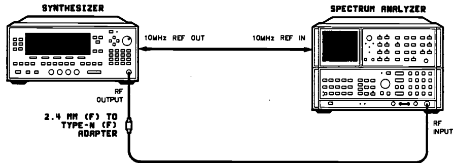
Figure 2-14. Alternate Phase Noise Test Setup
