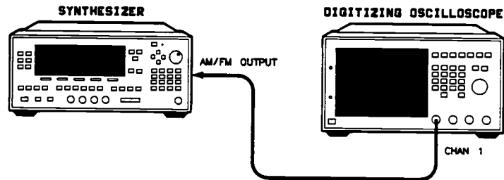
Figure 3-44. Modulation Generator Flatness Adjustment Setup
