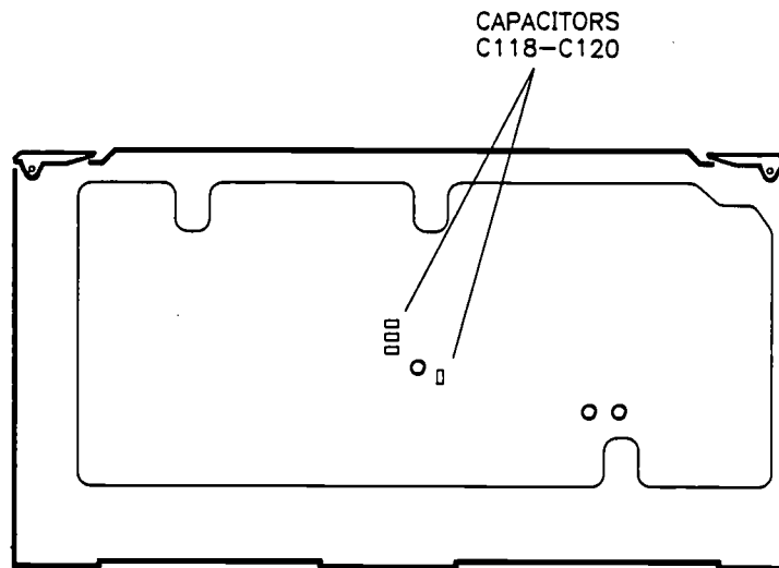
Figure 3-10. Capacitor Locations
