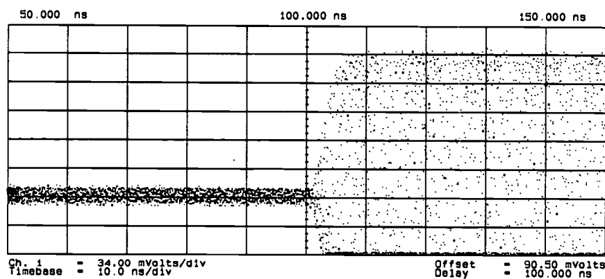
Figure 2-17. Signal Level between RF Power Off and On
