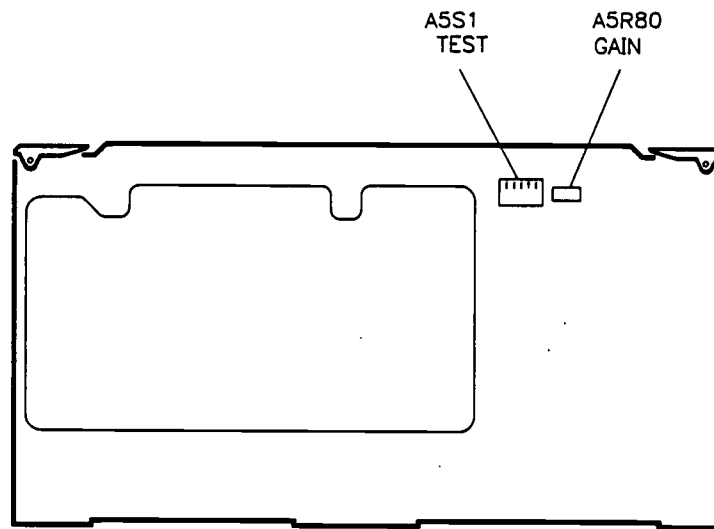
Figure 3-14. Switch and Adjustment Locations
