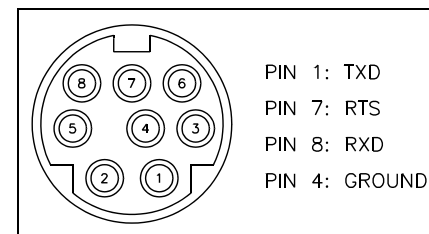
Figure 12. COMM Jack Pinout for RS-232 Communication
