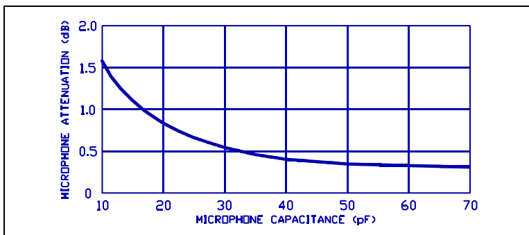
Figure 21. Microphone Output Attenuation Caused by Input Capacitance of Preamp
