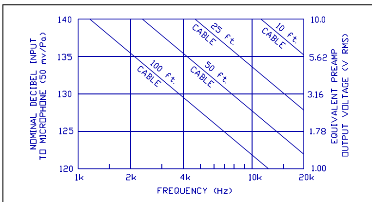
Figure 22. Frequency/Amplitude Limitations with Extension Cables
