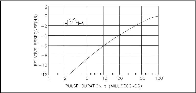
Figure 28. IMPULSE Response
