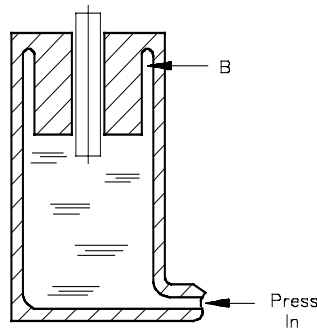
FIGURE 2-2 RE-ENTRANT CYLINDER
