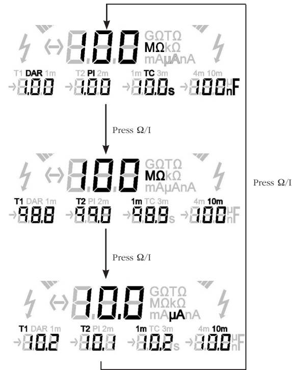
Figure 1 - The result of an insulation resistance test (IR) Test settings: T1 and T2 times set in order to measure the DAR Test conditions: test runs for longer than 10 minutes as this is required for a PI reading.
