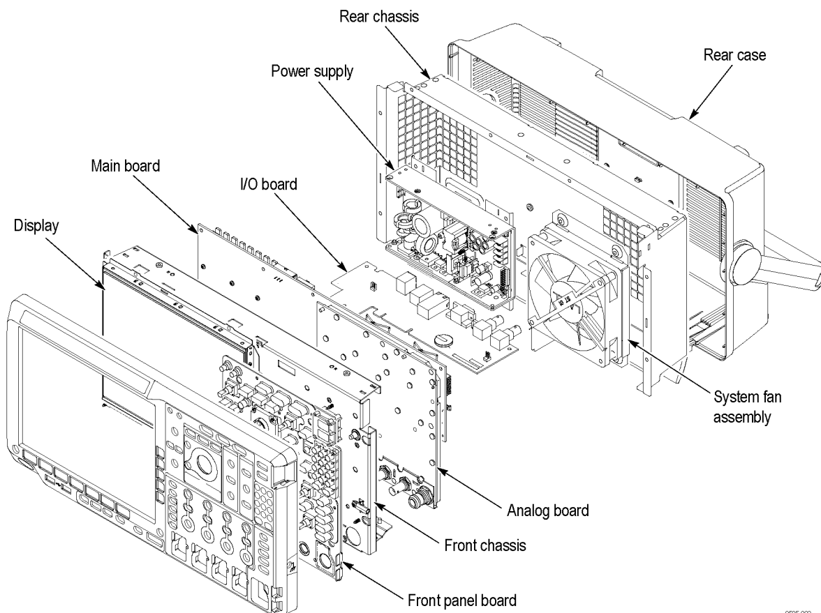
Figure 3: Module locator
