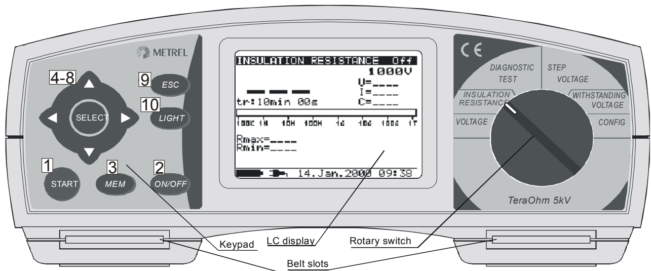
Fig. 1. Front panel
