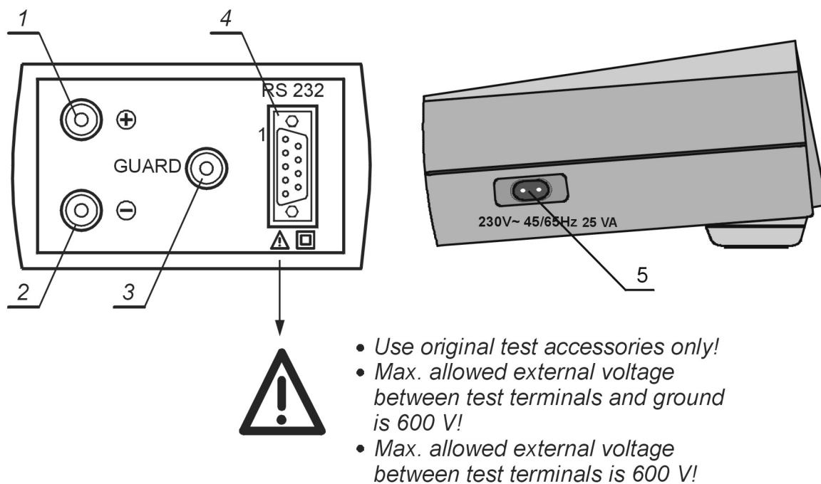
Fig. 2. Connectors
