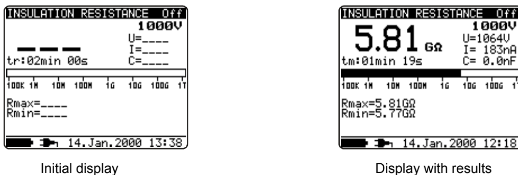
Fig. 9. Insulation Resistance function display states
