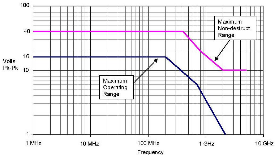
Figure 1, Input Voltage vs. Frequency
