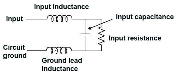
Figure 3 Probe Input Equivalent Circuit
