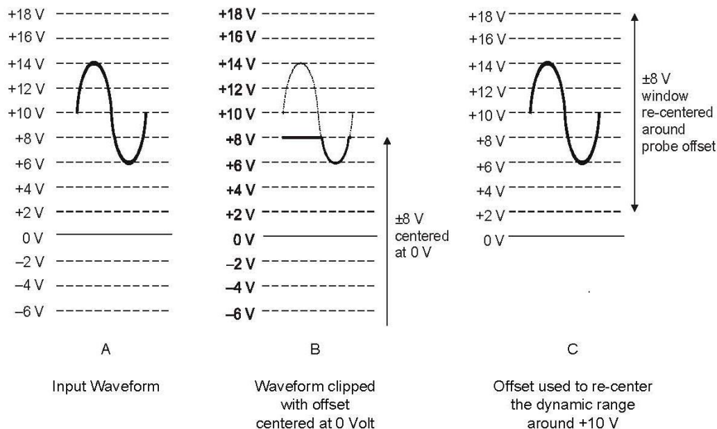
Figure 2, Dynamic Range and Offset Effects
