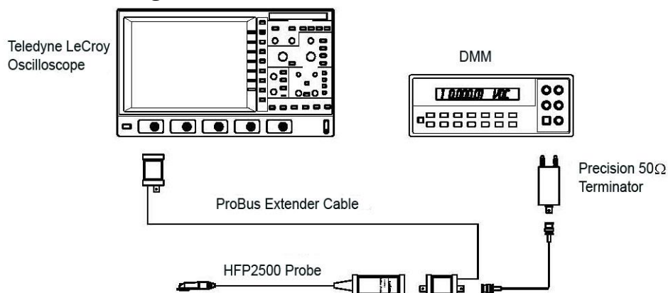
Figure 5, Output Zero Voltage Test Setup
