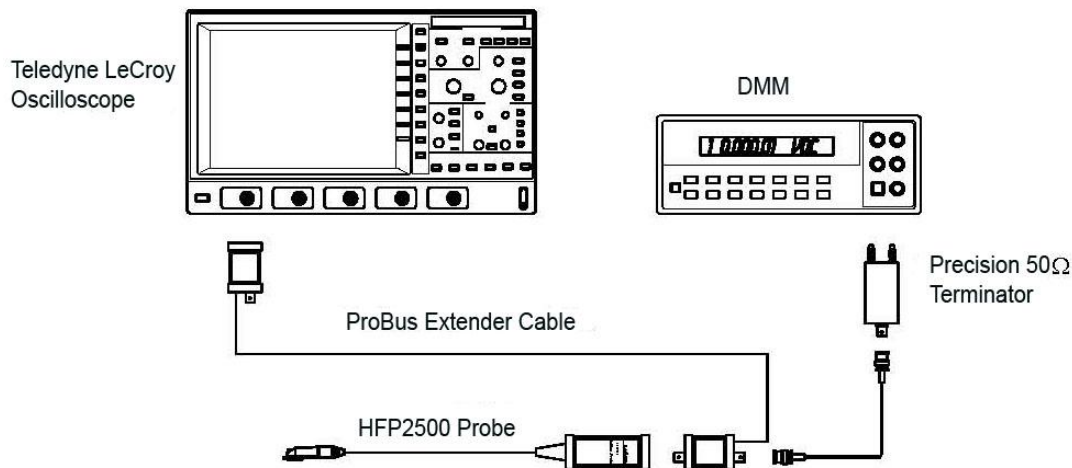
Figure 7 Output Zero Voltage Adjustment Setup
