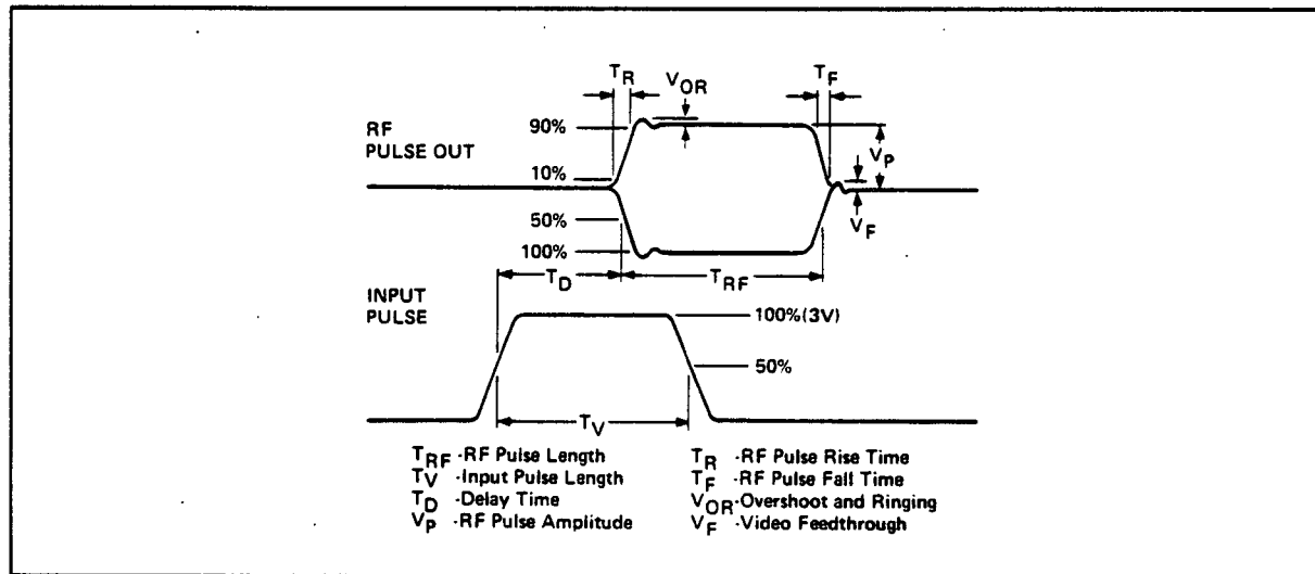
Figure 4-12. Pulse Definitions
