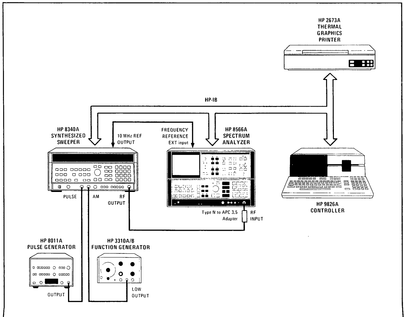
Figure 4. Modulation Setup
