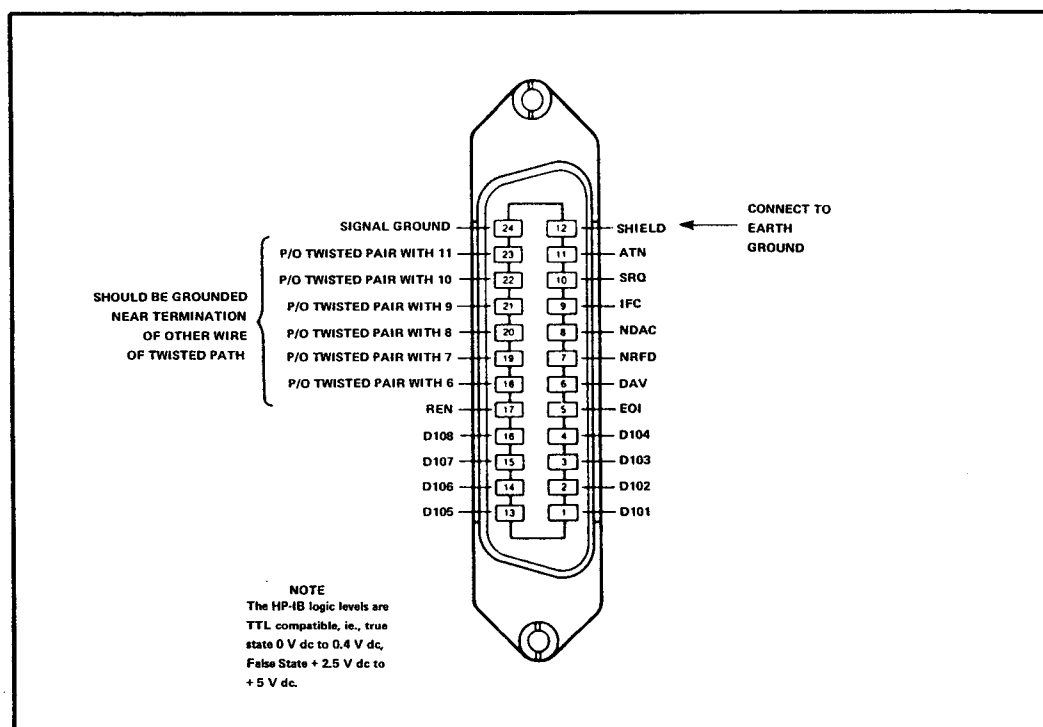
Figure 3-25. HP-IB Pin-Out
