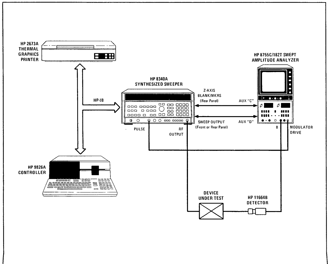
Figure 2. Equipment Setup
