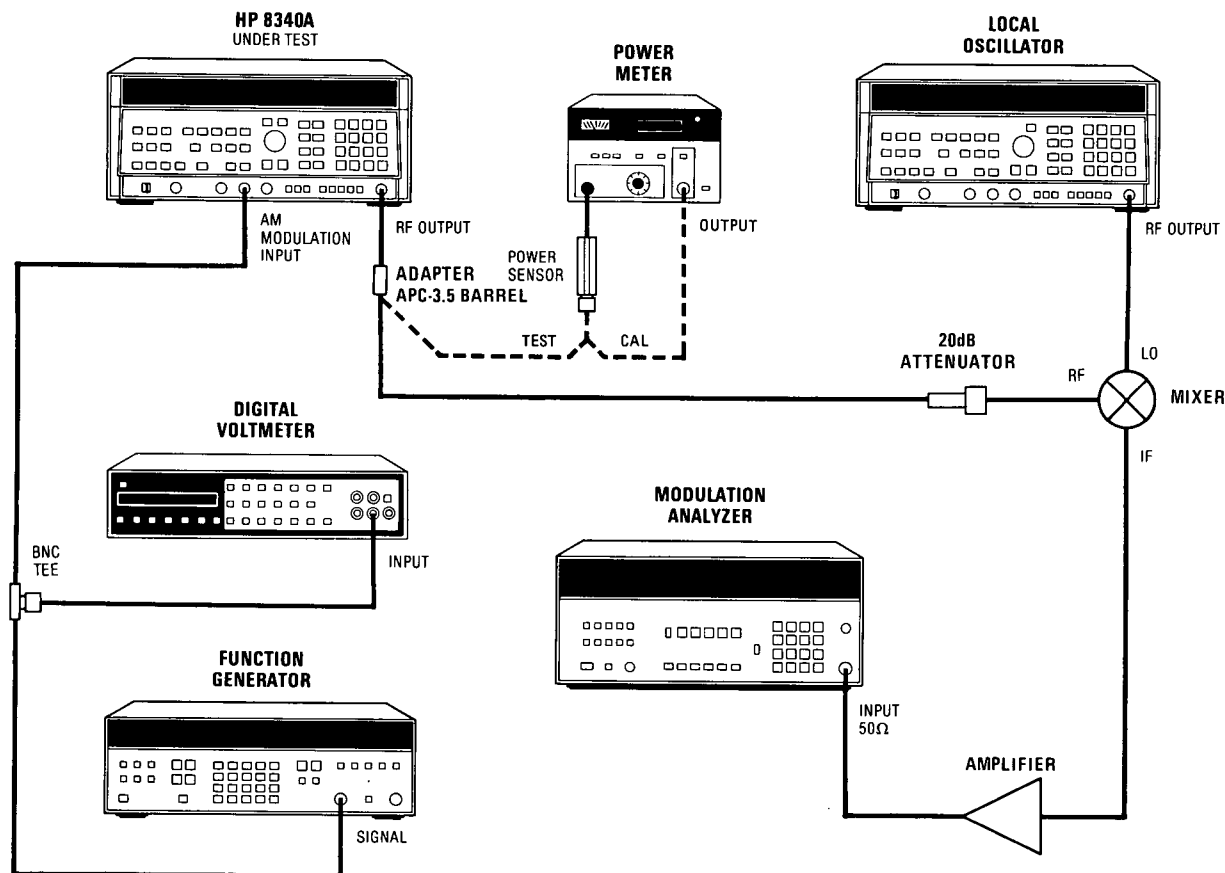
Figure 4-19. Amplitude Modulation Test Setup
