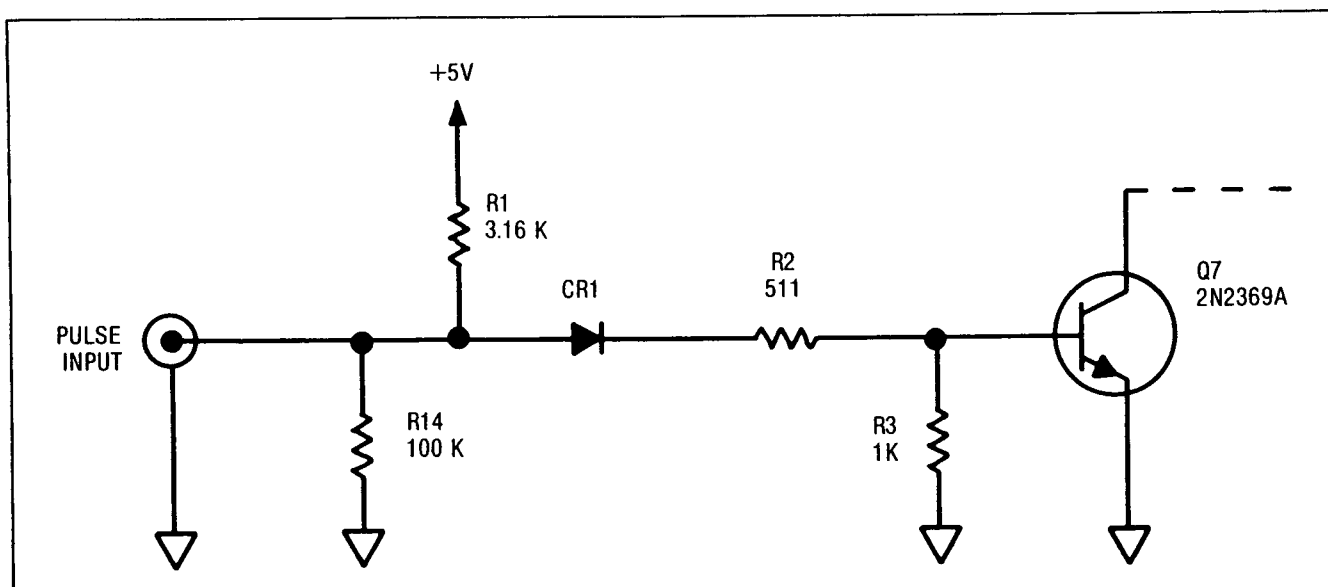
Figure 8-36. Pulse Input Circuit
