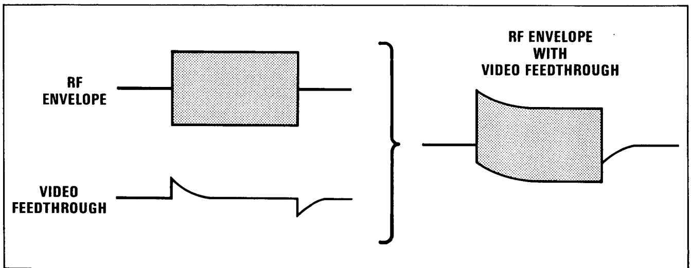
Figure 3-37. Video Feedthrough
