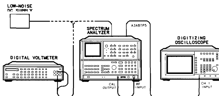
Figure 3-100. Analog-To-Digital Converter Adjustments Setup
