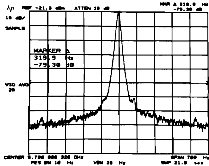
Figure 2-23. Noise Sidebands Measurement
