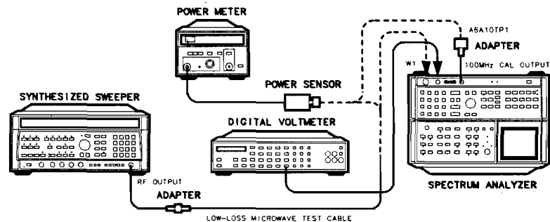
Figure 3-89. Frequency Response Preliminary Adjustments Setup
