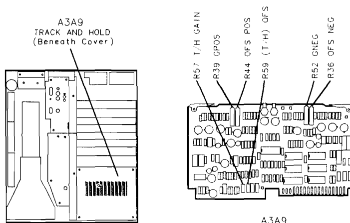
Figure 3-103. Location of Track and Hold Adjustments
