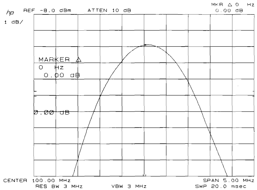
Figure 4-6. Bandwidth Switching Uncertainty Measurement
