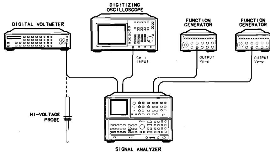
Figure 3-5. High Voltage Adjustment Setup
