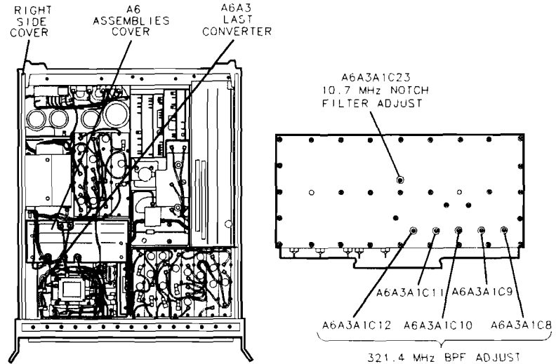
Figure 3-88. Location of Last Converter Adjustments
