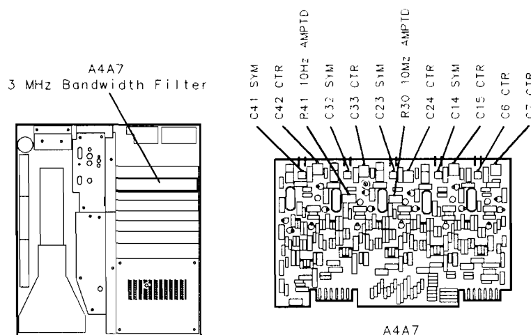
Figure 3-38. Location of Center, Symmetry, and 10 Hz Amplitude Adjustments
