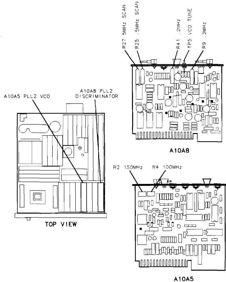
Figure 3-79. Location of PLL2 Adjustments
