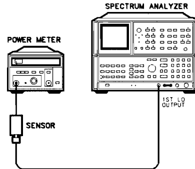
Figure 2-33. 1st LO Output Amplitude Test Setup
