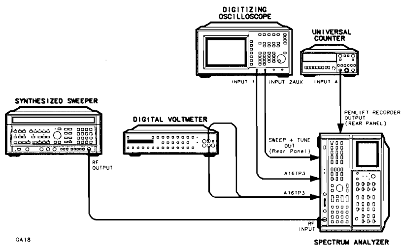
Figure 3-56. Sweep and DAC Adjustments Setup
