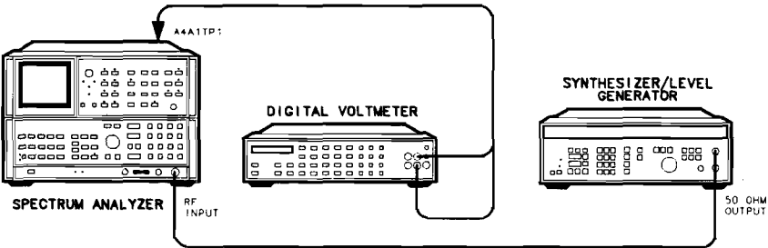
Figure 3-33. Log Amplifier Adjustments Setup
