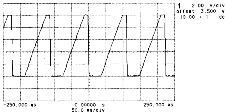
Figure 3-57. 0V to +10V Sweep Ramp at A16TP3
