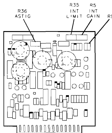
Figure 3-8. Location of A1A2 Components
