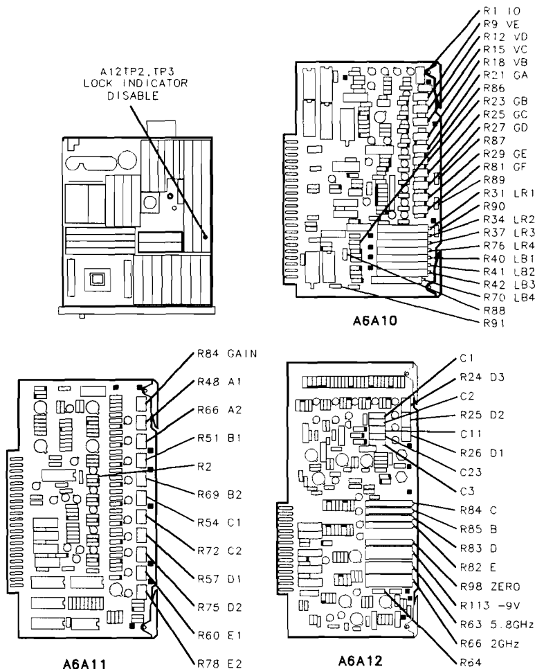
Figure 3-90. Location of Frequency Response Adjustments
