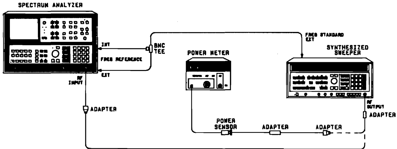
Figure 2-32. Gain Compression Test Setup
