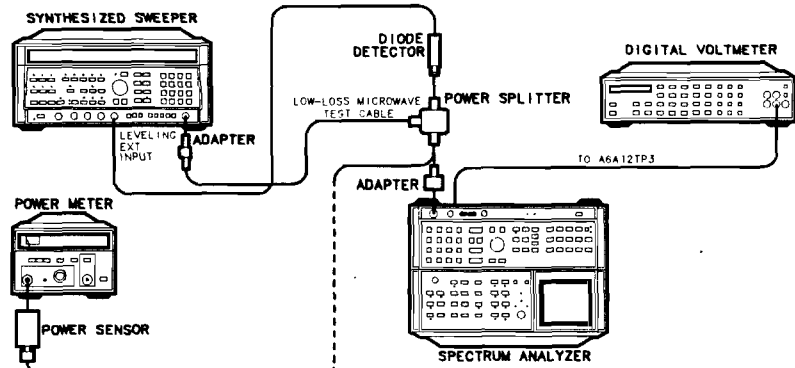
Figure 3-94. Frequency Response Adjustments Setup (2.0 GHz to 22.0 GHz)
