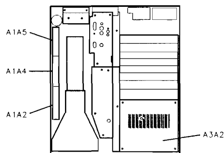
Figure 3-17. Location of A1A2, A1A4, A1A5, and A3A2
