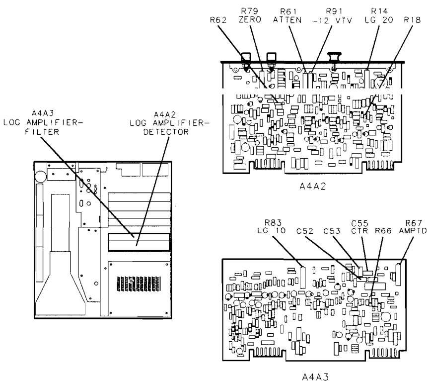
Figure 3-34. Location of Log Amplifier Adjustments
