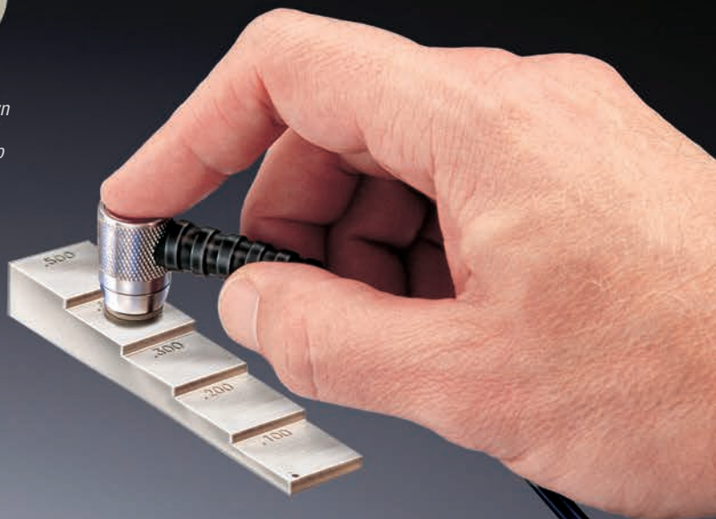
UTG M Thru-Paint models measure the metal thickness of a painted structure without having to remove the coating.
