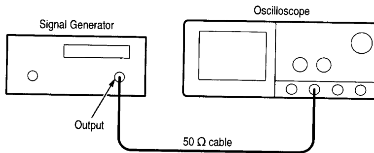
Figure 1–32: 60 Hz Rejection test hookup
