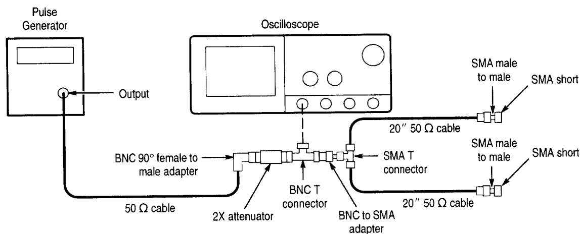
Figure 1-14: Delta time accuracy test hookup
