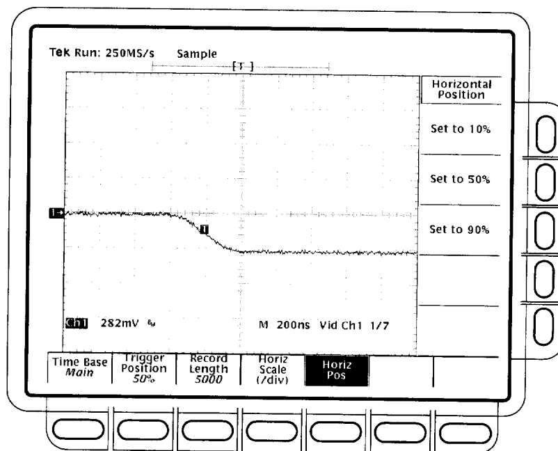
Figure 1-37: Line count accuracy test setup waveform – TDS 684C shown
