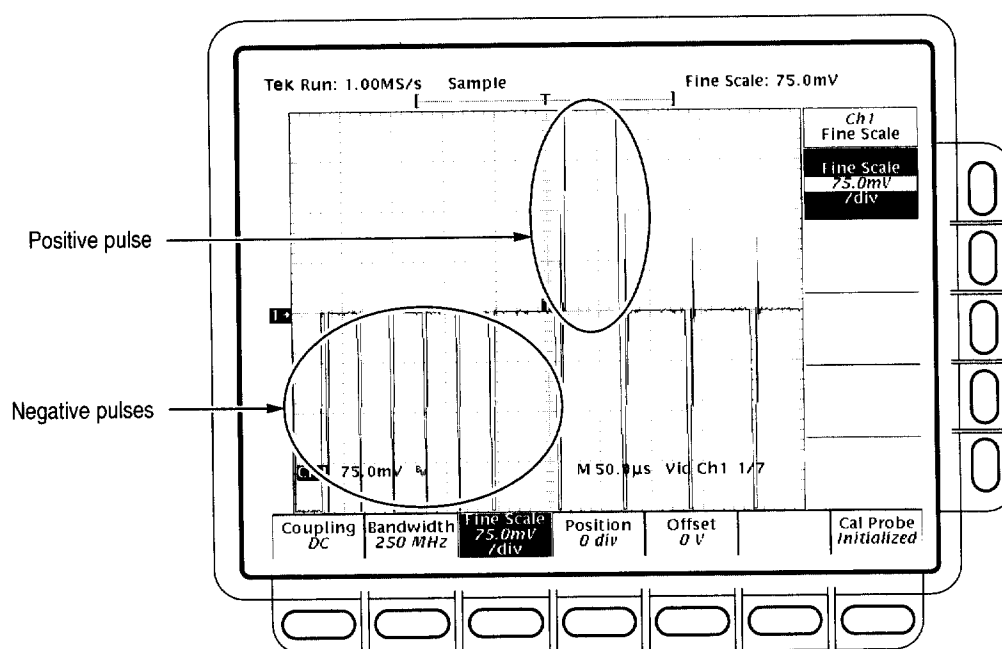
Figure 1–31: Triggered signal range test – 75 mV
