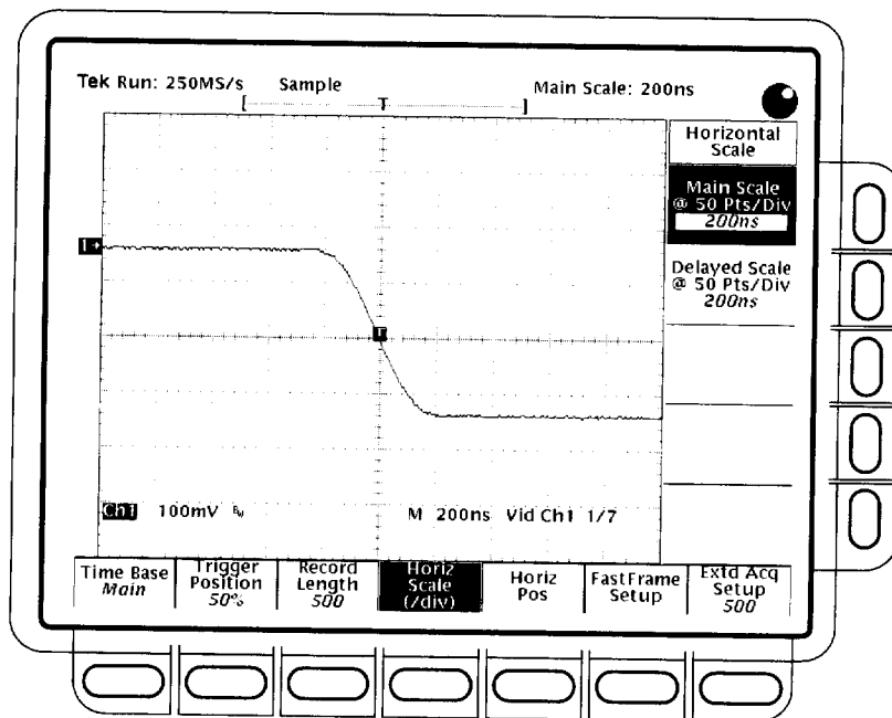
Figure 1-28: Jitter test displayed waveform – TDS 754D shown
