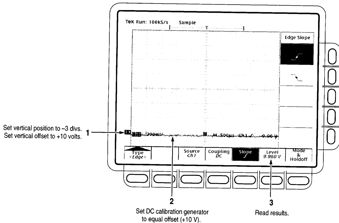
Figure 1-18: Measurement of trigger-level accuracy
