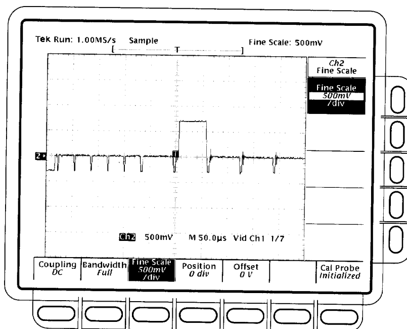
Figure 1-35: 60 Hz Rejection test result – TDS 684C shown
