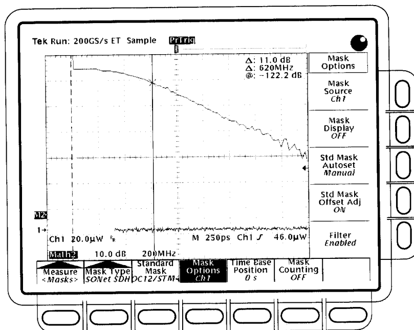
Figure 1-46: Optical impulse response for OC-12 SONET Reference Receiver
