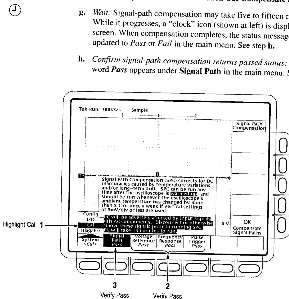
Figure 1–2: Verifying adjustments and signal-path compensation
