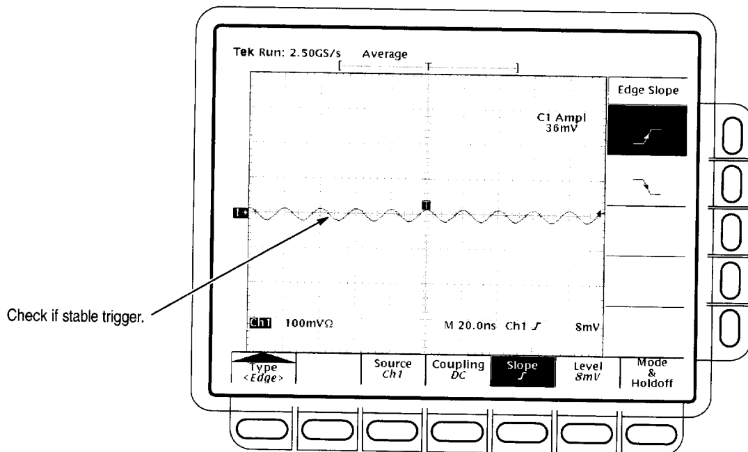
Figure 1-20: Measurement of trigger sensitivity – 50 MHz results shown on a TDS 684C screen
