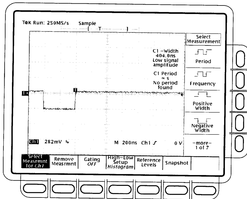
Figure 1-40: Sync duty cycle test: one-div neg pulse waveform
