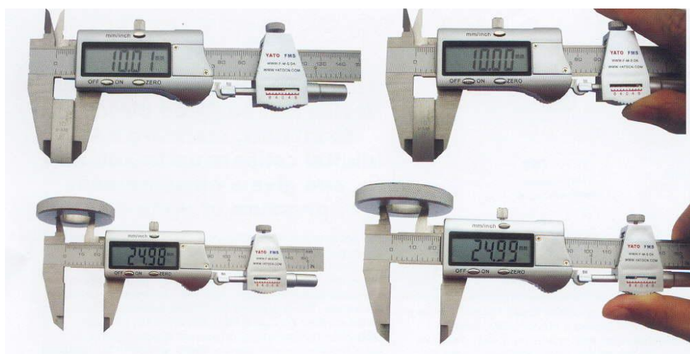
External and internal pressure with a genuine 2-way pressure device. Push or pull. The measurement force used can be seen directly on the device scale.
