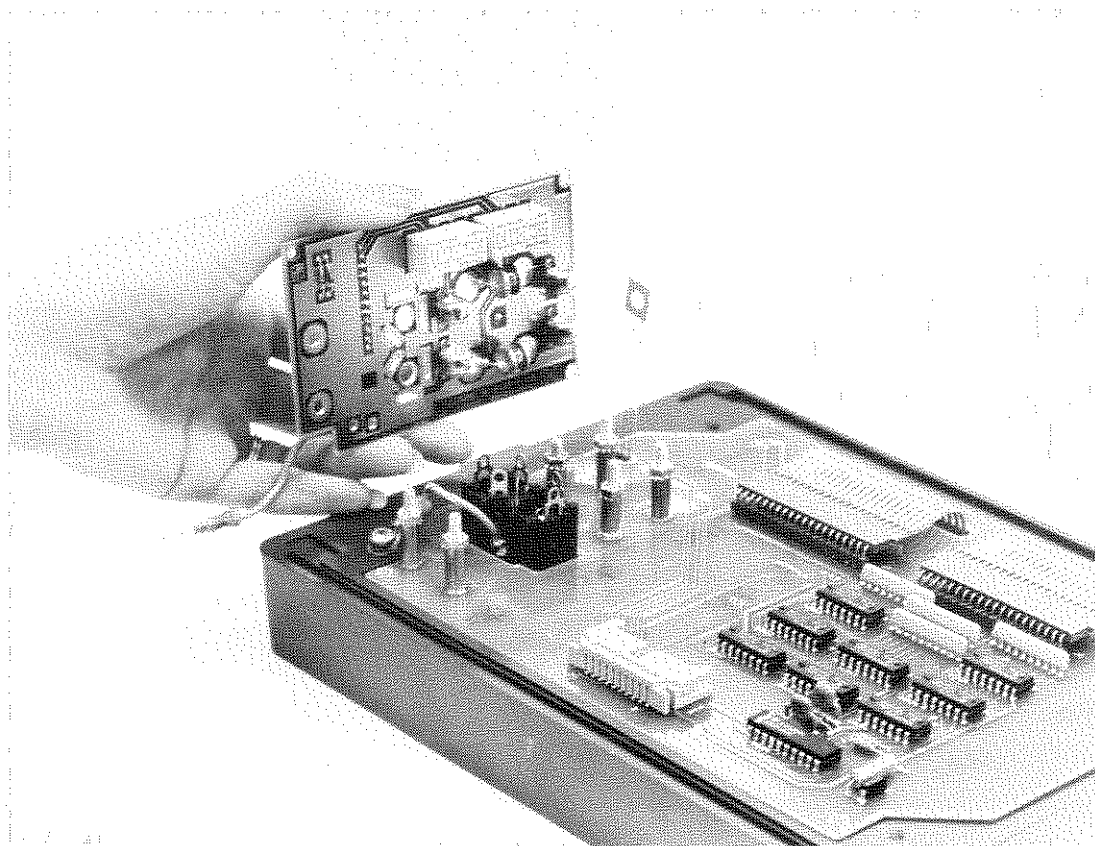
Figure 6-6. 310 Connector Installation
