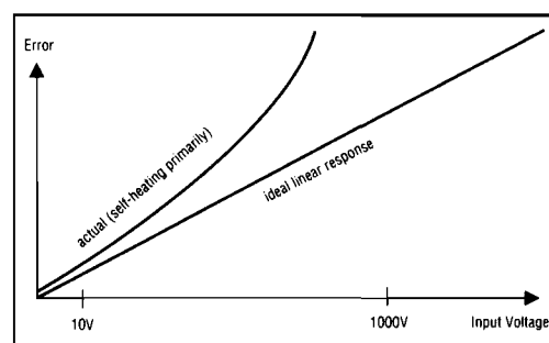
Figure 3. On the 1000 V range, nonlinear self-heating errors of the 100:1 resistive attenuator are noticeable.
