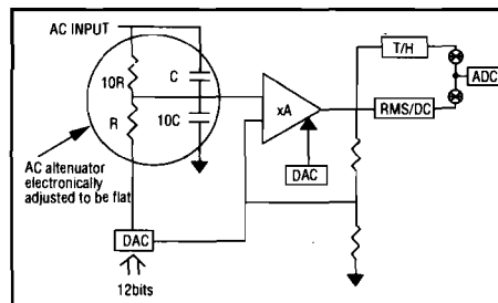
Figure 4. The AC input paths are first adjusted for flatness. Later, in the normal calibration process, gain adjustments are made.
