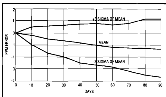
Figure 1. This plot shows stability with time of the reference voltage standard used in the HP 3458A Multimeter.
