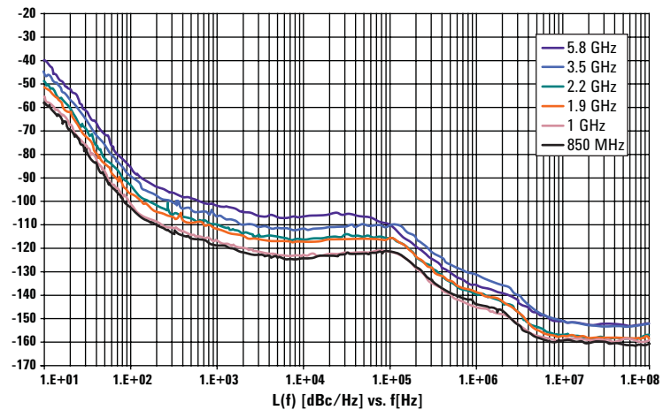
Single sideband phase noise in low floor mode
