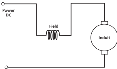
Fig 3: Series excited DC motor
