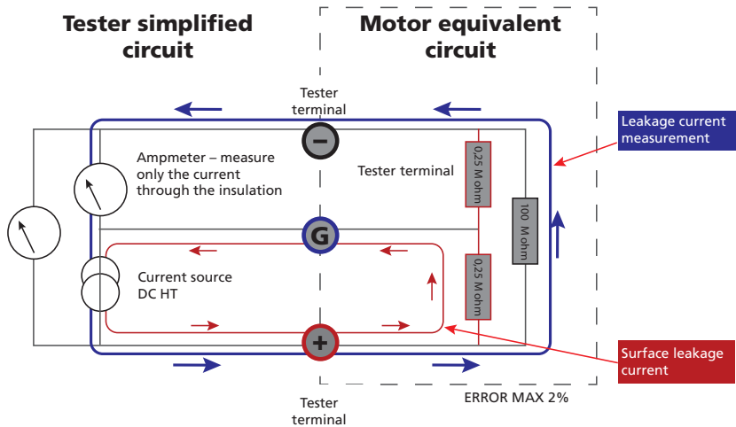
Fig 18: Guard Diagram
