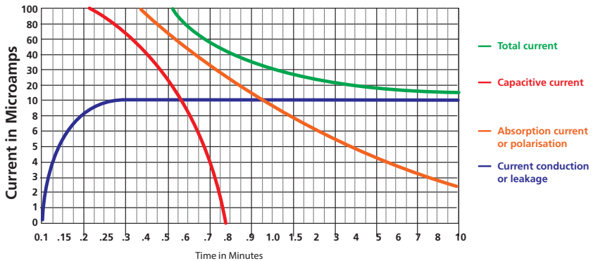
Fig 12: Current elements under test
