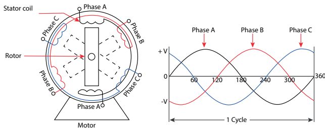
Fig 7: 3 phase motor
