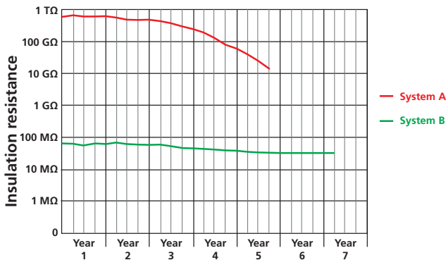
Fig 11: Insulation resistance rate graph
