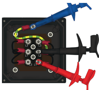
Fig 17: Guard connected to ground
