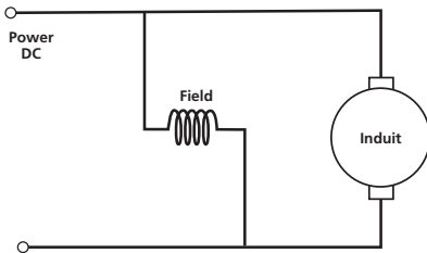
Fig 4: Shunt excited DC motor
