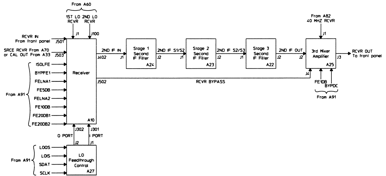
Receiver Block Diagram
