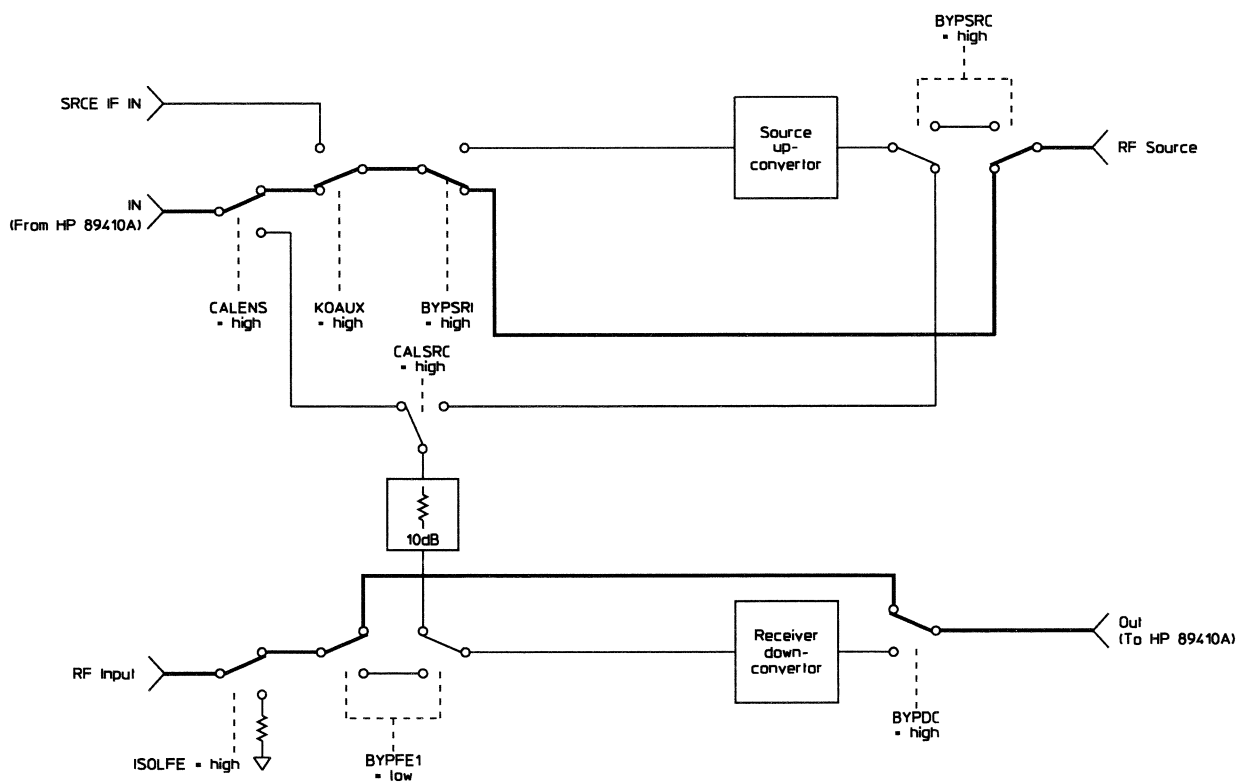
Bypass Signal Path
