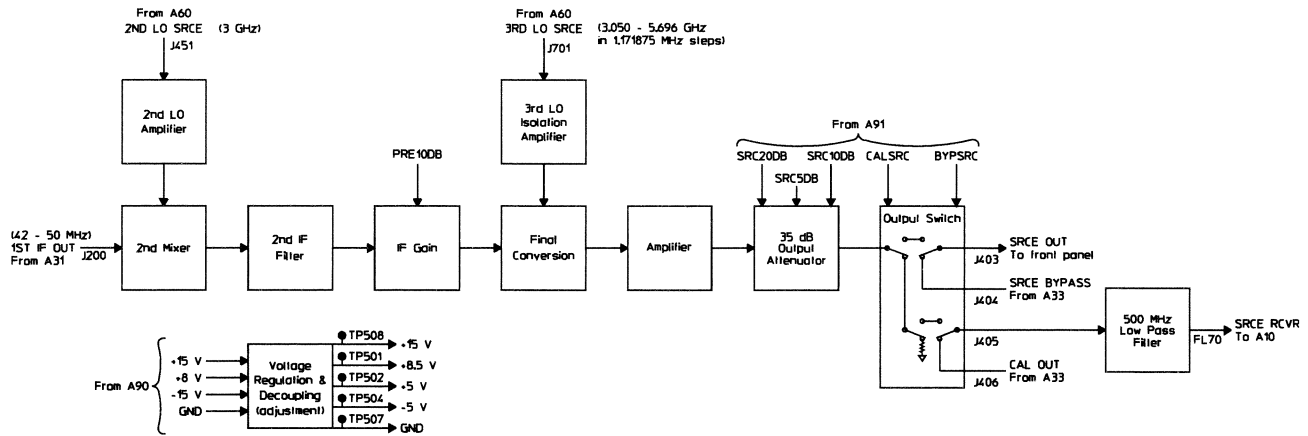
A70 Source Block Diagram
