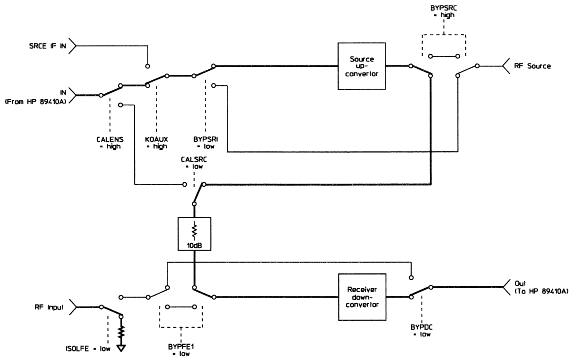
Through Signal Path
