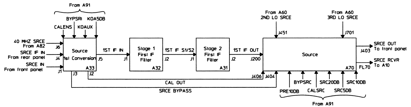
Source Block Diagram
