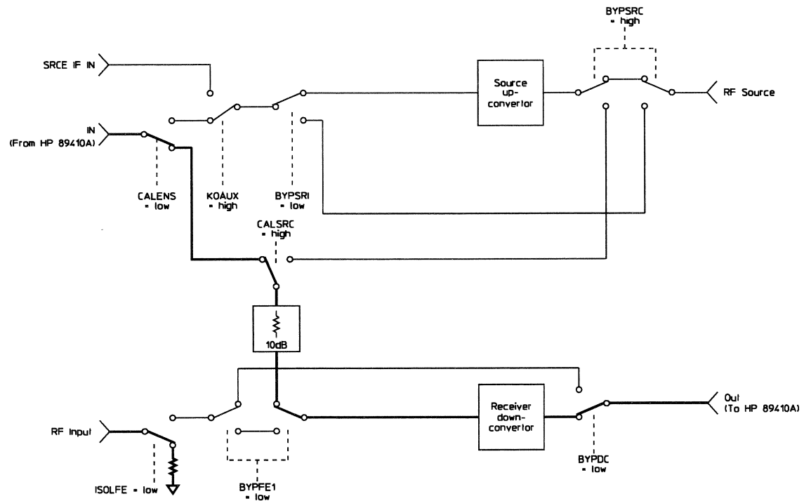
Calibration Signal Path
