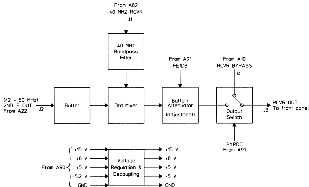
A25 3rd Mixer Amplifier Block Diagram
