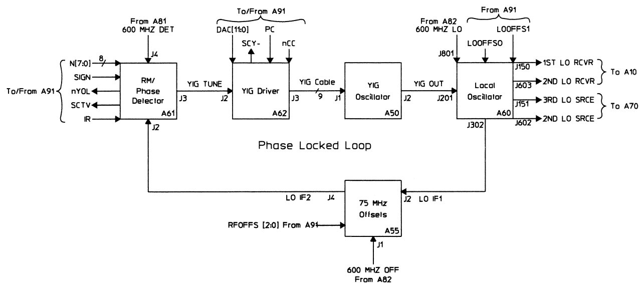
Local Oscillator Block
