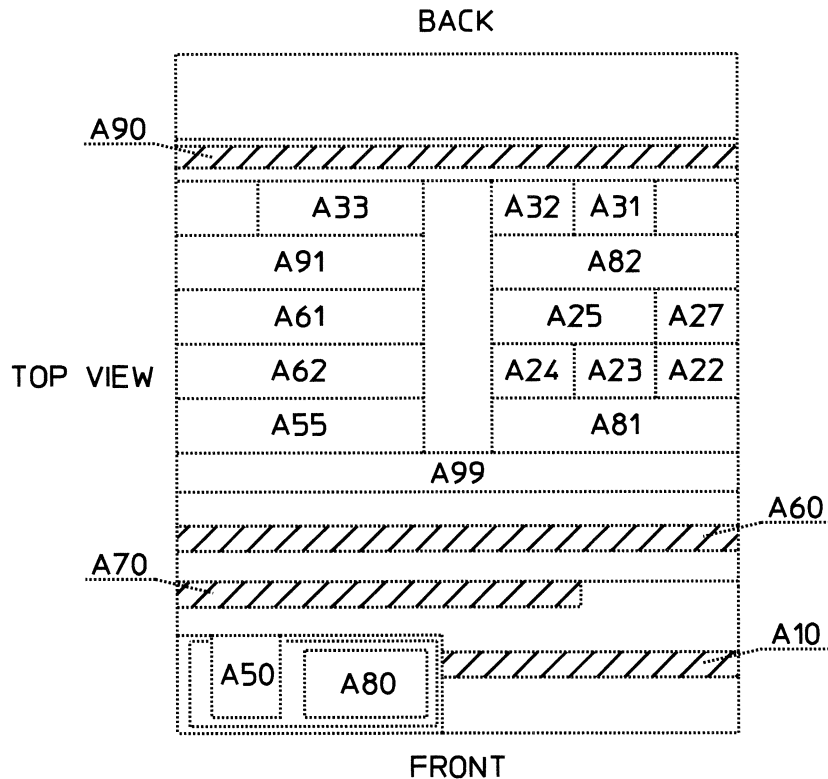
Assembly Locations
