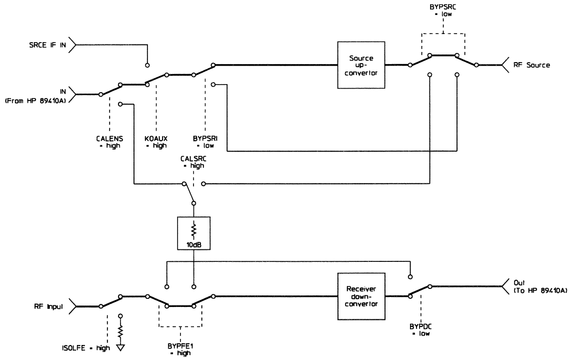
Normal Signal Path
