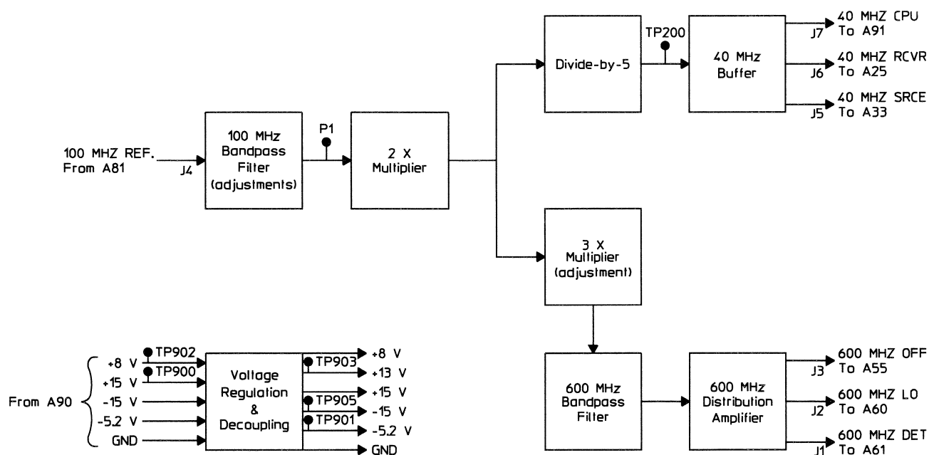
A82 600 MHz Reference Block Diagram
