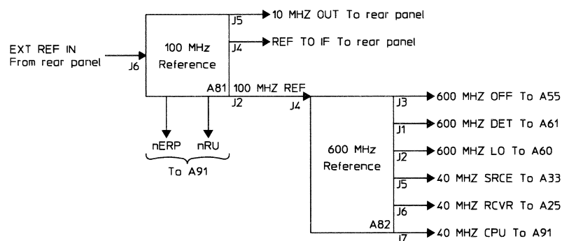
Frequency Reference Block Diagram
