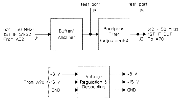
A31 Stage 2 First IF Filter Block Diagram
