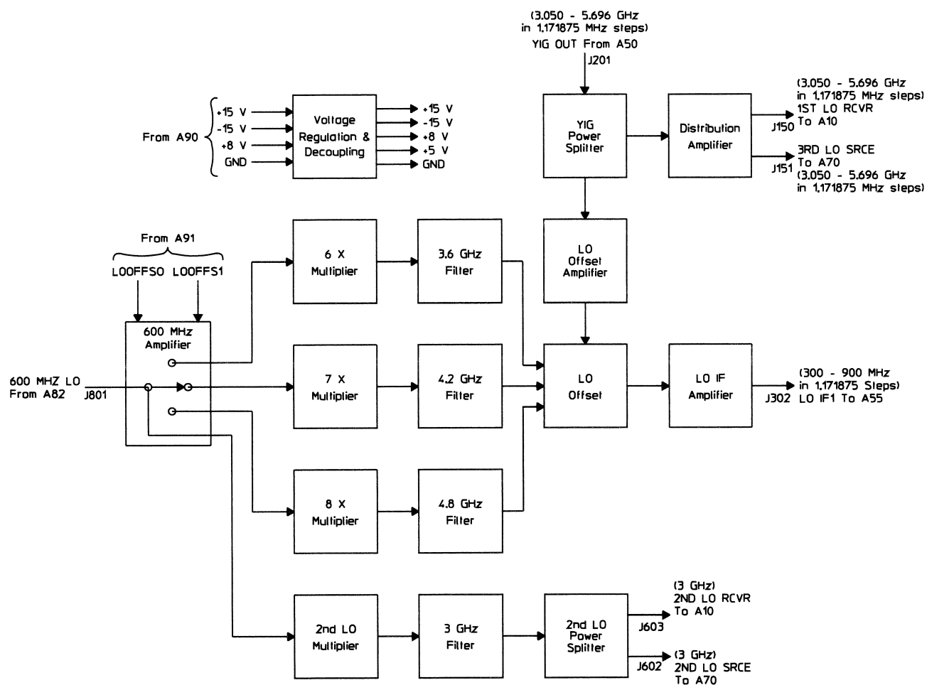
A60 Local Oscillator Block Diagram
