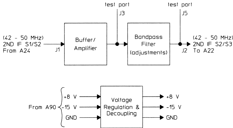
A23 Stage 2 Second IF Filter Block Diagram
