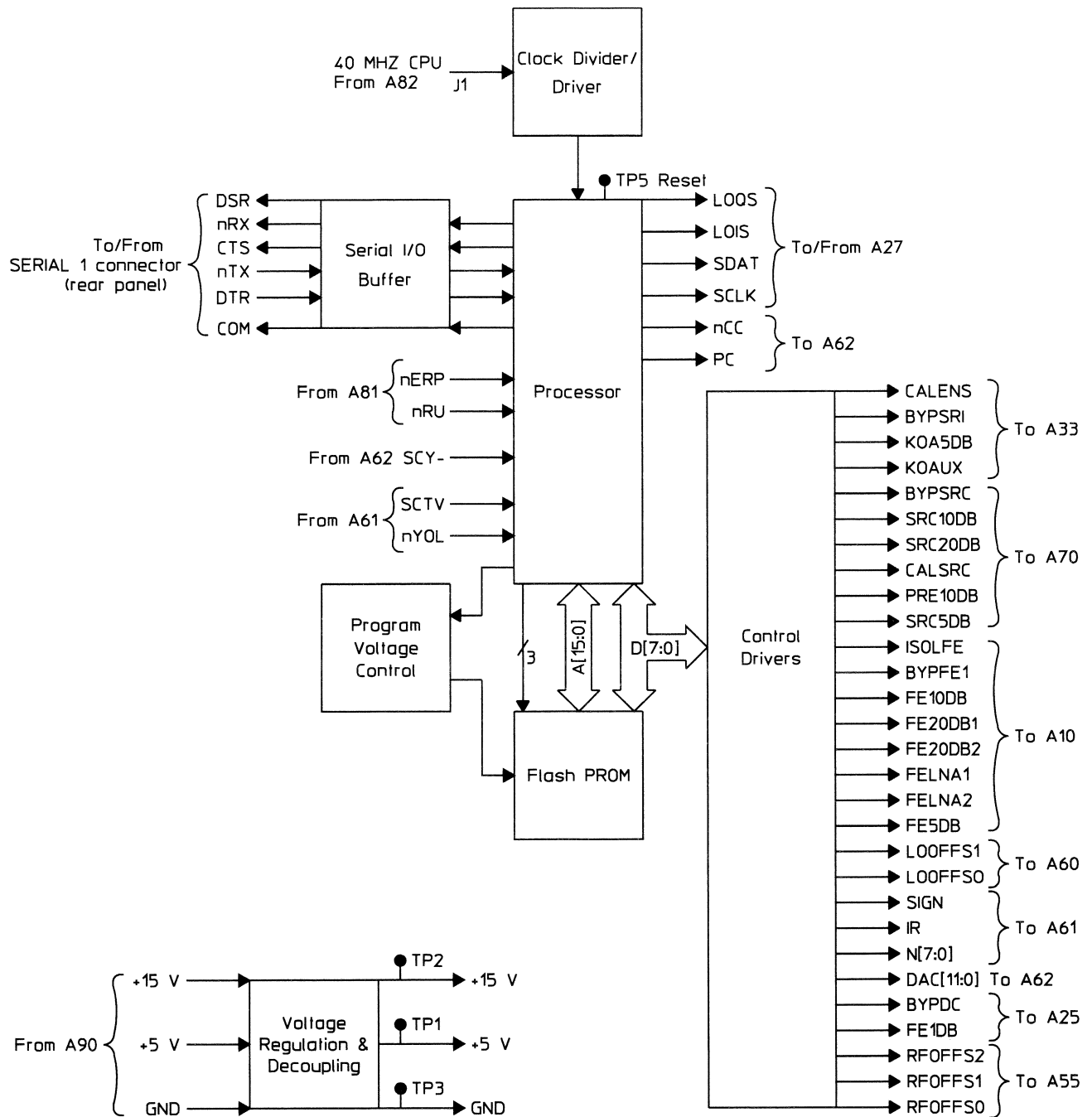
A91 Digital Control Block Diagram
