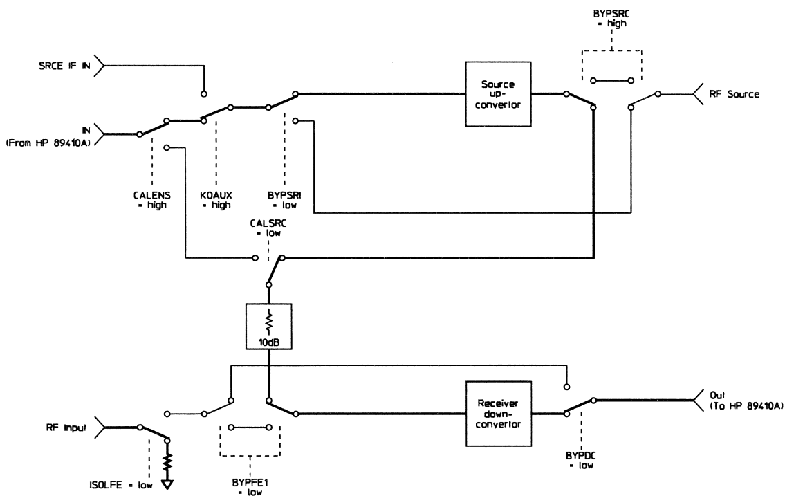
Through Signal Path
