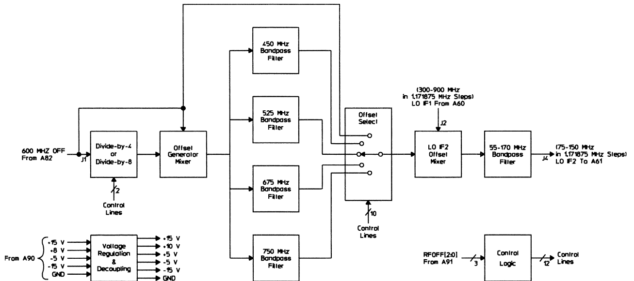
A55 75 MHz Offsets Block Diagram
