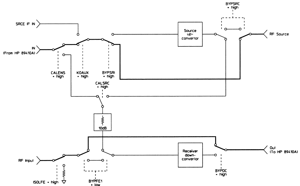
Bypass Signal Path
