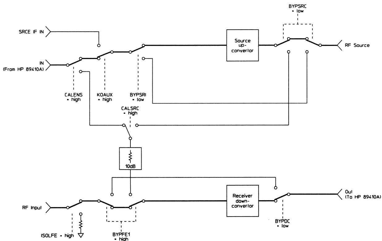
Normal Signal Path
