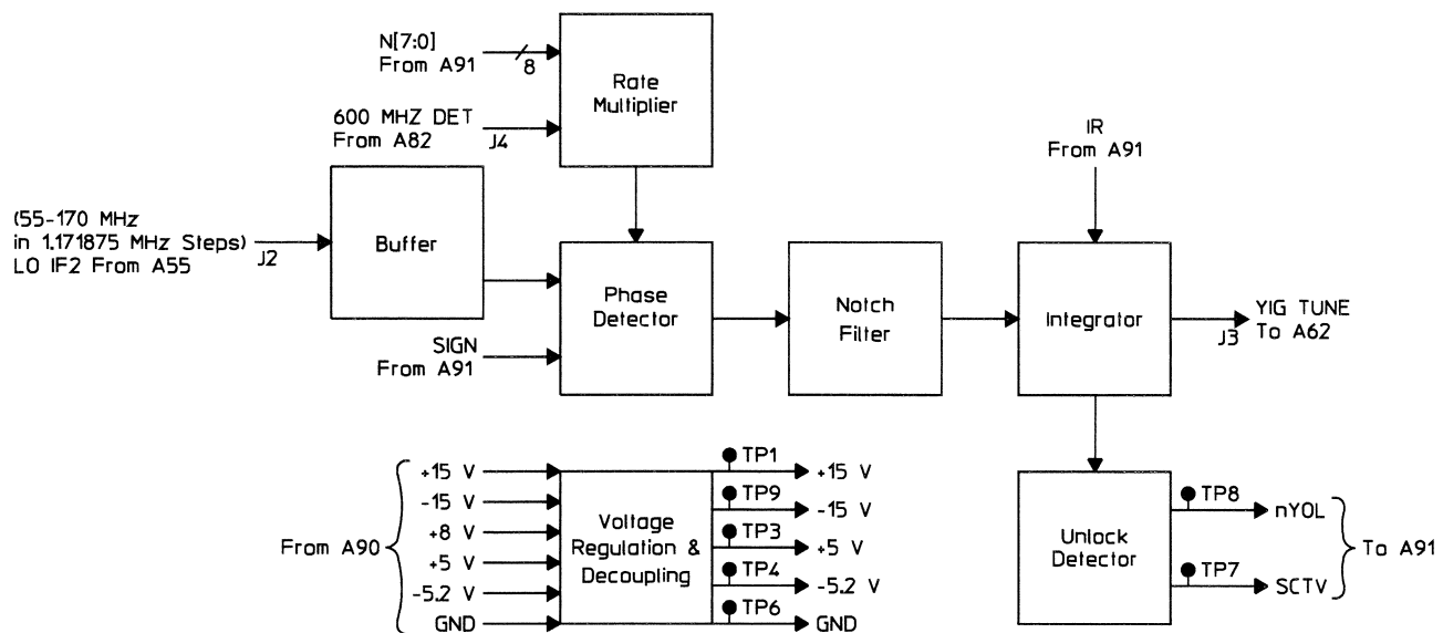
A61 RM/Phase Detector Block Diagram
