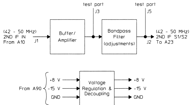
A24 Stage 1 Second IF Filter Block Diagram
