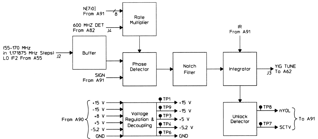
A61 RM/Phase Detector Block Diagram
