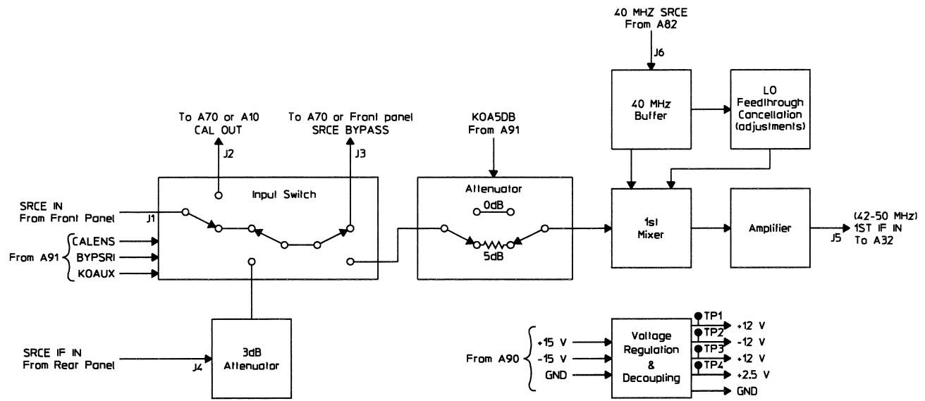
A33 Source 1st Conversion Block Diagram
