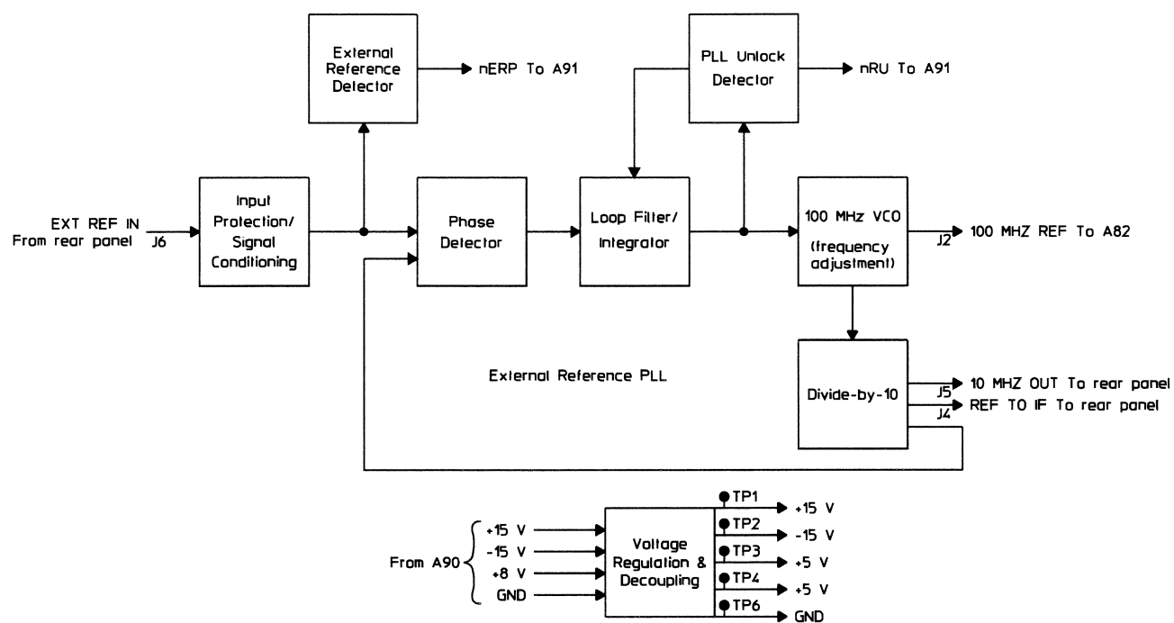
A81 100 MHz Reference Block Diagram
