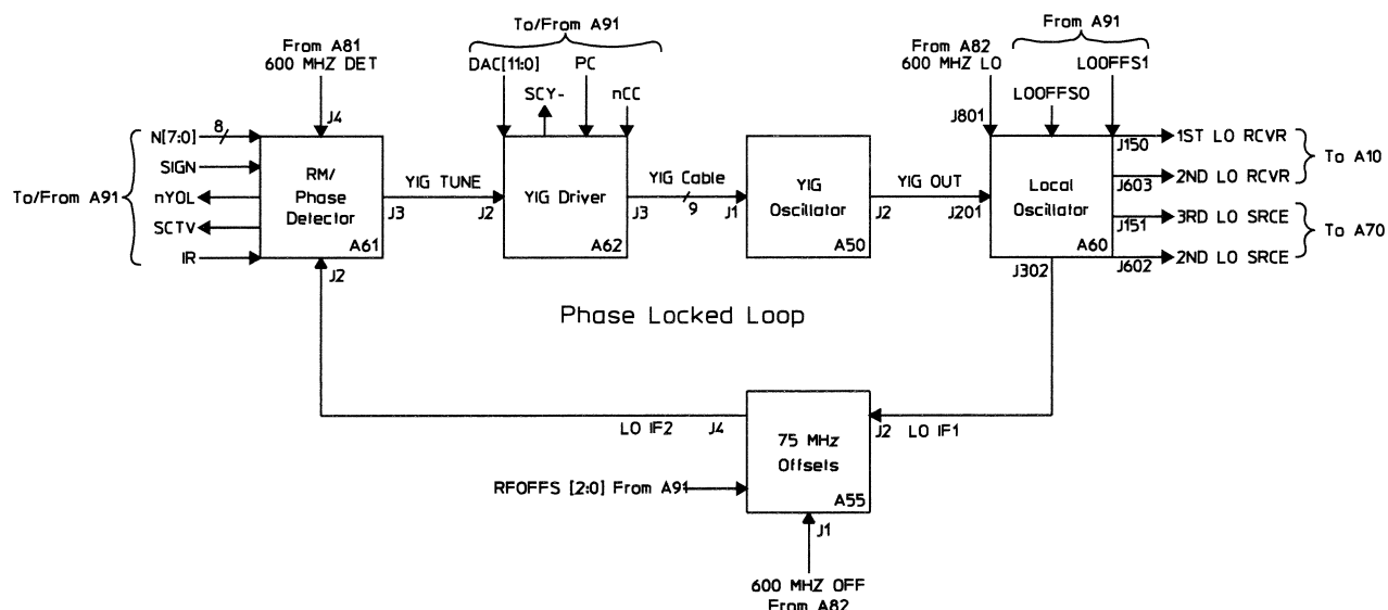
Local Oscillator Block Diagram
