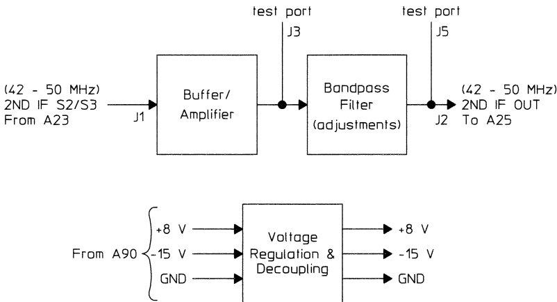
A22 Stage 3 Second IF Filter Block Diagram
