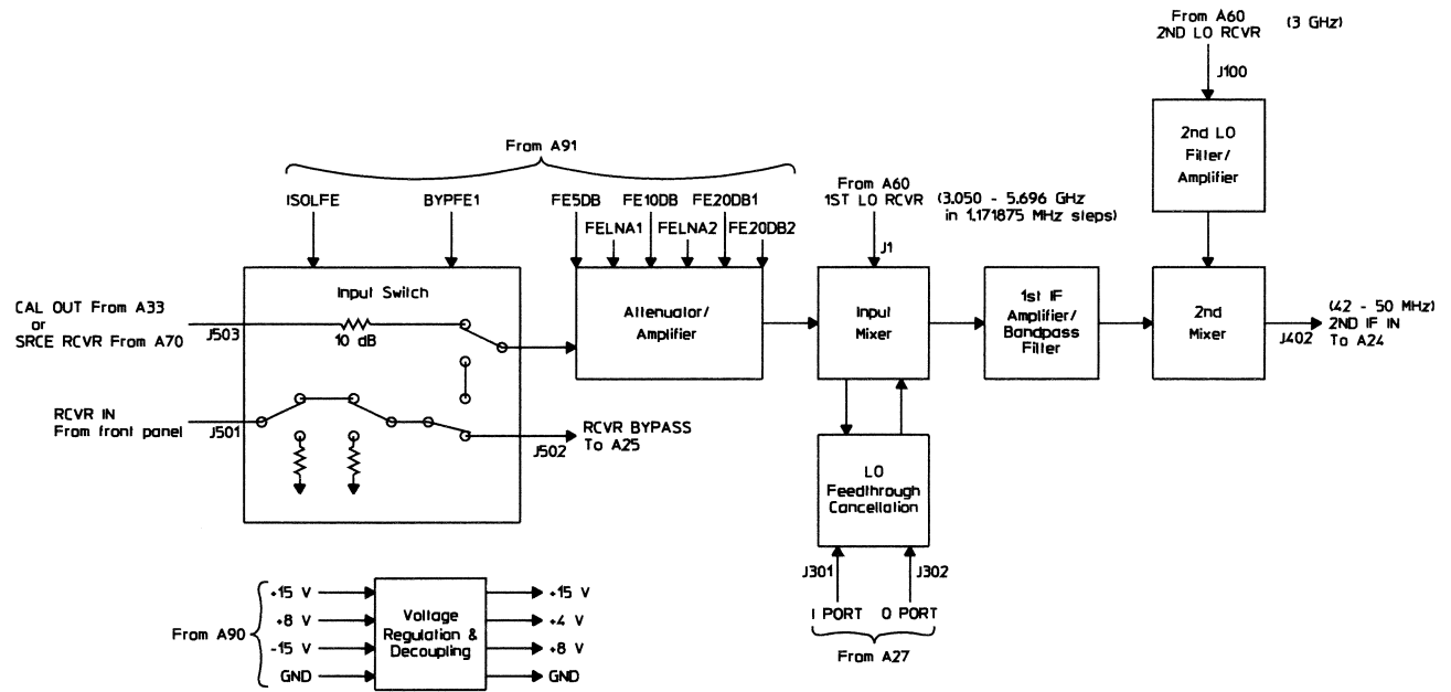
A10 Receiver Block Diagram
