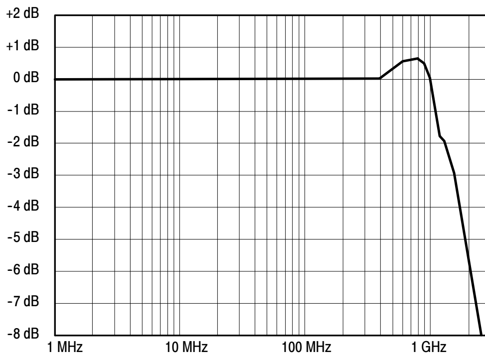
Figure 3-1: Typical Bandwidth
