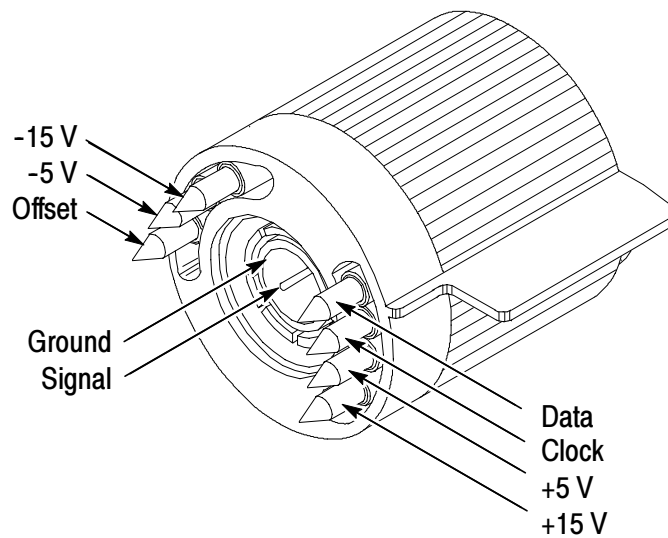
Figure 4-2: TEKPROBE Interface
