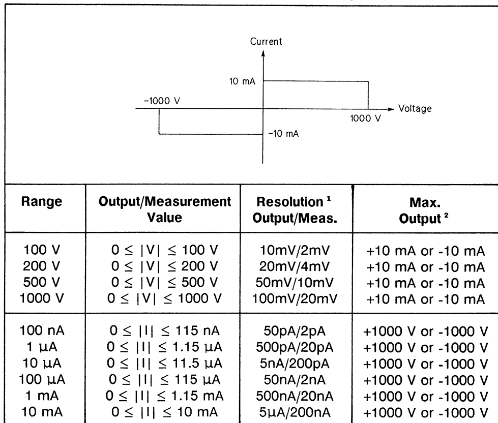
HVU Output/Measurement Ranges
