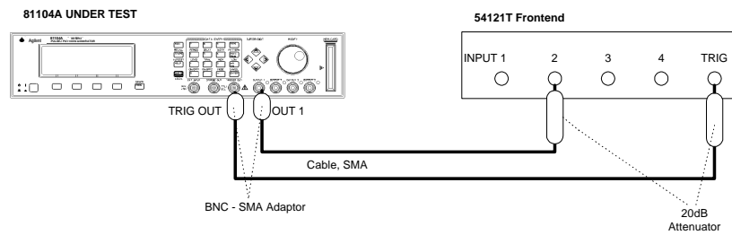
Connecting Agilent 81104A to the Scope
