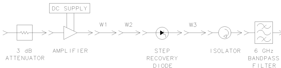
Figure 5-1. 300 MHz Up-Converter Block Diagram
