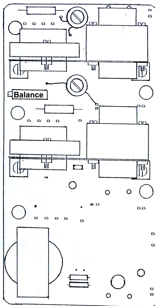
Figure 6b 2 and 2 1/2 element models with option E, the 4 to 20 ADC output.
