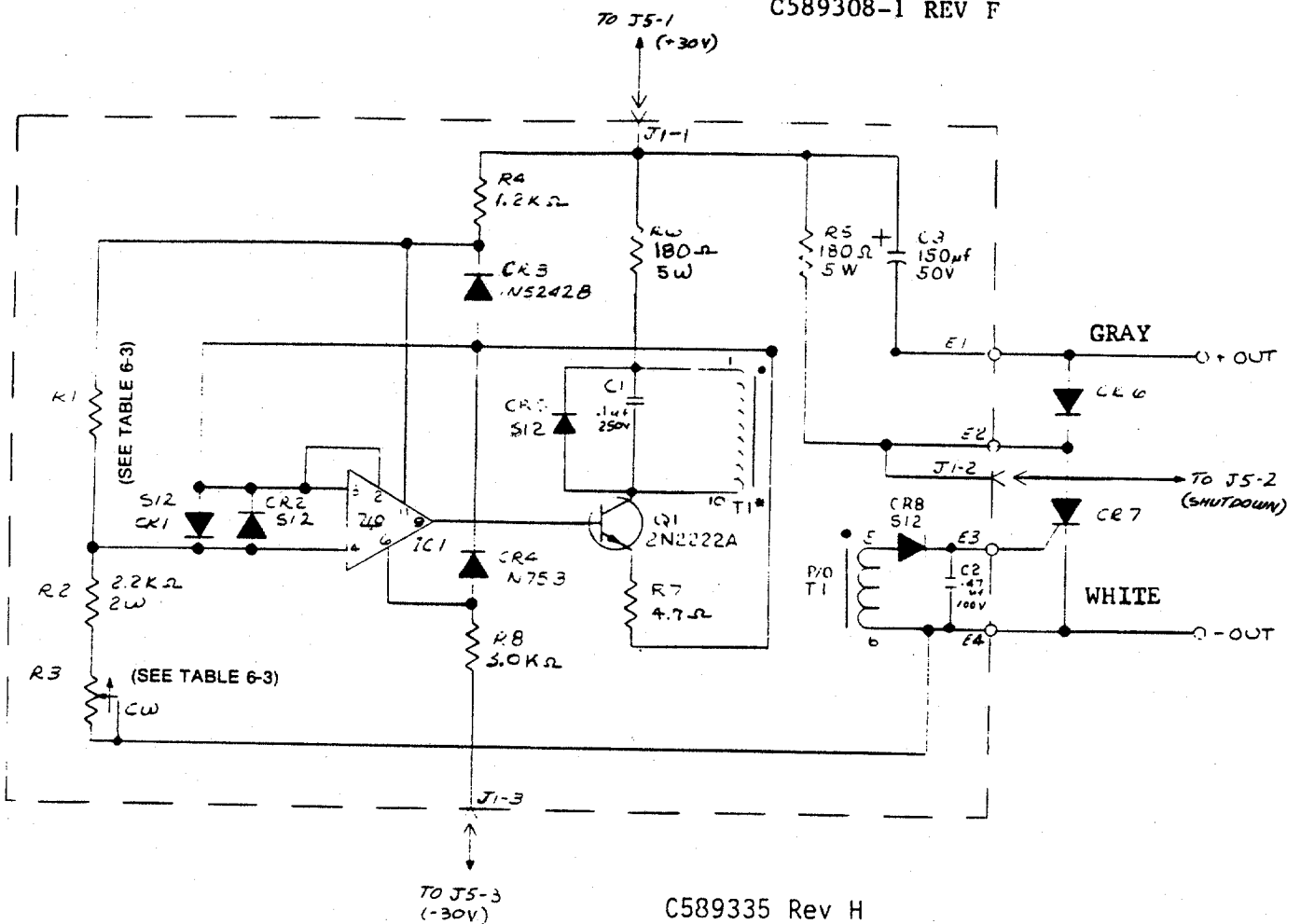
C589308-1 REV F
