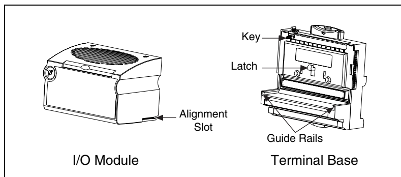
Figure 2-7. Module Installation Diagram
