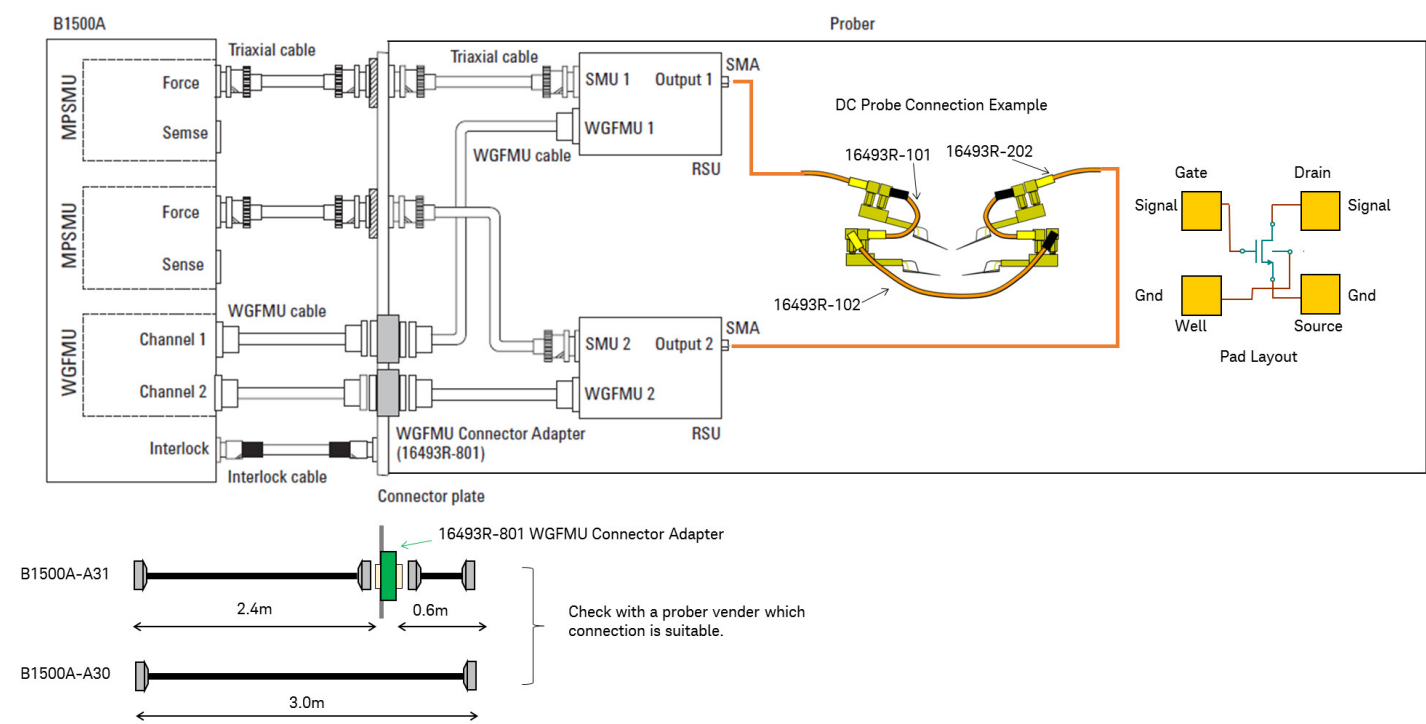
Example-9. For NBTI measurement using WGFMU with DC probe
