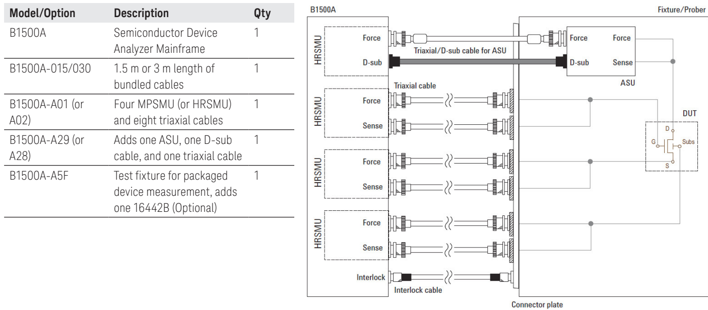
Example-3. For IV characterization of 4-terminal device with ASU
