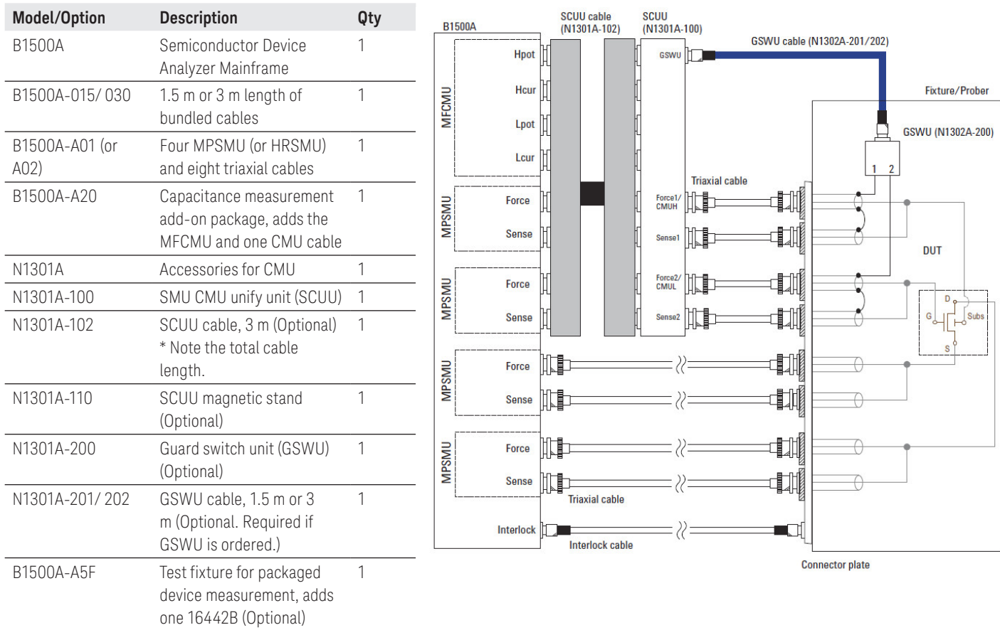
Example-4. For IV/CV characterization of 4-terminal device
