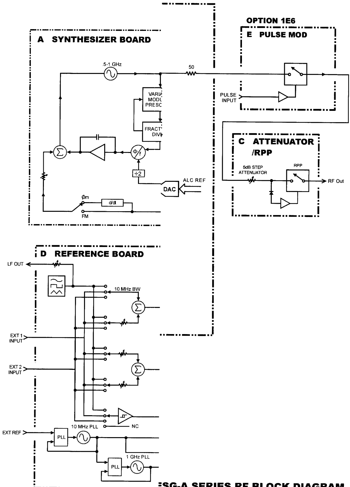
ESG-A SERIES RF BLOCK DIAGRAM STANDARD & OPTION 1E6)
