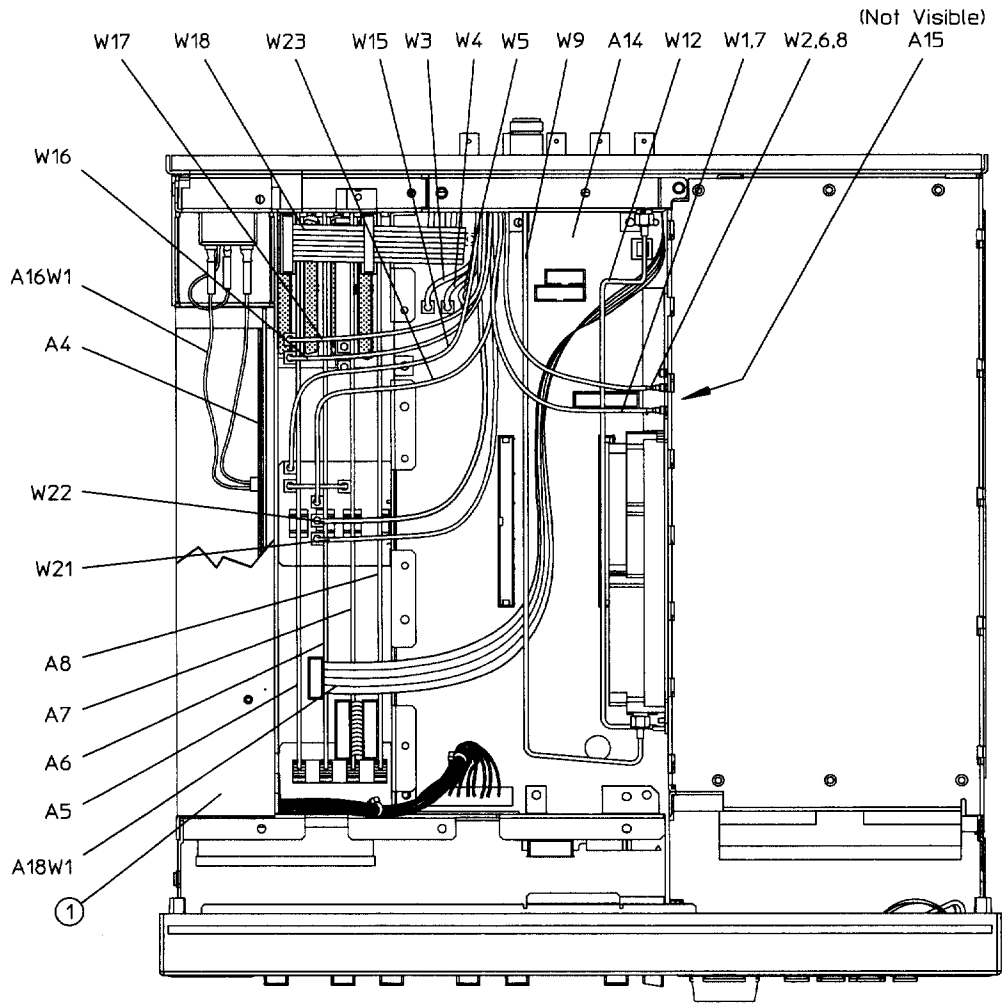
Figure 5-42 Rear Panel (with Option 1EM) (1 of 2)
