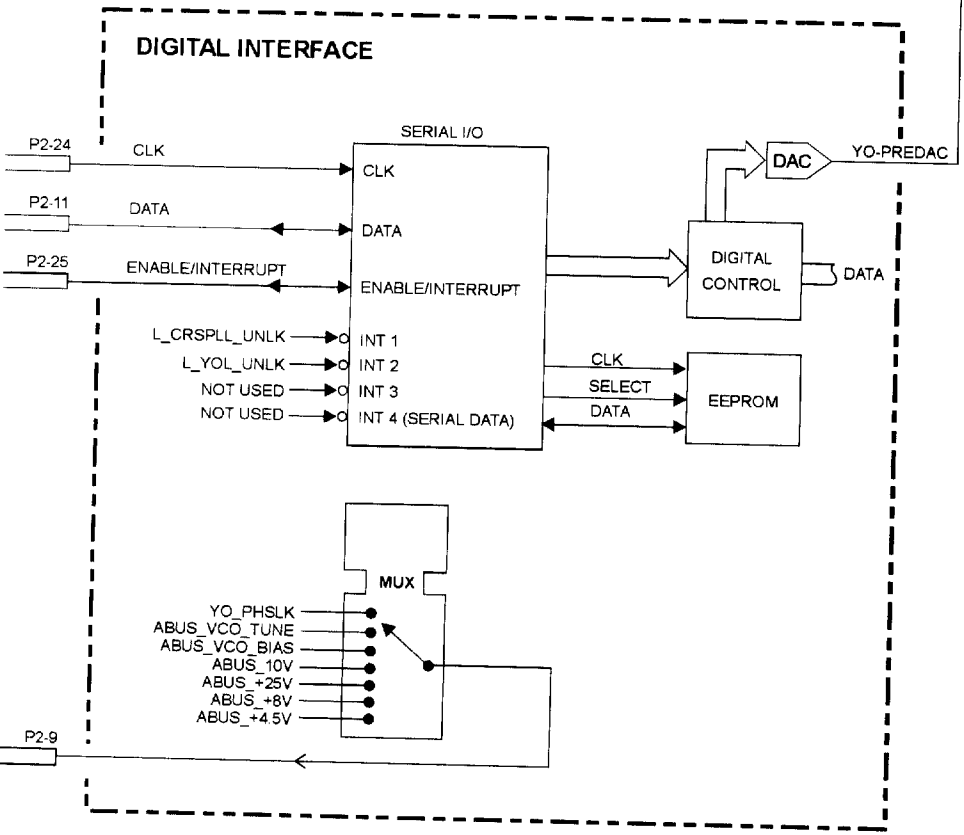
A23 SAMPLER (ESG-AP AND ESG DP SERIES)
