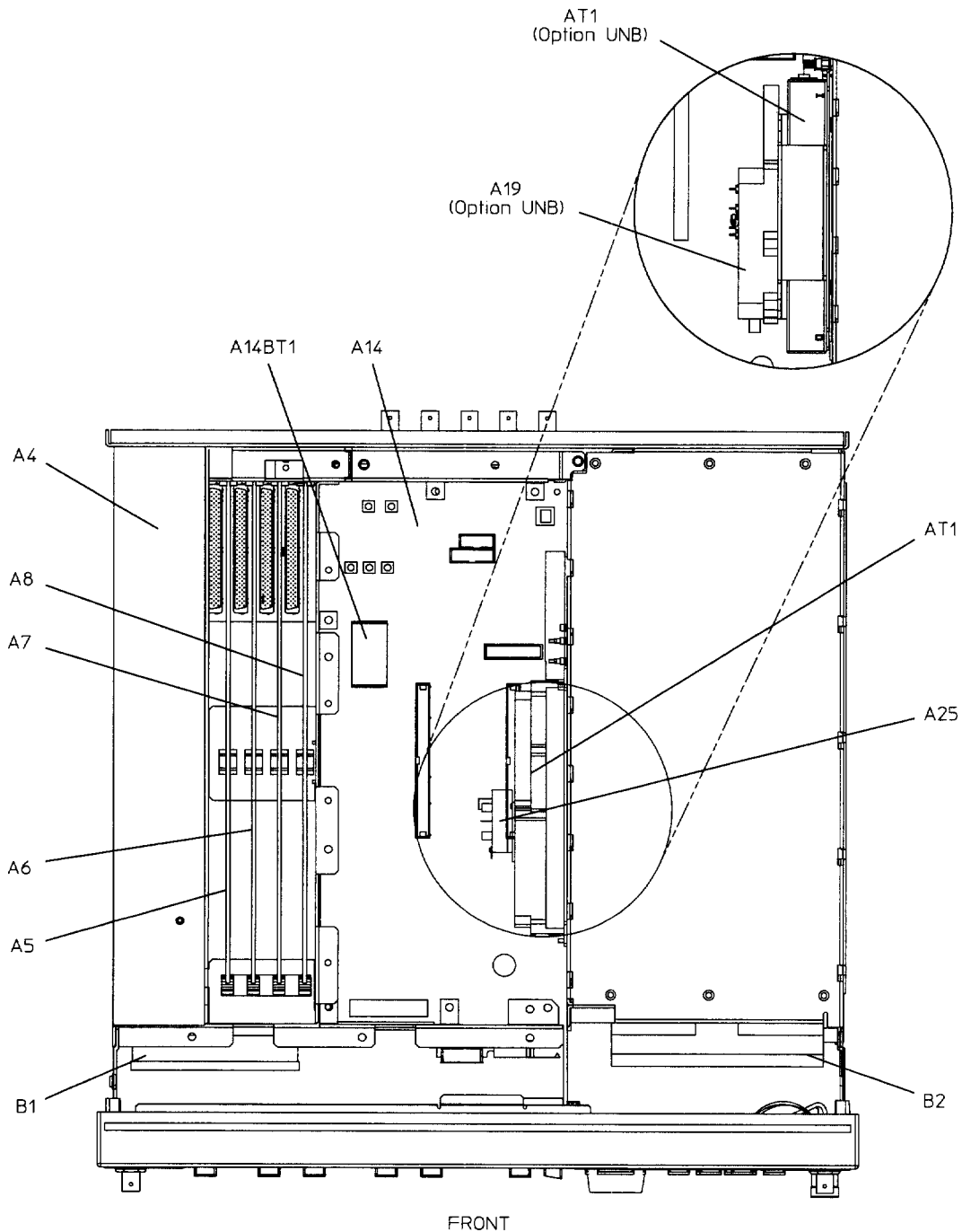
Figure 3-1 Top View
