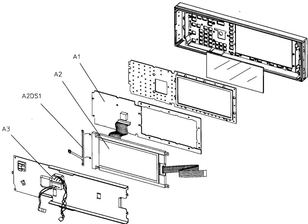
Figure 4-3 Disassembled Front Panel View
