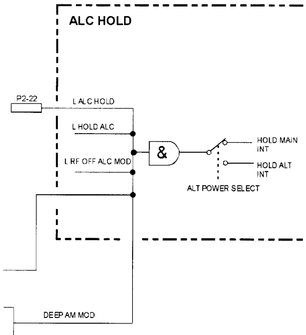
A9 OUTPUT BLOCK DIAGRAM (ESG-A SERIES)
