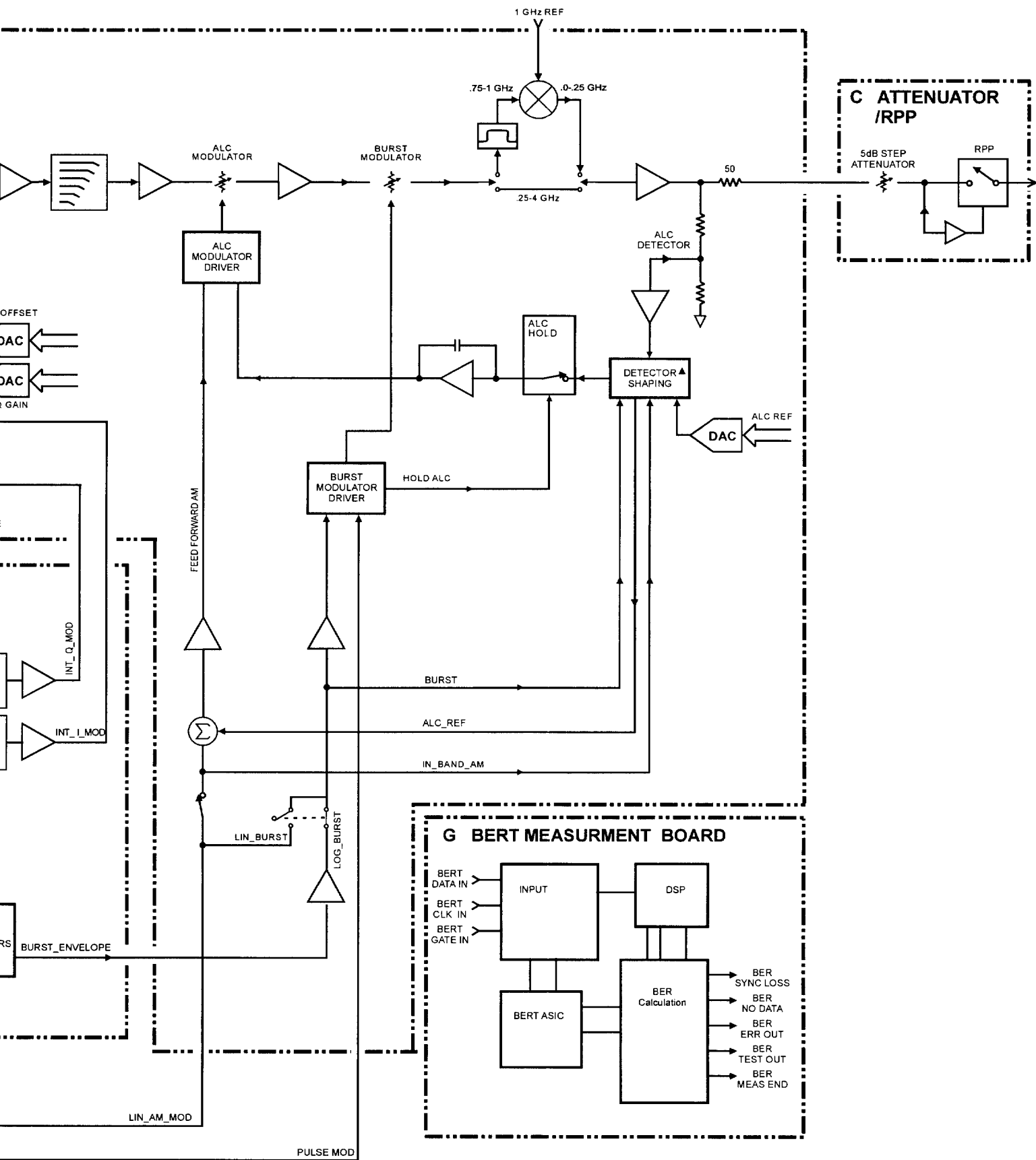
ESG-D SERIES RF BLOCK DIAGRAM (OPTION UN7)
