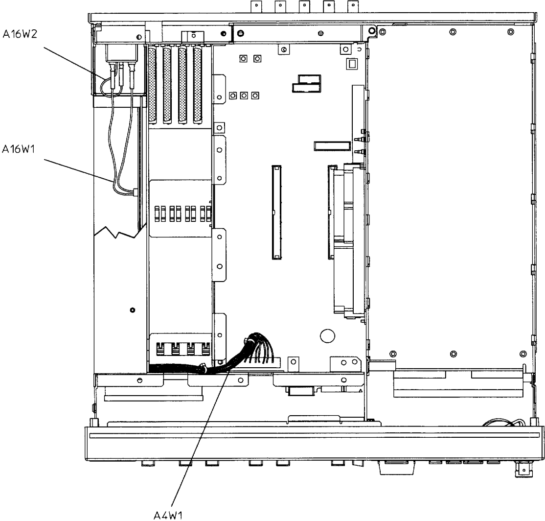
Figure 3-6 Top View (ESG-A Series)
