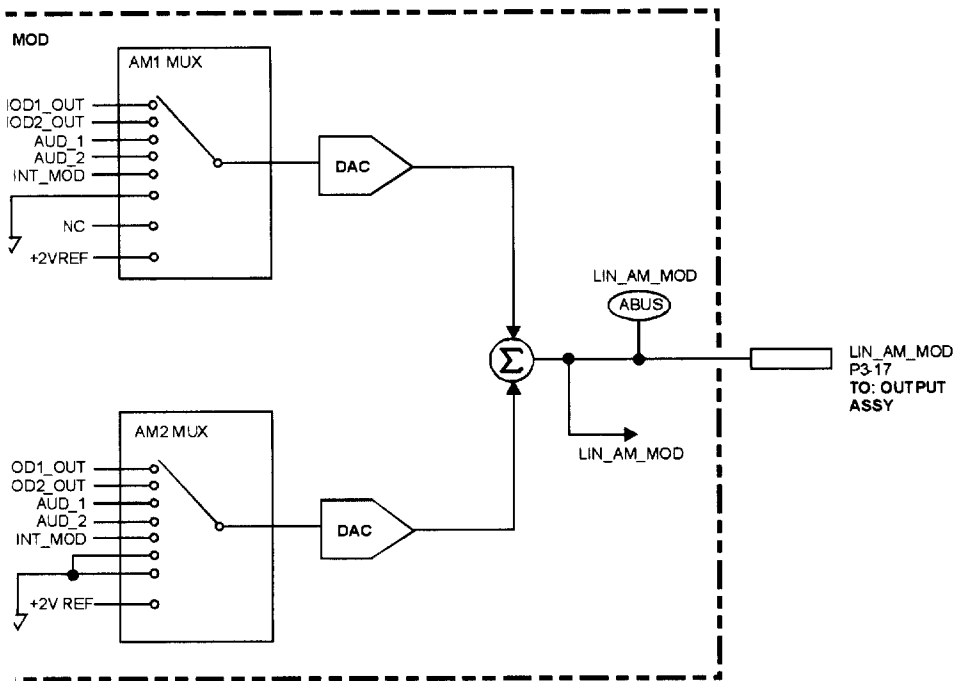
REFERENCE BLOCK DIAGRAM (ESG-AP & ESG-DP SERIES)
