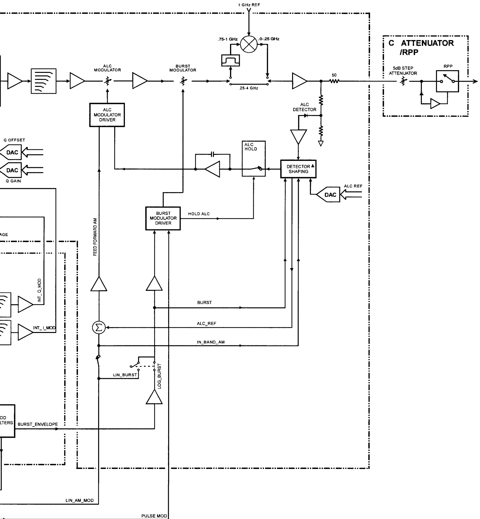
ESG-D SERIES RF BLOCK DIAGRAM (OPTIONS UN3 & UN4)
