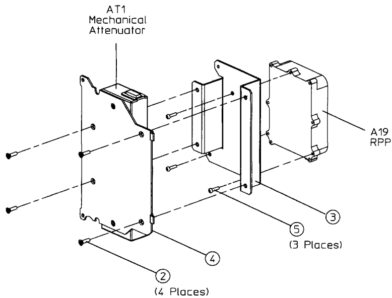
Figure 5-21 A19 Reverse Power Protection (RPP) (3 of 3)
