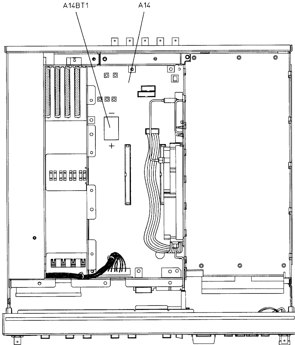
Figure 5-13 A14BT1 Battery
