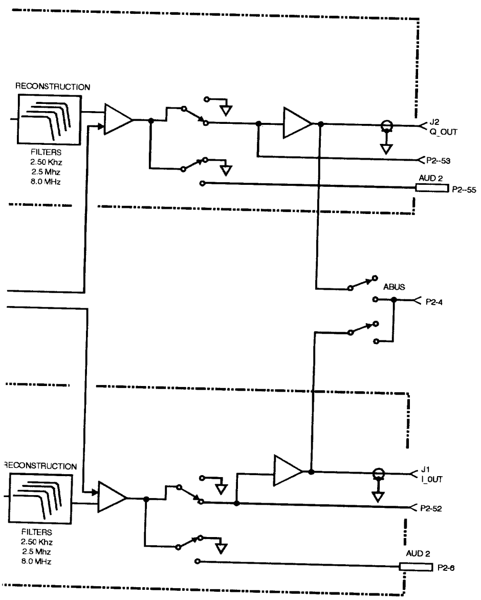
ARBITRARY WAVEFORM GENERATOR BLOCK DIAGRAM (OPT UND)
