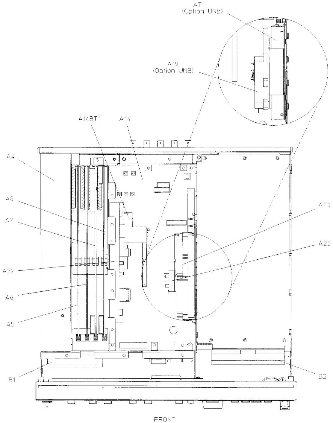
Figure 4-1 Top View
