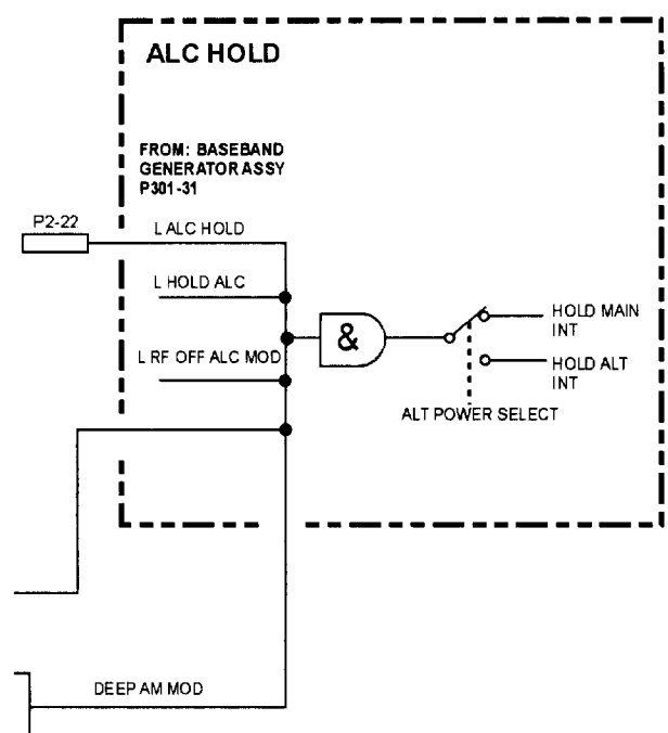
A9 OUTPUT BLOCK DIAGRAM (ESG-D, ESG-DP, & ESG-DP SERIES)
