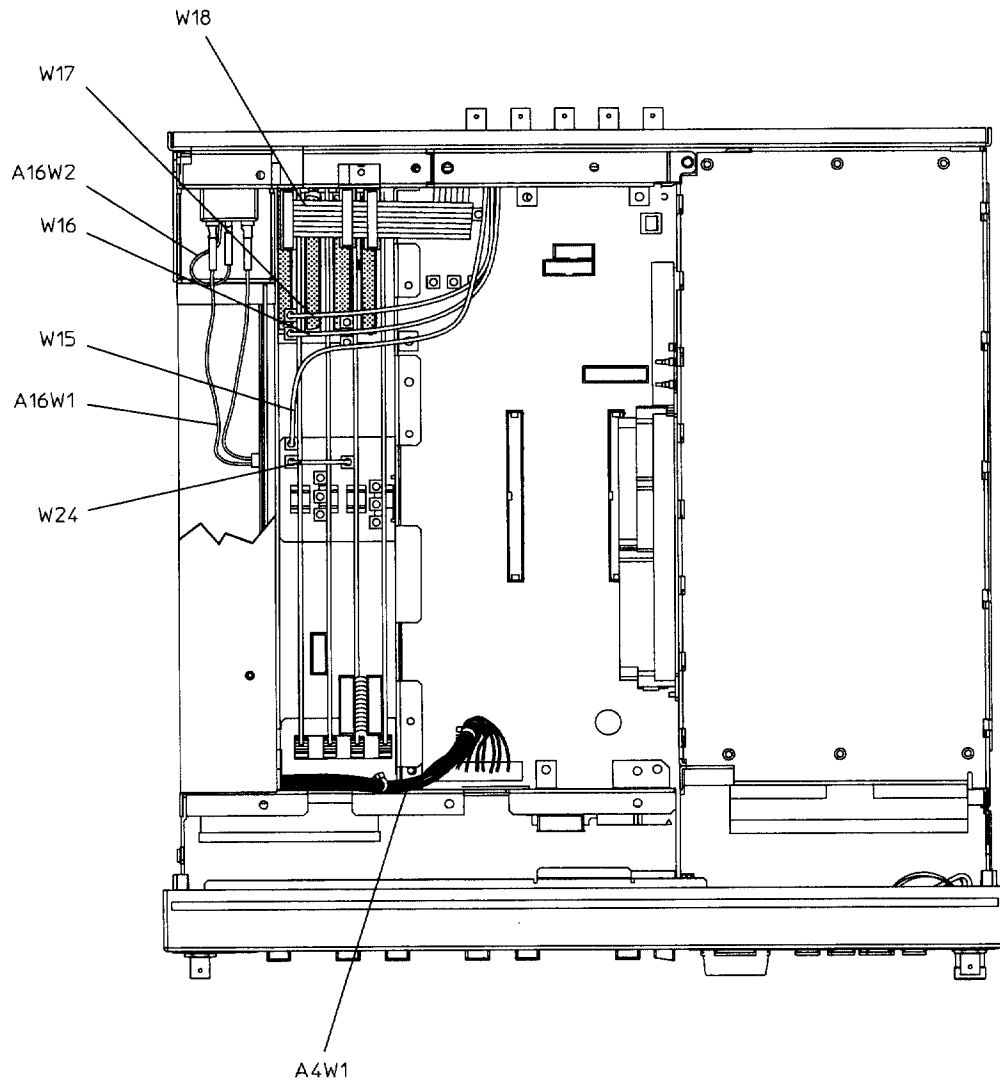
Figure 4-7 Top View (ESG-DP Series - Option UND)
