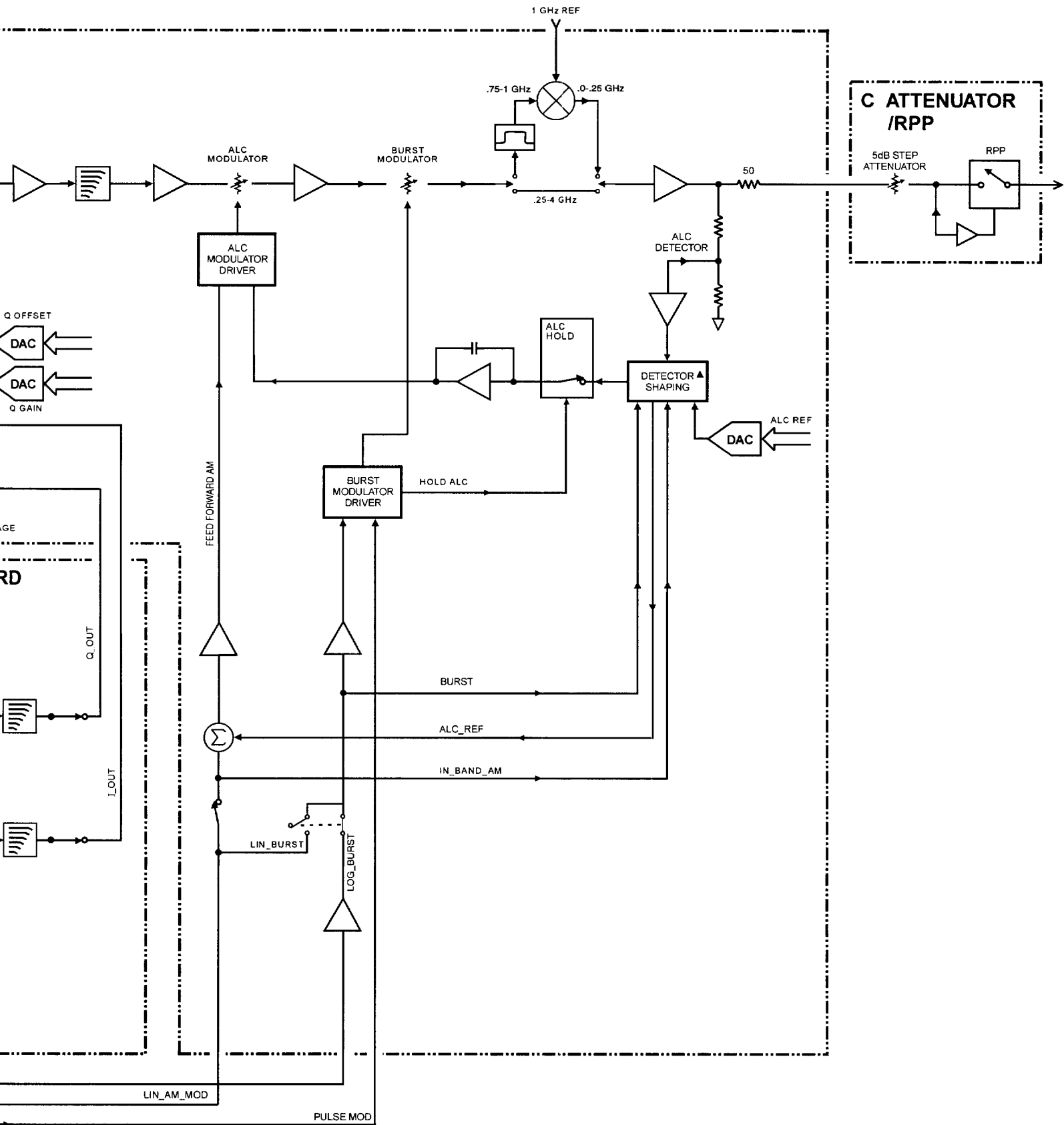
ESG-D SERIES RF BLOCK DIAGRAM (OPTION UND)
