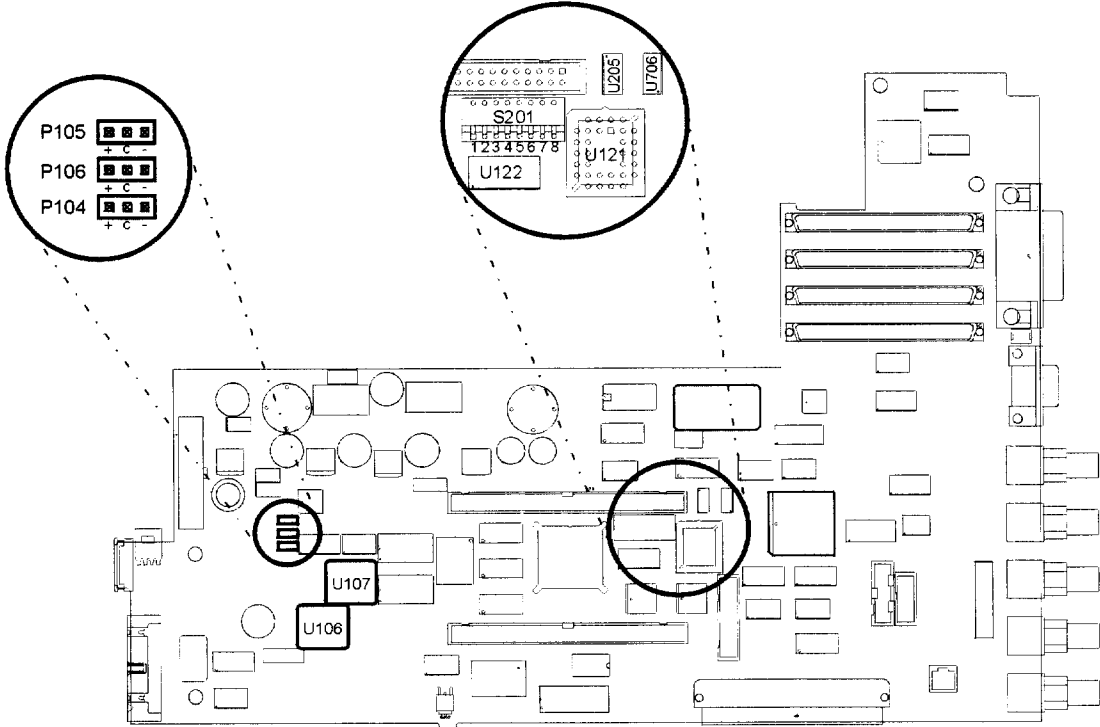
Figure 5-12 A14 CPU/Motherboard (3 of 3)
