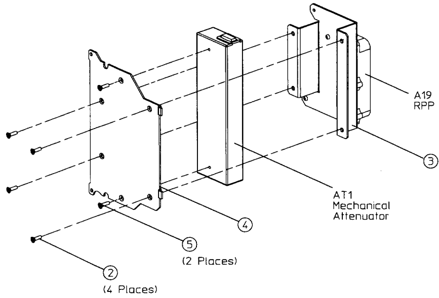
Figure 5-31 AT1 Mechanical Attenuator (3 of 3)
