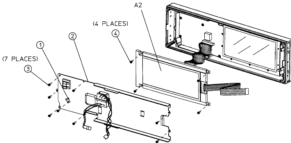
Figure 5-2 A2 Display (1 of 2)
