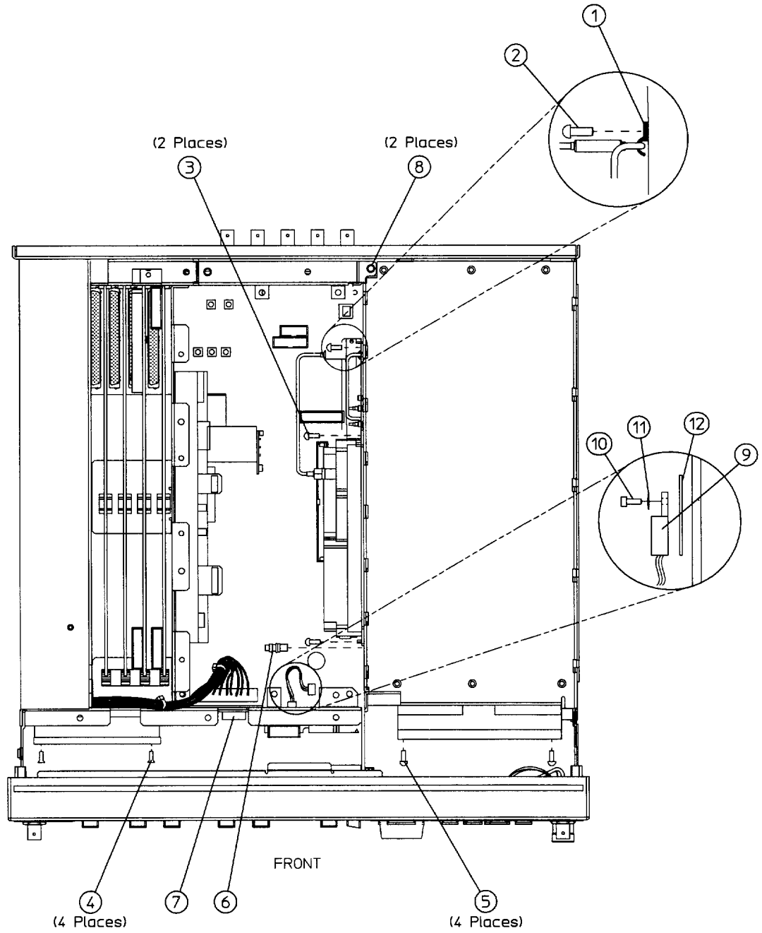
Figure 4-18 Top View
