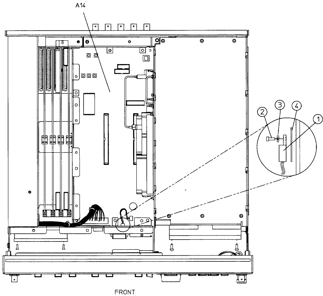
Figure 5-14 A14Q501 Transistor
