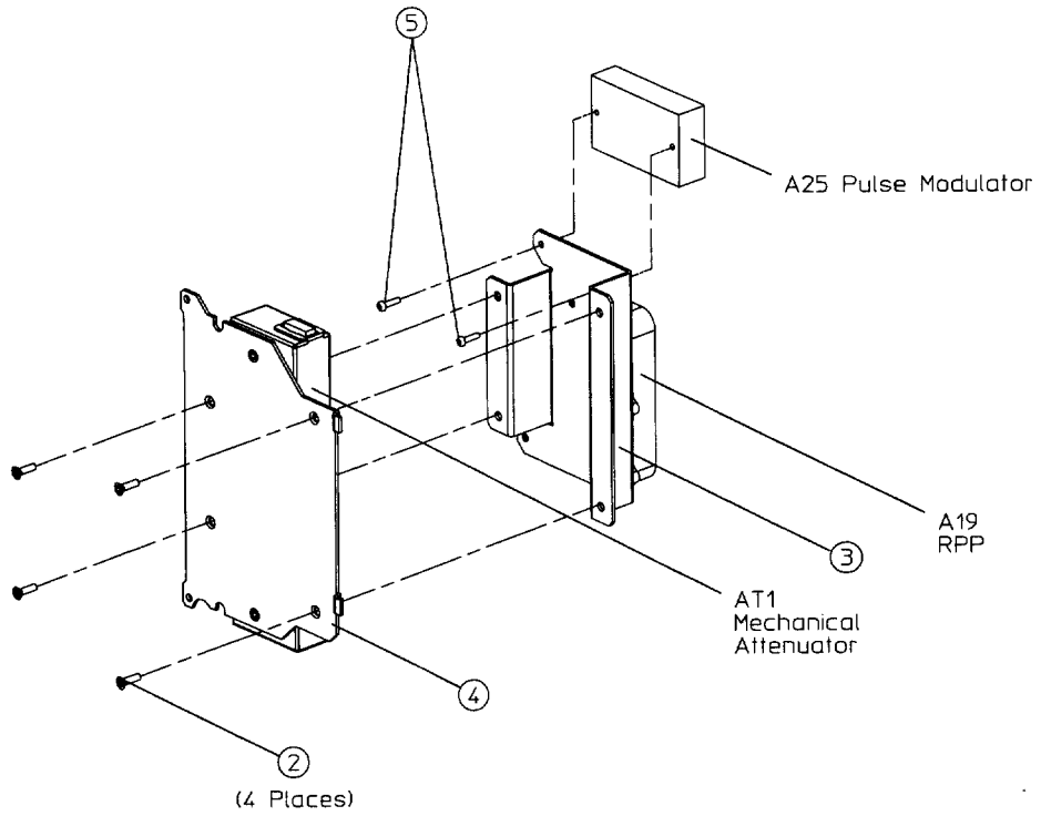
Figure 5-27 A25 Pulse Modulator (with Option UNB) (2 of 2)
