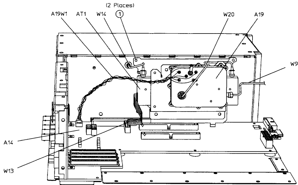
Figure 5-30 AT1 Mechanical Attenuator (2 of 3)
