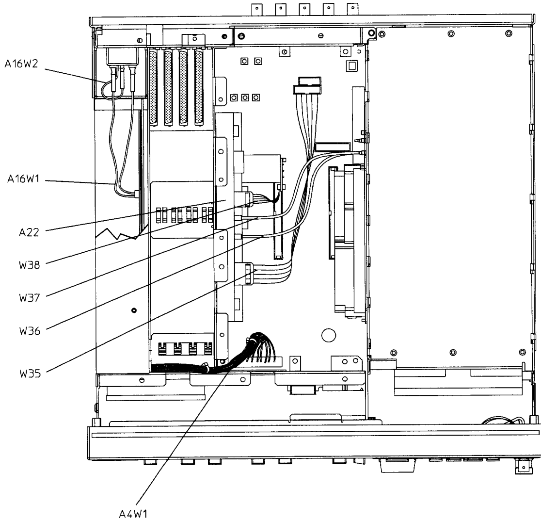
Figure 4-5 Top View
