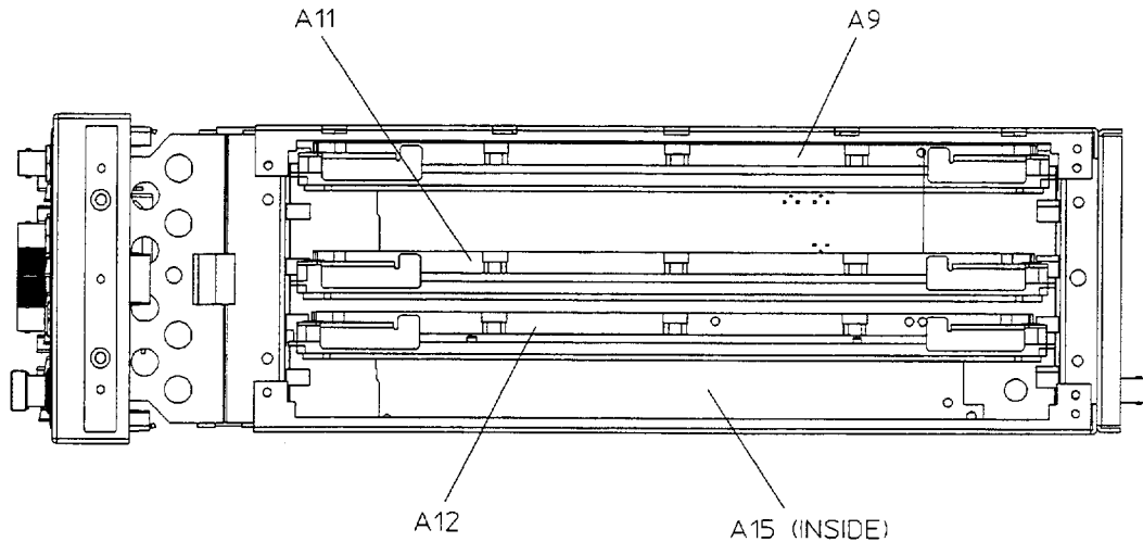
Figure 3-3 Right Side View
