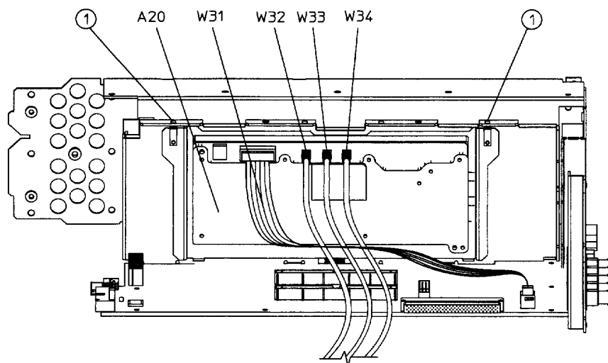
Figure 5-22 A20 Downconverter
