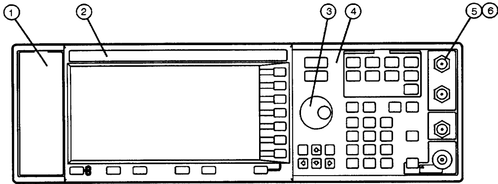
Figure 4-23 Front Panel View (ESG-AP Series)
