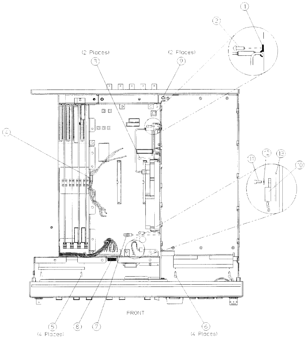
Figure 3-21 Top View
