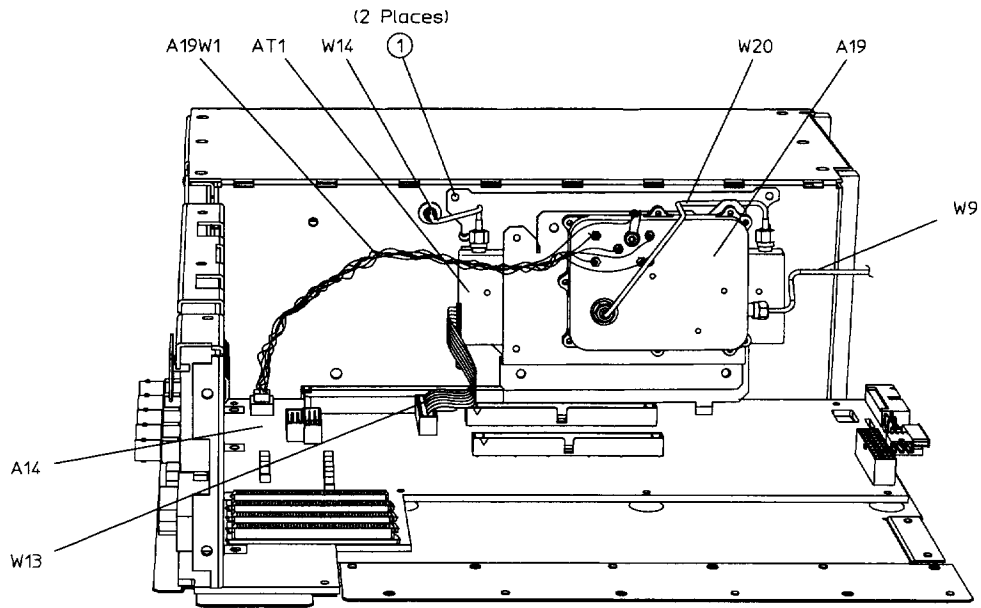
Figure 5-20 A19 Reverse Power Protection (RPP) (2 of 3)
