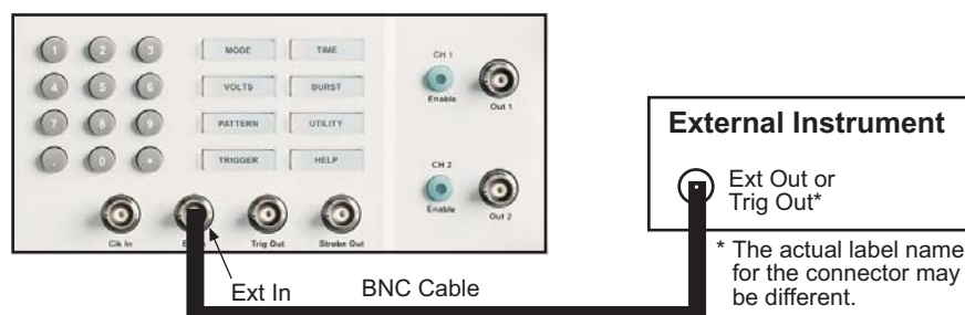
Figure 3-3 Ext In connections
