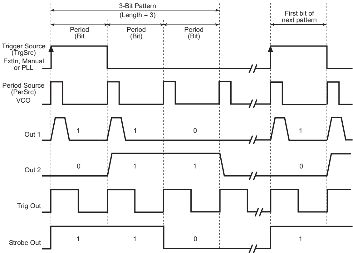
Figure 5-9 Triggered Pattern mode (VCO period source)
