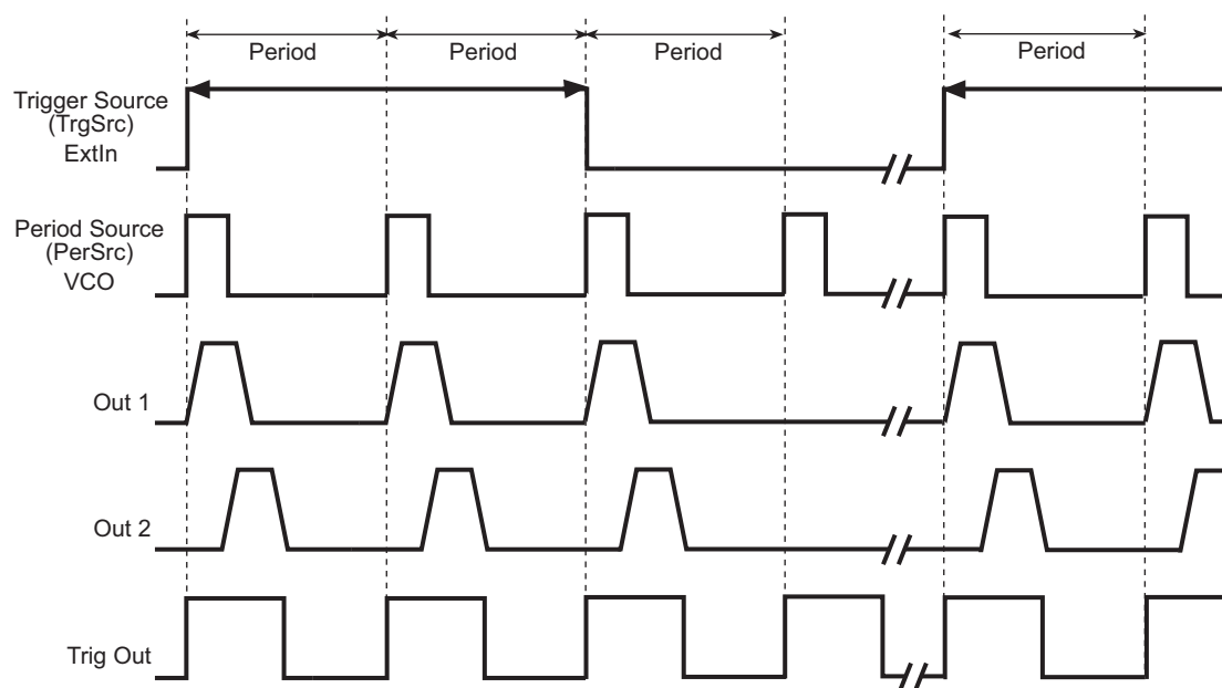
Gated Pulse mode (VCO period source)
