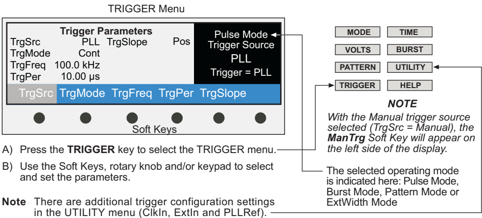
Figure 4-3 Configure triggering
