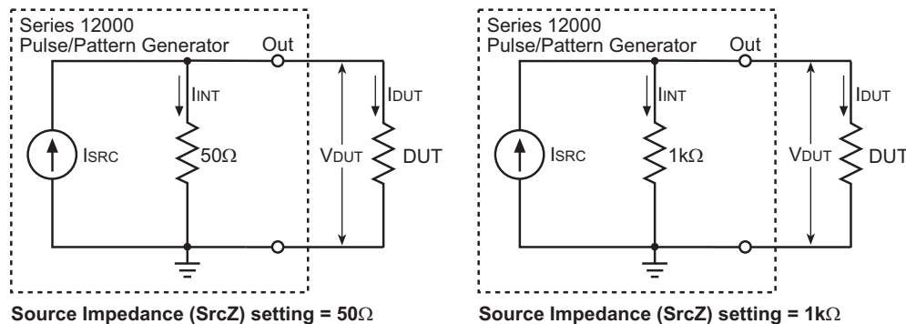
Series 12000 output diagrams
