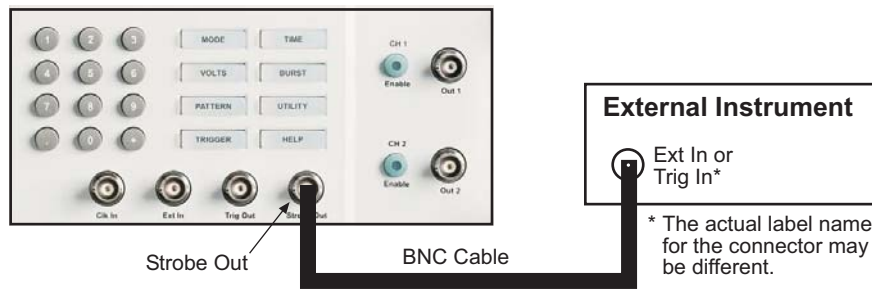
Figure 3-4 Strobe Out connections
