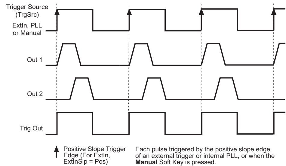
Figure 5-4 Triggered Pulse mode (positive slope)
