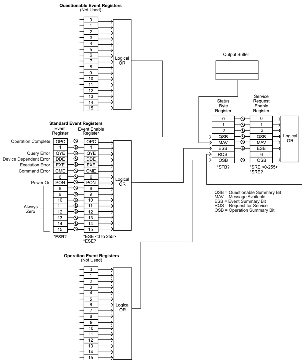
Figure 6-2 Status model
