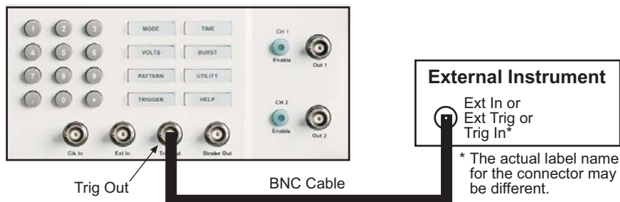
Figure 3-2 Trig Out connections
