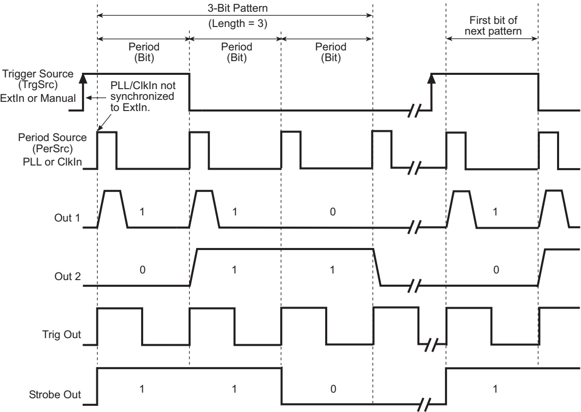
Figure 5-10 Triggered Pattern mode (PLL or ClkIn period source)
