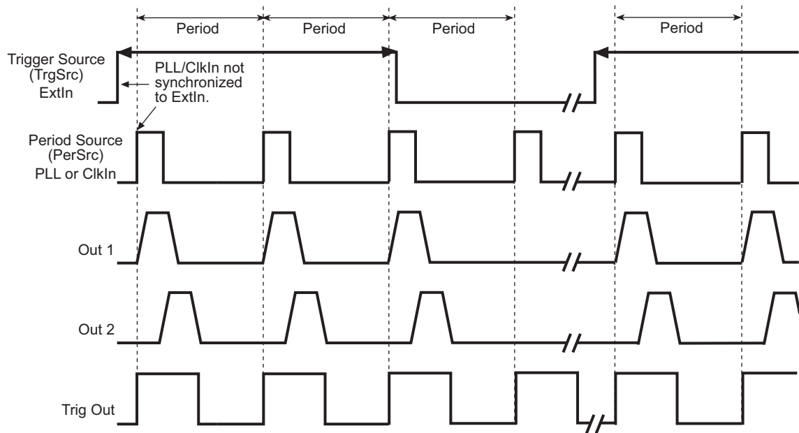
Figure 5-12 Gated Pulse mode (PLL or ClkIn period source)
