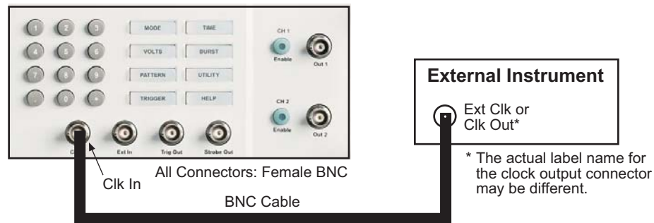
Figure 3-5 Clk In connections
