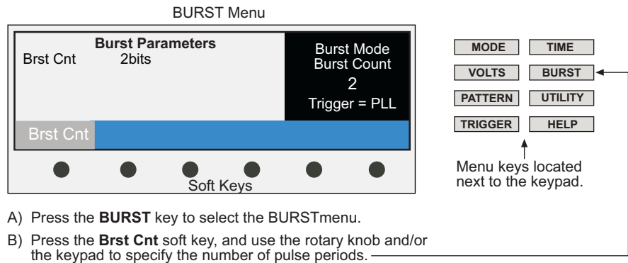
Figure 4-4 Setting Burst mode count
