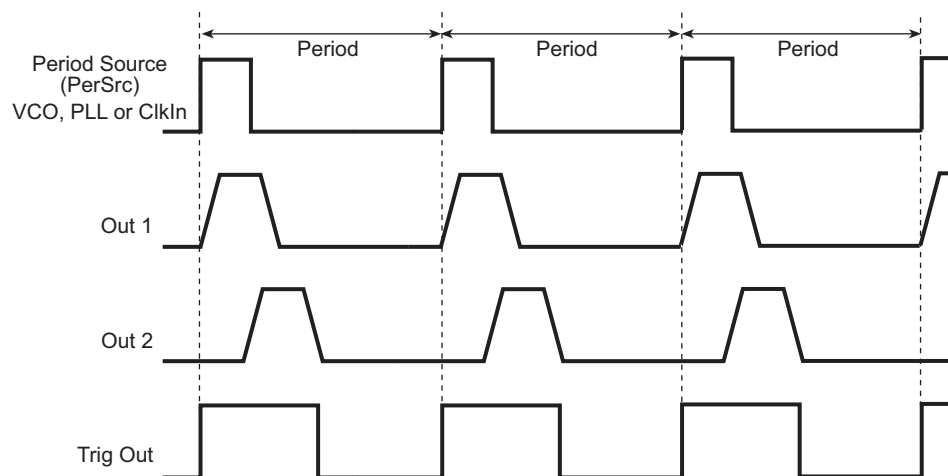
Continuous Pulse mode
