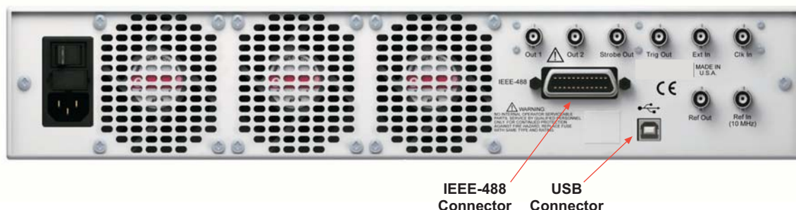
Figure 6-1 IEEE-488 and USB connector locations on rear panel
