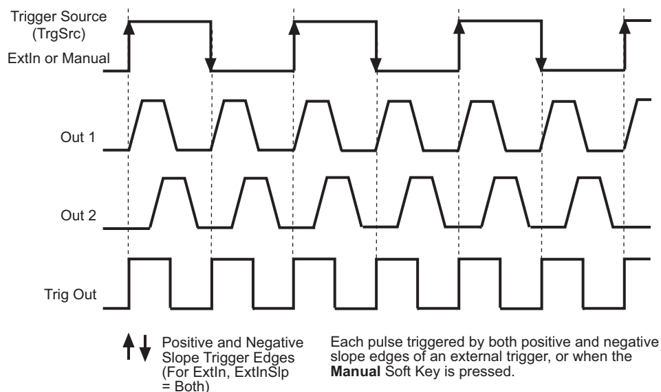
Figure 5-6 Triggered Pulse mode (positive and negative slope)
