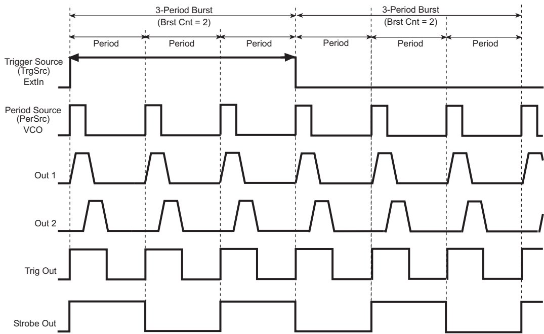
Figure 5-13 Gated Burst mode (VCO period source)
