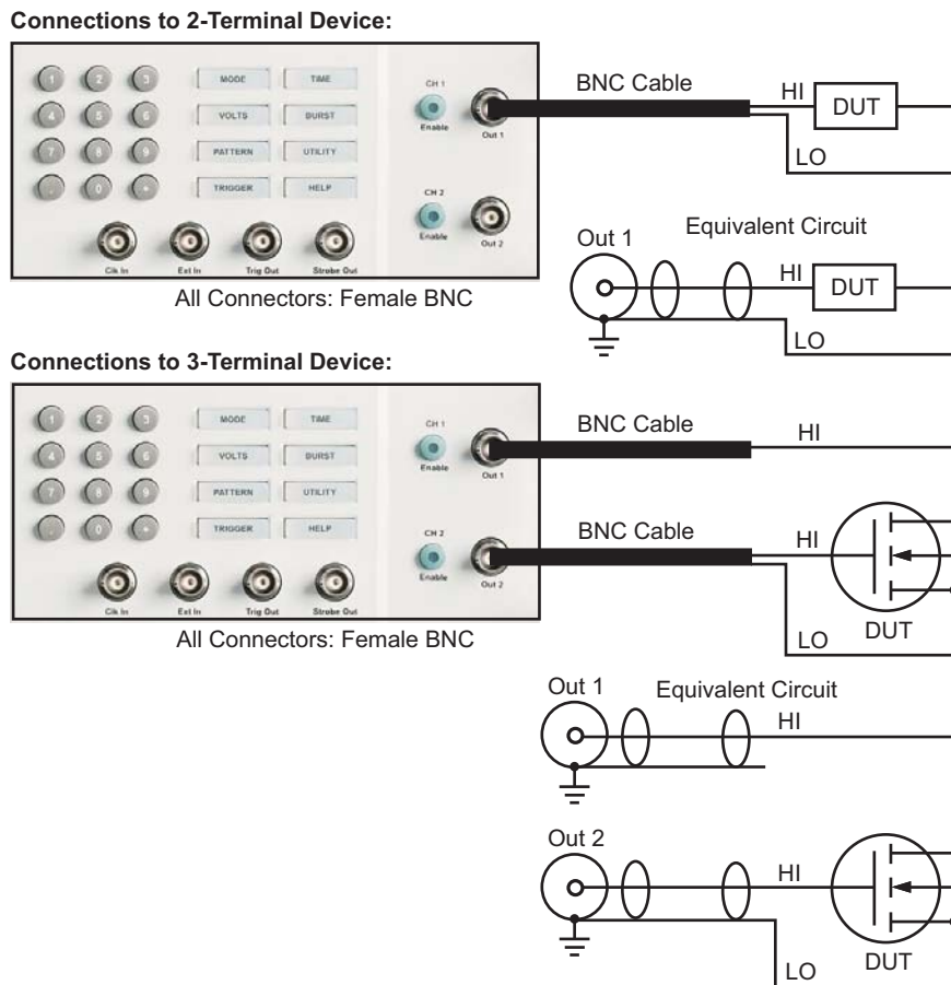
Figure 3-1 Out 1 and Out 2 connections
