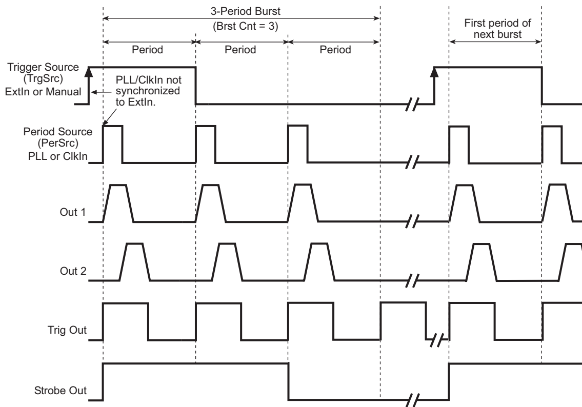
Figure 5-8 Triggered Burst mode (PLL or ClkIn period source)
