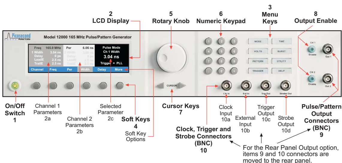
Figure 2-1 Front panel familiarization (Model 12000-2)
