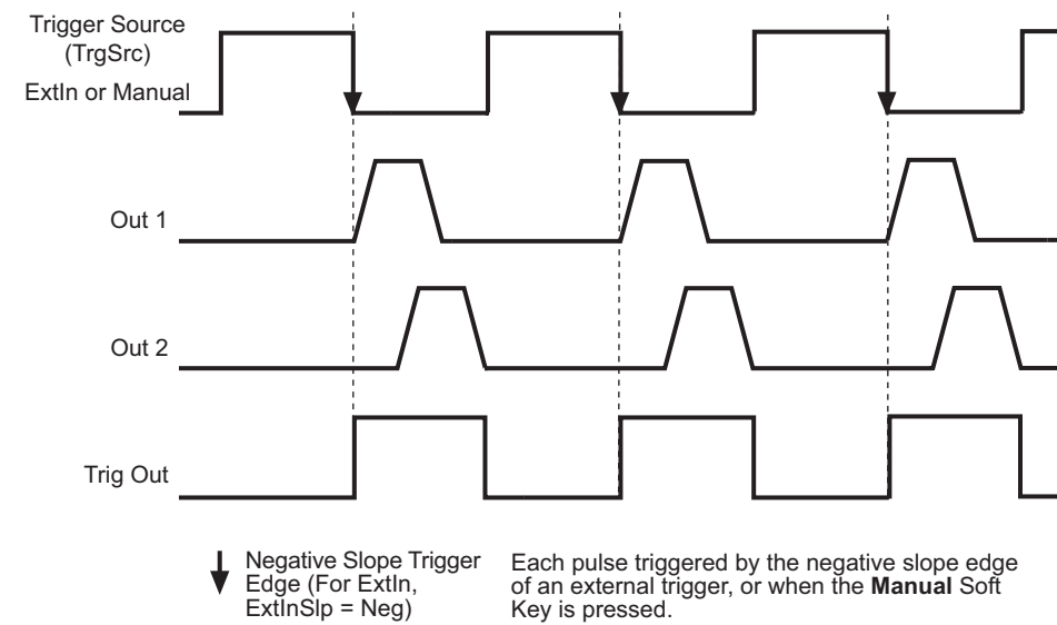
Figure 5-5 Triggered Pulse mode (negative slope)
