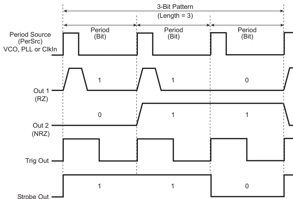
Figure 5-3 Continuous Pattern mode
