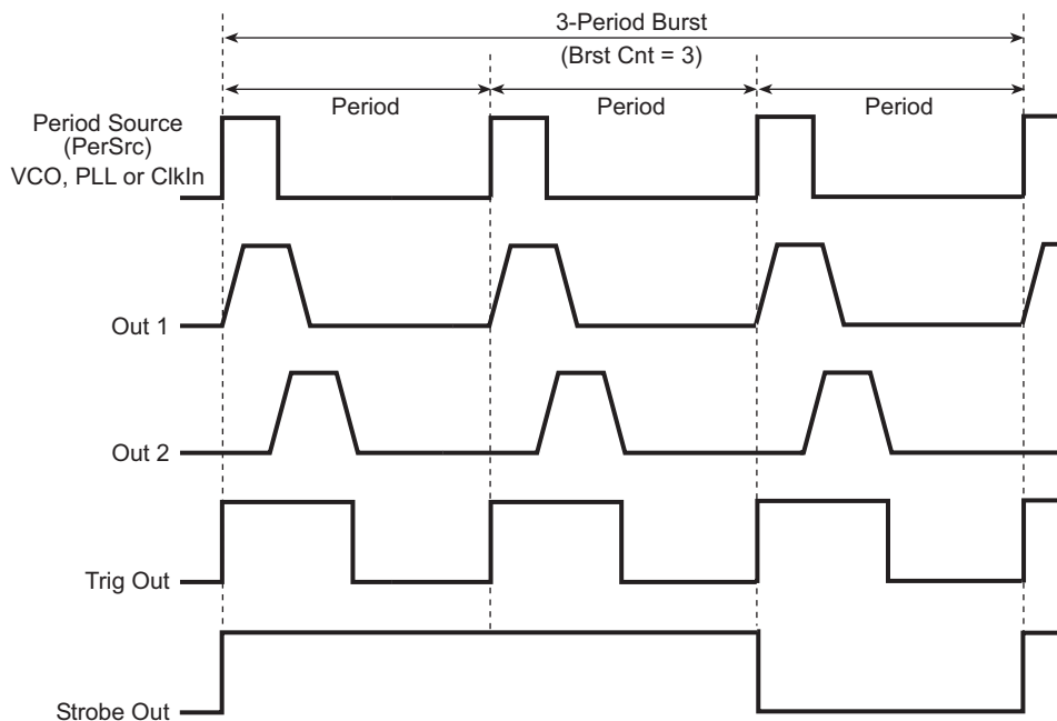
Figure 5-2 Continuous Burst mode
