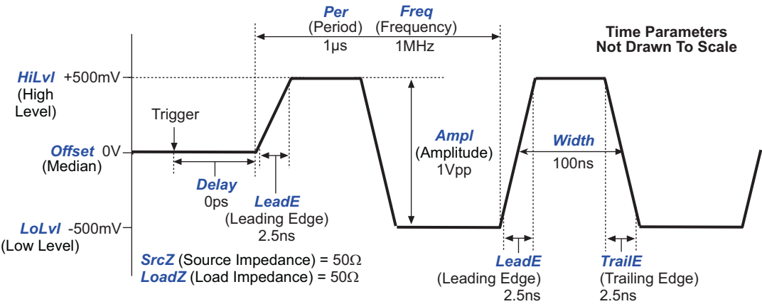
Figure 1-1 Default pulse level and timing parameter settings (Pulse mode, continuous triggering)
