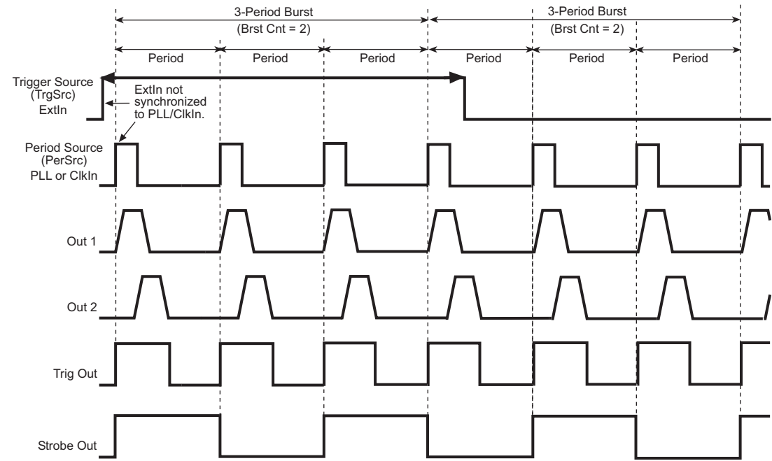
Figure 5-14 Gated Burst mode (PLL or ClkIn period source)
