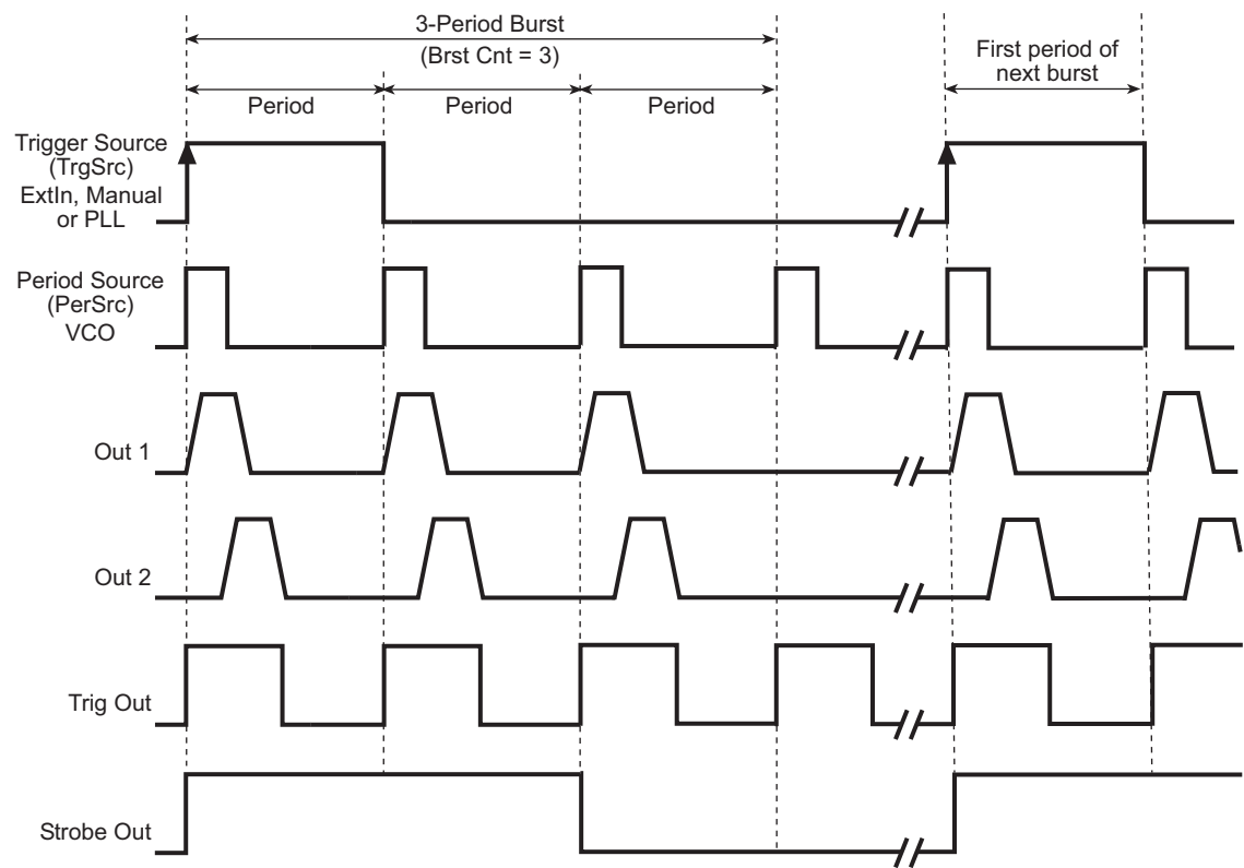
Figure 5-7 Triggered Burst mode (VCO period source)
