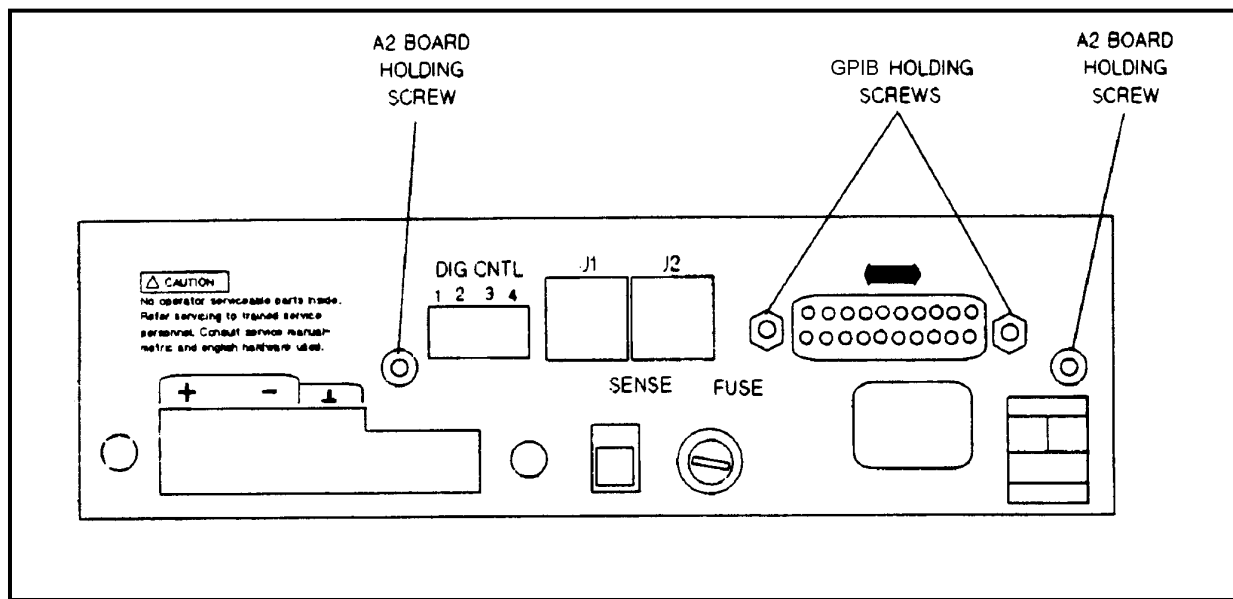
Figure 3-20. GPIB Connector and GPIB Board Holding Screws, Power Supply Rear View
