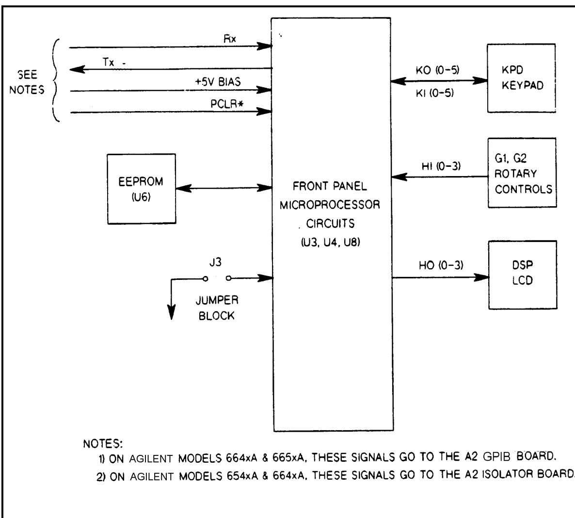
Figure 4-5. Front Panel Board, Simplified Block Diagram
