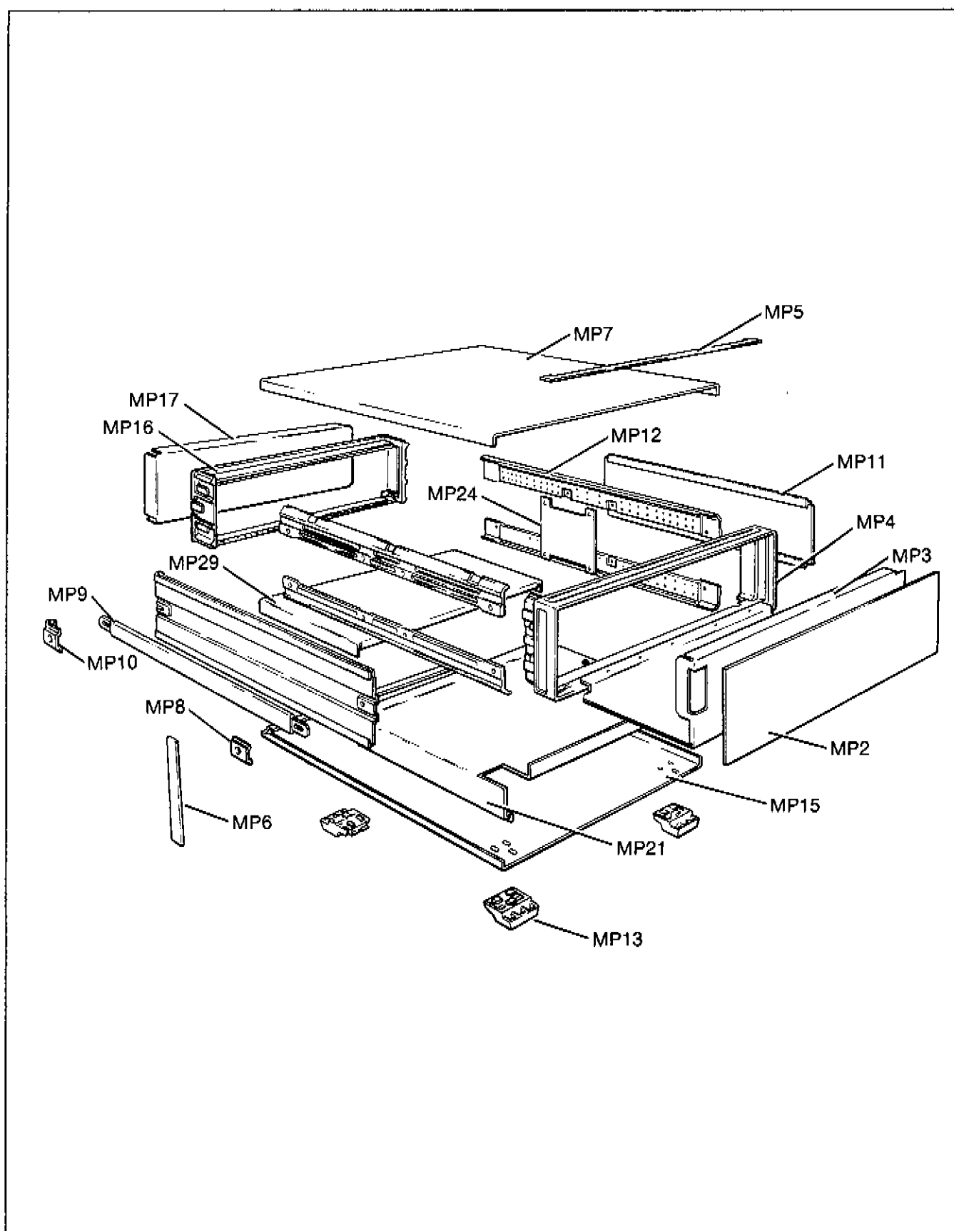
Figure 6. Cabinet Parts
