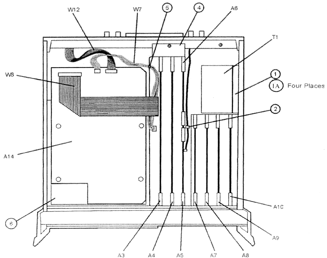
Figure 6-5. Top View
