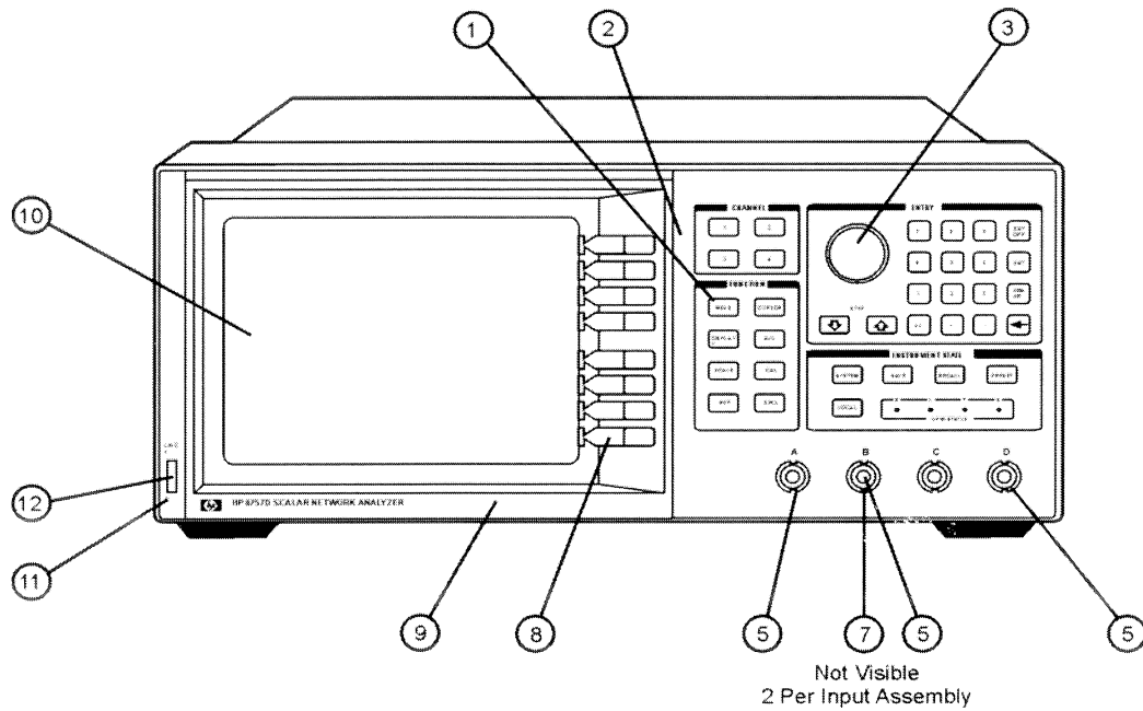
Figure 6-2. Front View
