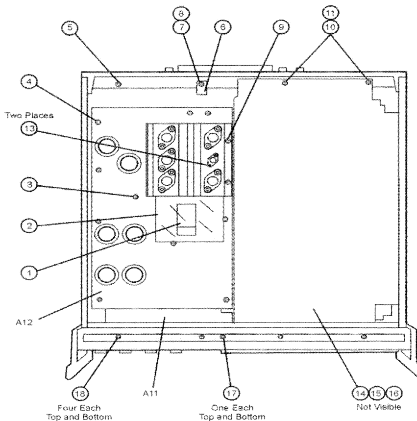
Figure 6-6. Bottom View
