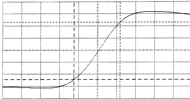
Figure 6-19. Risetime 10-90%
