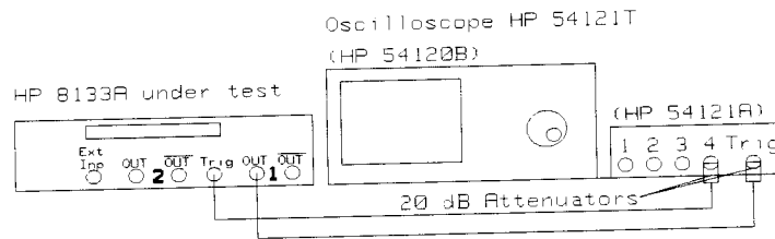
Figure 6-5. TRIGGER Transition Time Test Set-up
