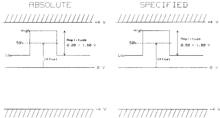
Figure 3-5. TRIGGER Output-level limits into 500
