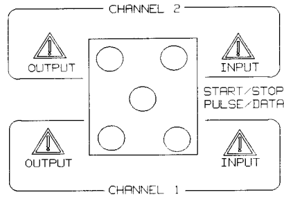
Figure 3-12. Rearpanel signal-connectors
