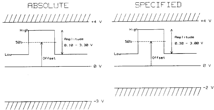
Figure 3-9. PULSE/DATA Output-level limits into 50 Ω
