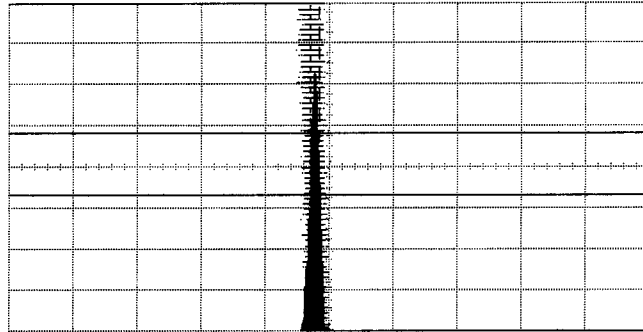
Figure 6-20. Jitter Histogram
